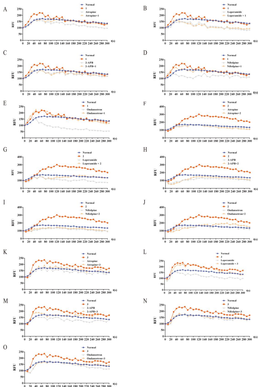
Figure S2: Calcium influx under AM flavonoids-treated with inhibitors. (A-O) Effects of 1 (A-E), 2 (F-J) and 3 (K-O) on isolated calcium influx of HCT116 with different inhibitors.
