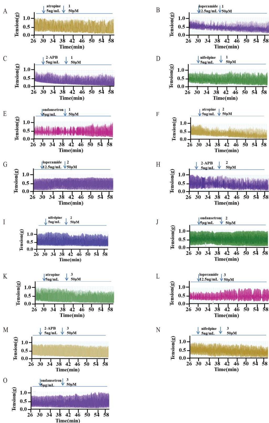
2 Figure S1: Intestinal contraction under AM flavonoids-treated with inhibitors. (A–O) Effects of 1 (A–E), 2 3 (F–J) and 3 (K–O) on spontaneous contractions of isolated intestinal contraction with different inhibitors. 4
