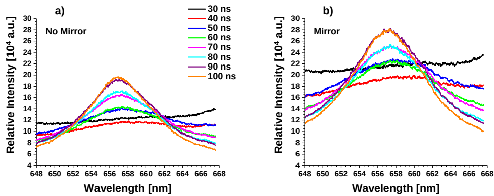
Figure 3. Temporal development of the H_{\alpha} line in the first 100 ns following plasma initiation. (a) Measured spectra and (b) spectra measured with its duplication.
