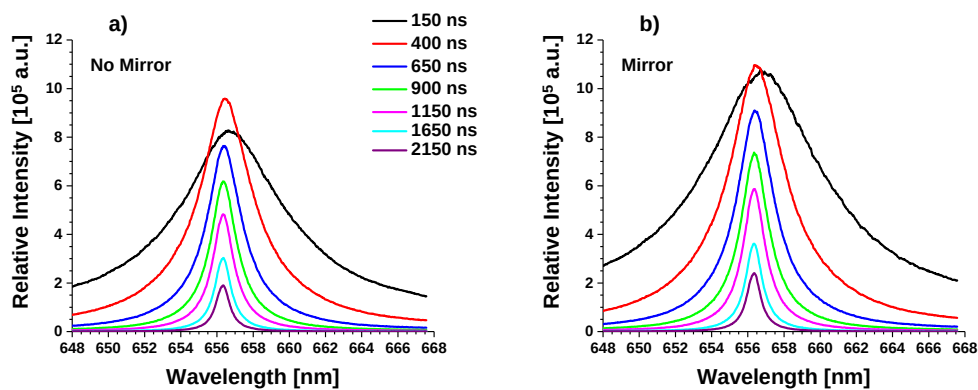
Figure 4. Temporal development of the H_{\alpha} line between 150 ns and 2150 ns following plasma initiation. (a) Measured spectra and (b) spectra measured with its duplication.
