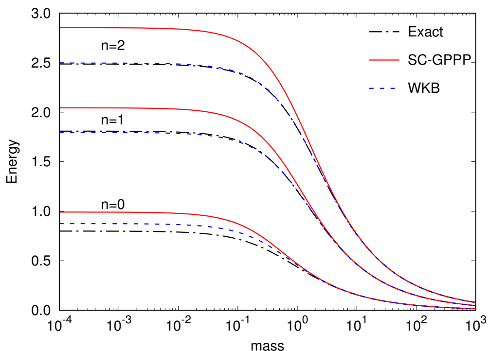
Figure 3. Comparison of three lowest-lying energy levels of the k = 1 , D = 5 MP system, as a function of mass, as computed using the following: exact numerical method (black dash-dotted lines); SC-GPPP method (red solid lines); WKB method (blue dashed lines). Units where \hbar = c = 1 were assumed.
