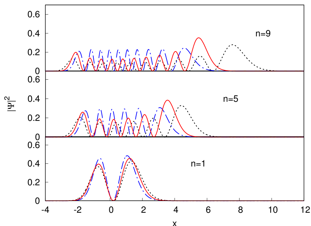
Figure 5. Comparison of wavefunction probability densities for several different k = m = 1 , D = 5 MP system eigenstates, as computed using the following: exact numerical method (blue dash-dotted lines); SC-GPPP method of Equation (34) (red solid lines); non-relativistic limit (black dotted lines) (color figure online).
