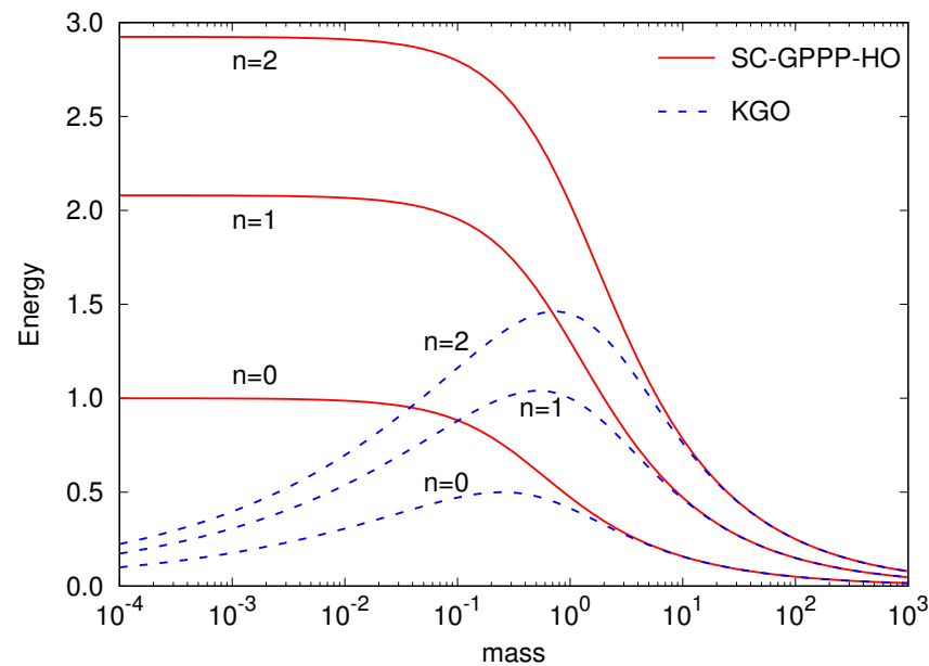
Figure 6. Comparison of three lowest-lying energy levels of the k = 1 HO system, as a function of mass, as computed using the SC-GPPP method and the values obtained from Equation (65) for the Klein–Gordon oscillator. Units where \hbar = c = 1 were assumed.
