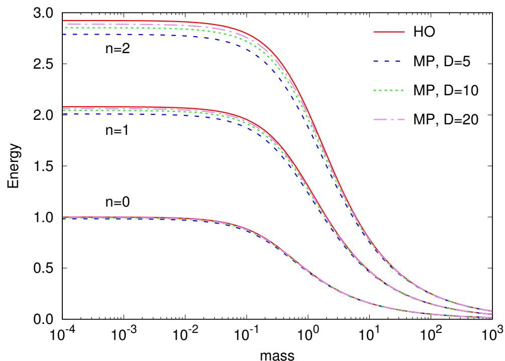
Figure 1. Three lowest-lying energy levels as a function of mass, for k = 1 MP, with three different well depths. The corresponding energy values for k = 1 HO [14] are included for comparison. All the values were obtained with the SC-GPPP method. Units where \hbar = c = 1 were assumed.
