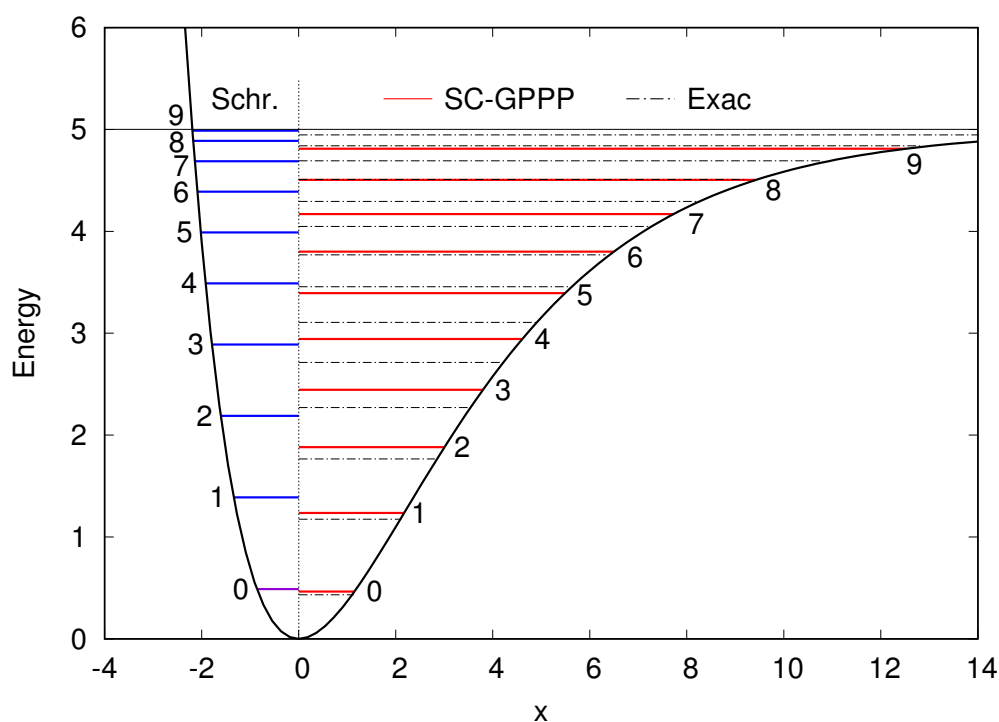
Figure 4. Schematic representation of the allowed energy levels of the k = m = 1 , D = 5 MP systems, as obtained from the Schrödinger solution (Schr.), the SC-GPPP (red solid lines), and exact numerical (black dash-dotted lines) methods. Units where \hbar = c = 1 were assumed.
