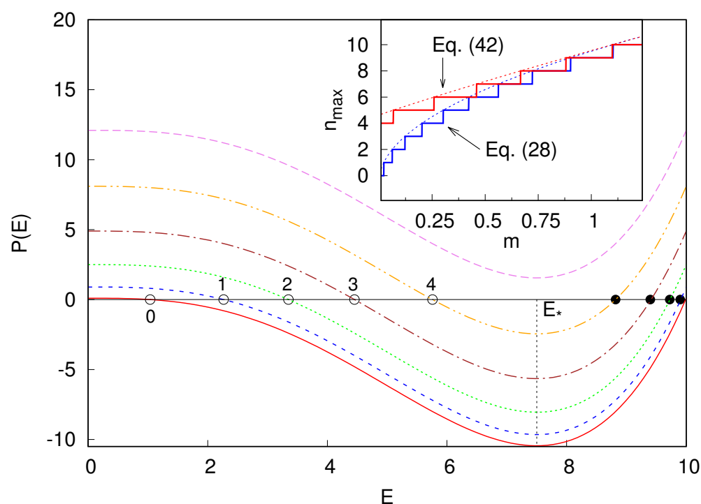
Figure 2. First six ( n = 0, \dots, 5 ) profiles of the polynomial of Equation (40) as a function of E , in the interval 0 \leq E \leq 2D , for k = 1 , m = 0.0001 , and D = 5 . The empty dots correspond to the roots of P(E) or the solutions E_{H,n} of Equation (39). The inset shows the profiles of Equations (28) and (42), in the interval of 0 \leq m \leq D/4 , for an MP with k = 1 and D = 5 . Units where \hbar = c = 1 were assumed.
