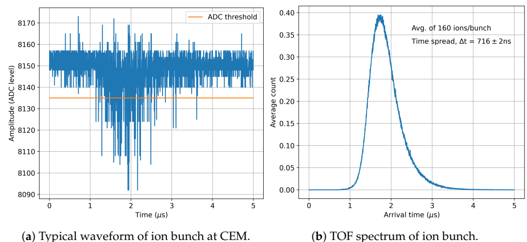
Figure 10. Bunched ion spectrum and waveform from run using bunched cesium ions. (a) Typical waveform of one ion bunch recorded using a CAEN DT5730. (b) Histogram of samples above the signal noise threshold, accumulated and averaged over 10,000 waveforms.
