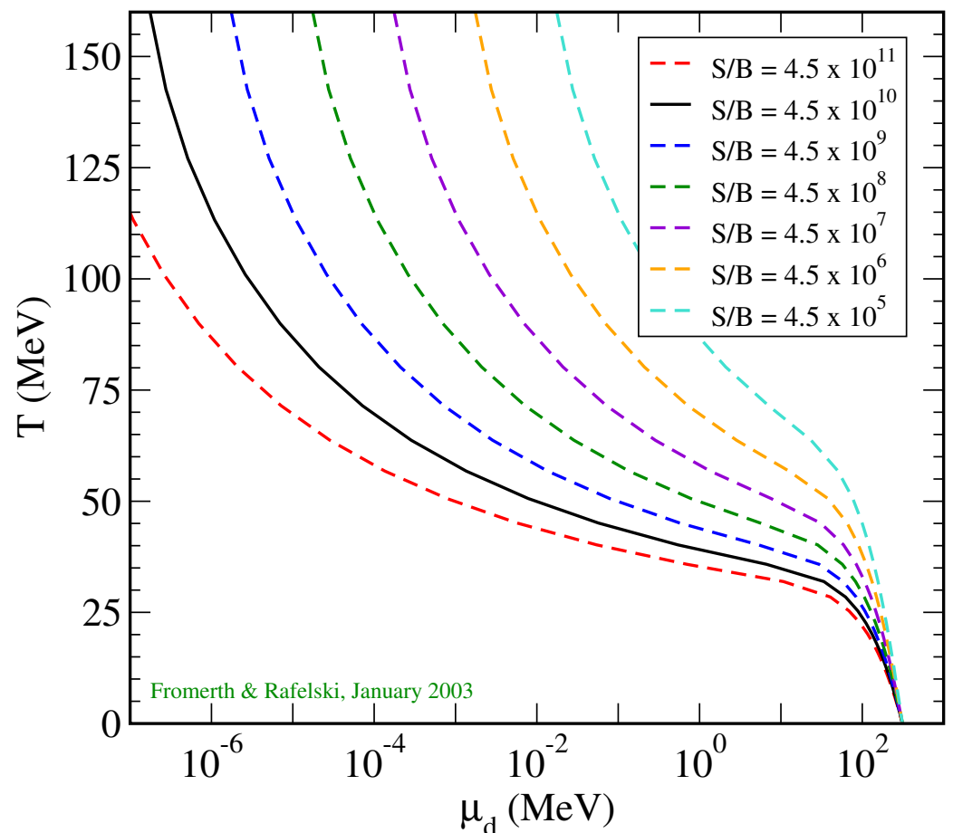
Figure 7. Plot of the down quark chemical potential \mu_d as a function of temperature for differing values of entropy-per-baryon S/B ratios (2003 unpublished, Fromerth & Rafelski [62]).
