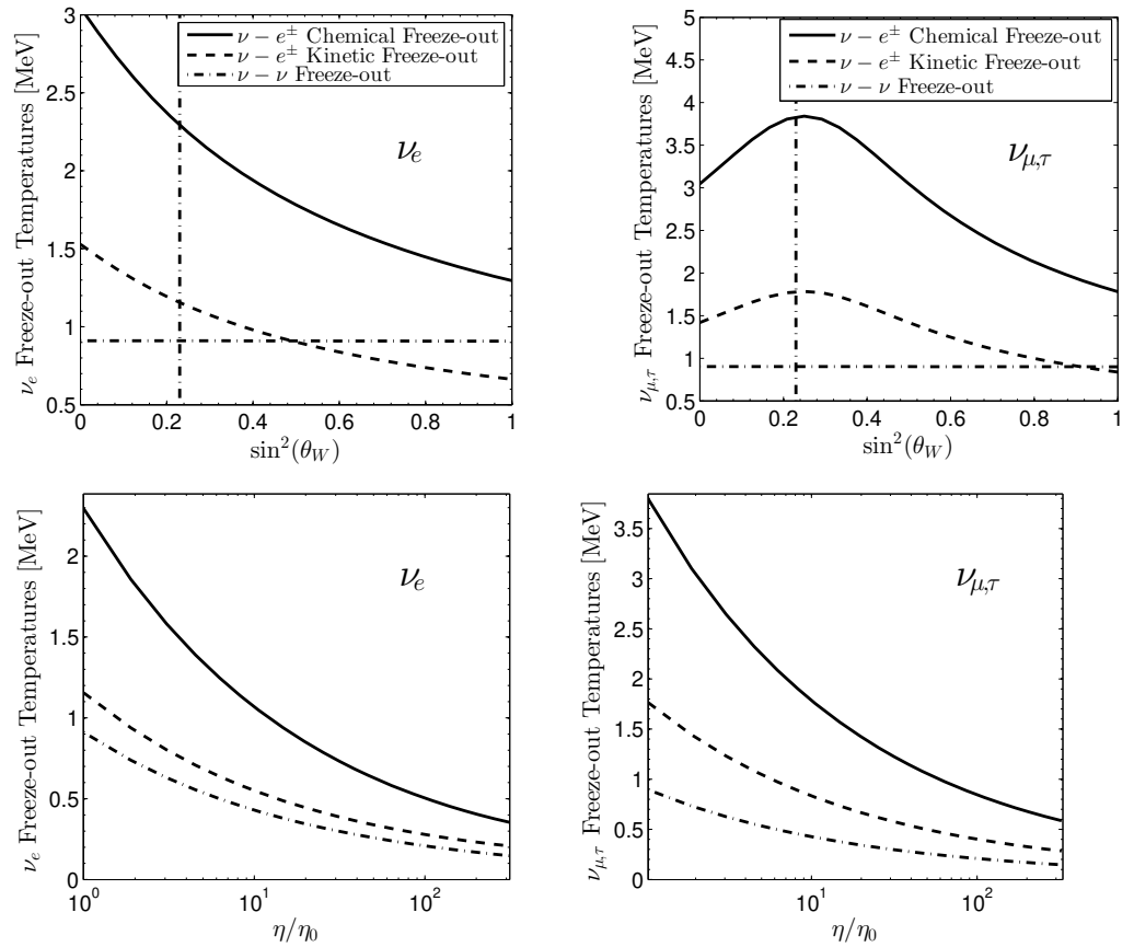
Figure 18. Freeze-out temperatures for electron neutrinos ( left ) and \mu , \tau neutrinos ( right ) for the three types of freeze-out processes adapted from paper [109]. Top panels print temperature curves as a function of \sin^2 \theta_W for \eta = \eta_0 , the vertical dashed line is \sin^2 \theta_W = 0.23 ; bottom panels are printed as a function of relative change in interaction strength \eta/\eta_0 obtained for \sin^2 \theta_W = 0.23 .
