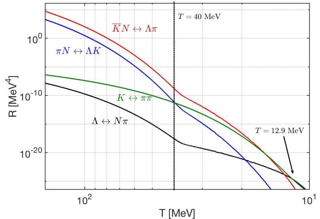
Figure 15. Thermal reaction rate R per volume and time for important hadronic strangeness production, exchange and decay processes as a function of temperature 150 \text{ MeV} > T > 10 \text{ MeV} . The following processes are presented: \Lambda \leftrightarrow N\pi (solid black line), K \leftrightarrow \pi\pi (solid green line), \pi N \leftrightarrow \Lambda K (solid blue line), \bar{K}N \leftrightarrow \Lambda\pi (solid red line). Two temperature crossings are denoted at T = 40 \text{ MeV} , 12.9 \text{ MeV} .
