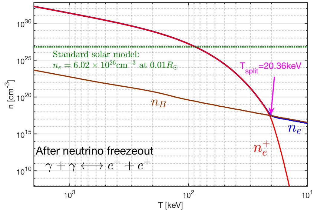
Figure 19. The e^\pm number densities as a function of temperature in the range 2\text{ MeV} > T > 10\text{ keV} . The blue solid line is the electron density n_{e^-} , the red solid line is the positron density n_{e^+} , and the brown solid line is the baryon density n_B . For comparison, we also show the green dotted line as the solar electron density within the solar core [127].
