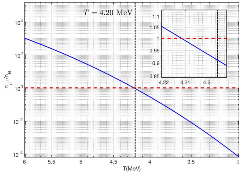
Figure 17. The density ratio between \mu^\pm and baryons n_{\mu^\pm}/n_B (blue solid line) is plotted as a function of temperature. The red dashed line indicates a density ratio value of n_{\mu^\pm}/n_B = 1 . The density ratio at the muon disappearance temperature (vertical black dashed line) is about n_{\mu^\pm}/n_B(T_{\text{dis}}) \approx 0.911 .
