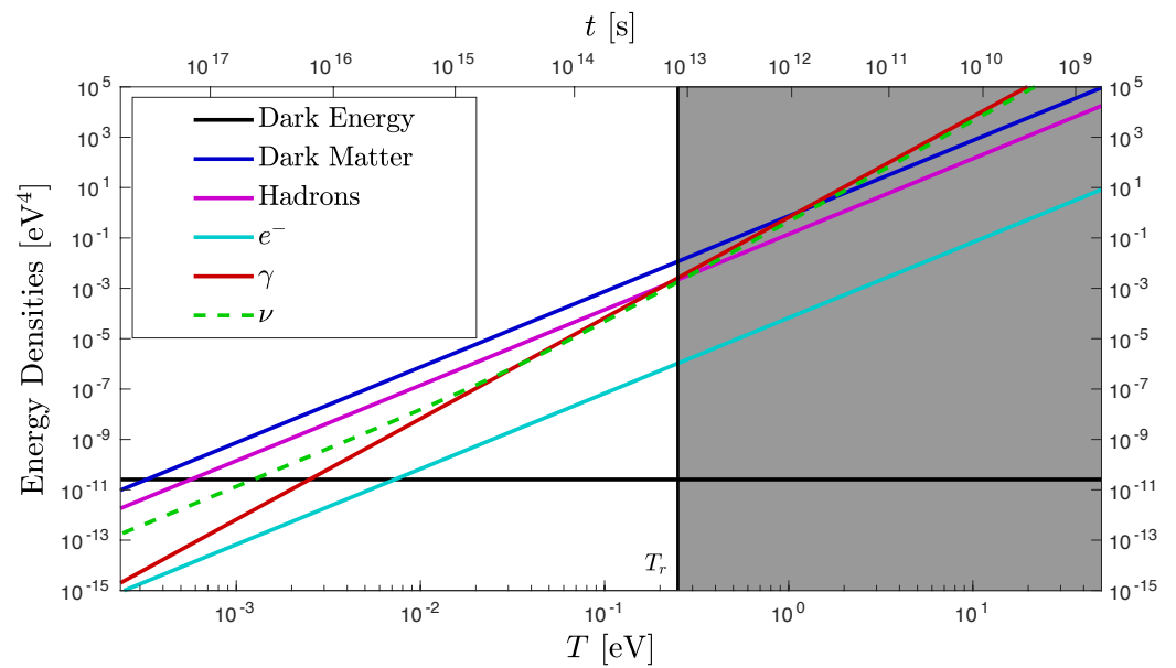
Figure 1. Contemporary and recent Universe composition: In this example we assumed present day composition to be 69% dark energy, 26% dark matter, 5% baryons, <1% photons and neutrinos. The dashed line shows how introduction of 2 \times 0.1 eV mass in two of the three neutrinos impacts the energy density evolution (Neutrino mass choice is just for illustration. Other values are possible). The recombination temperature T_r \approx 0.25 eV delimits the era when the Universe was opaque shown as the shaded region.
