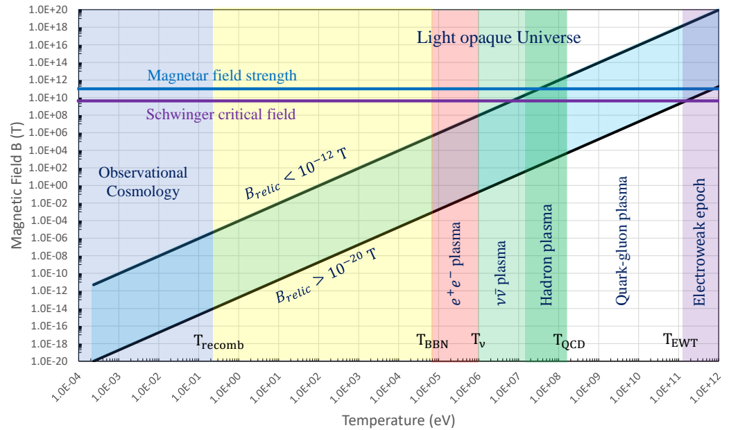
Figure 21. Qualitative value of the primordial magnetic field over the evolutionary lifespan of the Universe. The upper and lower black lines represent extrapolation of the EGMF bounds into the past. The major phases of the Universe are indicated with shaded regions. The values of the Schwinger critical field (purple line) and the upper bound of surface magnetar field strength (blue line) are included for scale.
