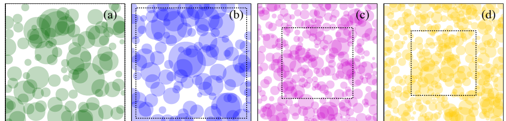
Figure 7. Samples of generated systems in the picture of the CGC after the thermalization for (a) AuAu collisions at \sqrt{s} = 130 GeV, (b) AuAu collisions at \sqrt{s} = 200 GeV, (c) PbPb collisions at \sqrt{s} = 2760 GeV, and (d) PbPb collisions at \sqrt{s} = 5020 GeV. These systems correspond to a square box of around 1\text{fm}^2 . The inner dashed square is the size of the simulated system for the purposes of the computation of the radial distribution function.
