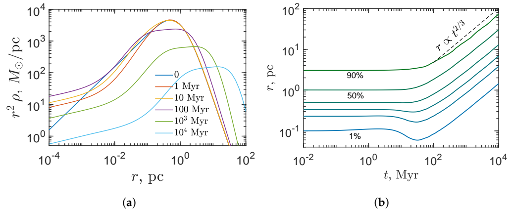
Figure 4. The evolution of the mass distribution is shown. (a) The density profile at different times. (b) The evolution of the mass shells containing 1, 5, 10, 20, 50, and 90 percent of the cluster mass, respectively.
