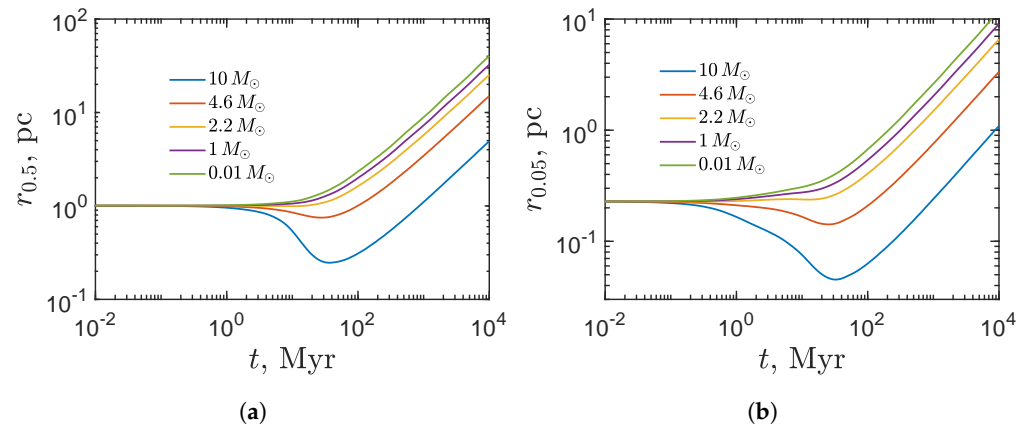
Figure 5. The evolution of mass shells containing 50 (a) and 5 (b) percent of the mass for different types of PBHs is shown.
