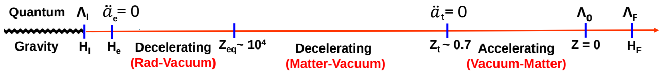
Figure 1. From de Sitter to de Sitter (out of visible scale). Just after the unknown quantum gravity regime, all the energy of the universe is concentrated on the emergent and unstable de Sitter spacetime ( \Lambda_I = 3H_I^2, \rho_{\Lambda_I} = 3M_P^2 H_I^2, \rho_M \equiv 0 ). The classical evolution shown above is analytically described by the decaying \Lambda(H) model, as given by Equation (13), which is the unique fuel of both inflationary stages. Since \Lambda(H) is a continuous function, the equilibrium redshift z_{eq} is determined in the usual way (sudden transition), with a small contribution by the \nu parameter, as discussed in Equation (32). For all allowed values of \nu , the ultimate destiny of the model is the pure de Sitter vacuum state fixed by \Lambda_F = 3H_F^2 . However, it is attained only in the distant future ( a \rightarrow \infty ), as shown in Equation (26). For \nu = 0 , the late time evolution after \ddot{a}(H_e) = 0 is just the rigid vacuum \Lambda CDM model.
