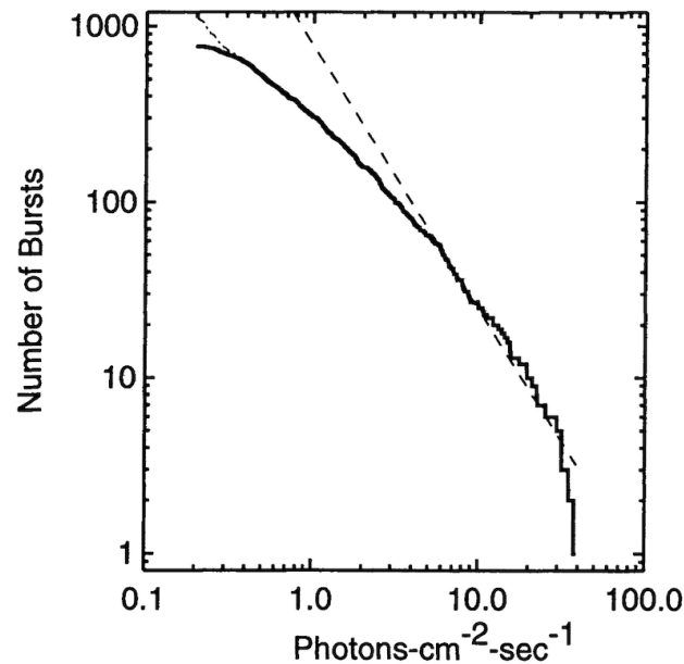
Figure 6. Integral log N -log P distribution of 772 GRB detected with BATSE in the range 50–300 keV band. The peak flux P is integrated over 1.024 s. The dot-dashed line gives the correction for instrumental trigger efficiency, while the dashed line gives the power-law slope ( -3/2 ) expected in the case of an homogeneous distribution of GRBs in space. Reprinted from [14].
