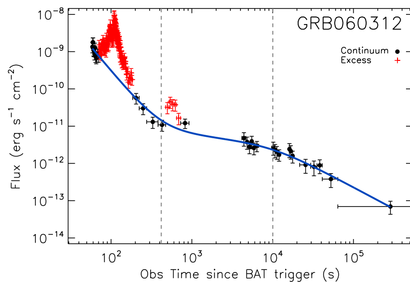
Figure 25. Example of light curve of the intrinsic 0.6–30 keV afterglow starting from T \geq 60 s as detected with Swift . Two X-ray flares above the smoothed light curve are apparent. Reprinted from [121].
