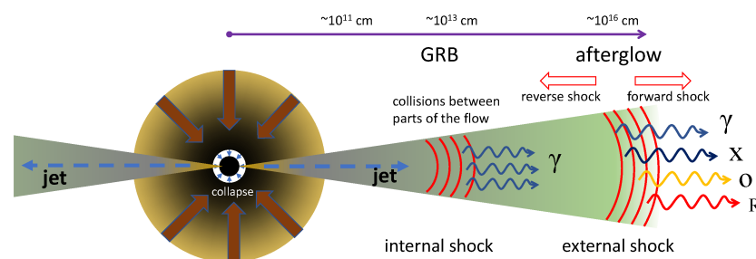
Figure 16. Sketch of a relativistically expanding fireball. The kinetic energy of the jet is converted through shocks (internal, external) in electromagnetic energy. Figure reprinted from [63].
