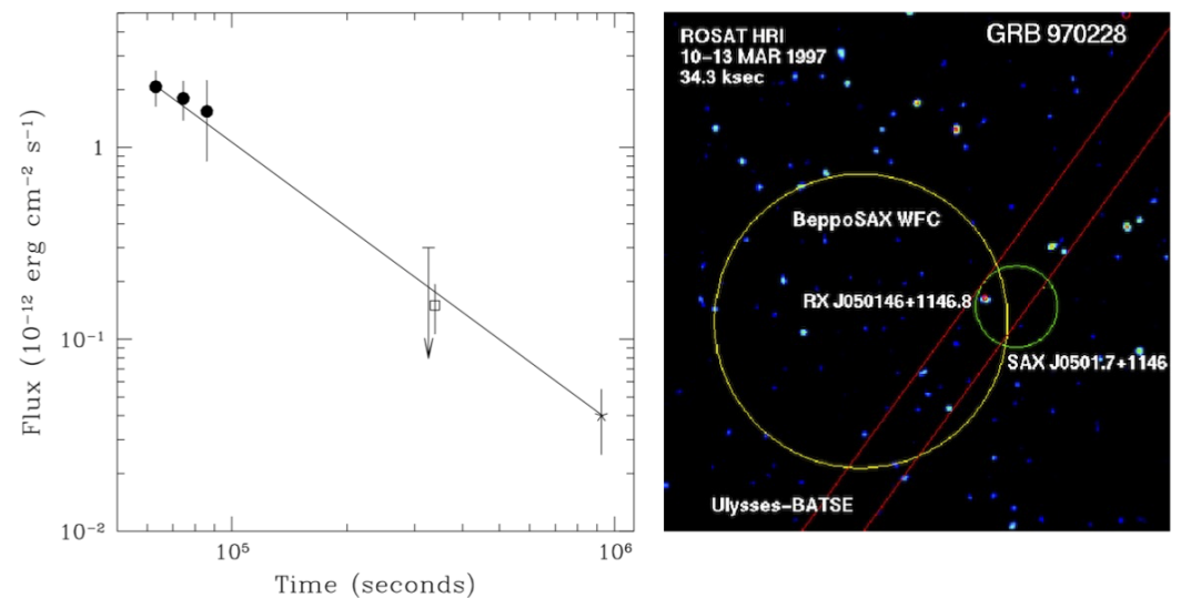
Figure 12. (Left): Decline in the GRB 970228 flux in 0.1–2.4 keV with time, starting from the follow-up time of GRB 970228 with BeppoSAX , uncorrected for galactic absorption. The filled dots are the LECS data points, the arrow is the LECS 3\sigma upper limit, the square gives the flux extrapolated from the MECS detection, and the asterisk shows the ROSAT HRI data point. The best fit power-law decay (continuous line) is also shown. (Right): Image of the ROSAT HRI FOV (8 arcmin wide) found during the GRB 970228 follow-up performed on 1997 March 10. Only one source (RXJ050146 + 1146.8) was found inside the error box (small circle with \sim 50 arcsec radius) of the fading source SAX J0501.7 + 1146. In addition, this ROSAT source was coincident with the optical source (in red) within 2 arcsec. The large circle shows the 3 arcmin error circle of GRB 970228 as determined with the BeppoSAX WFC, while the two straight lines give the uncertainty strip derived from the BeppoSAX GRBM and Ulysses –BATSE. Reprinted from Frontera et al. [37].
