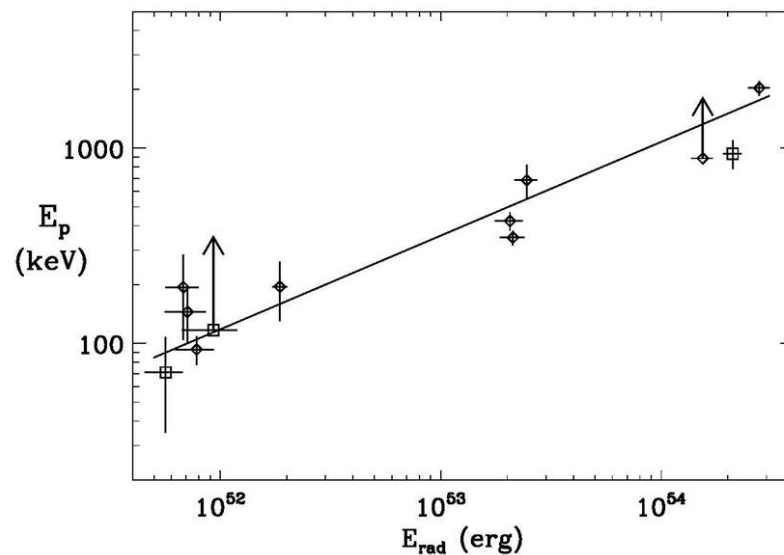
Figure 19. The E_p – E_{iso} relation discovered with BeppoSAX . Reprinted from [81].
