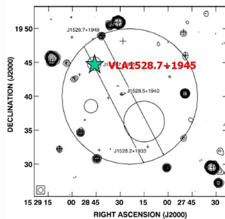
Figure 9. (Top panel): Light curve of GRB 970111. Reprinted from [32]. (Bottom panel): The largest circle gives the earliest WFC error box, while the smaller circle gives the latest WFC error box. The strip crossing the largest circle is the error box derived with the Interplanetary Network (IPN). As can be seen, in the intersection of the refined WFC error box with the IPN annulus, no source was observed. Adapted from the figure of [33].
