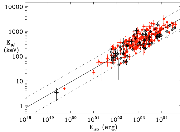
Figure 20. The E_{p,i} – E_{iso} correlation for a recent sample of 224 long GRBs. Those events detected and localized by the Swift satellite are shown in red color, while those in black color were detected with other satellites ( BeppoSAX , INTEGRAL , Fermi , etc). Courtesy of Lorenzo Amati.
