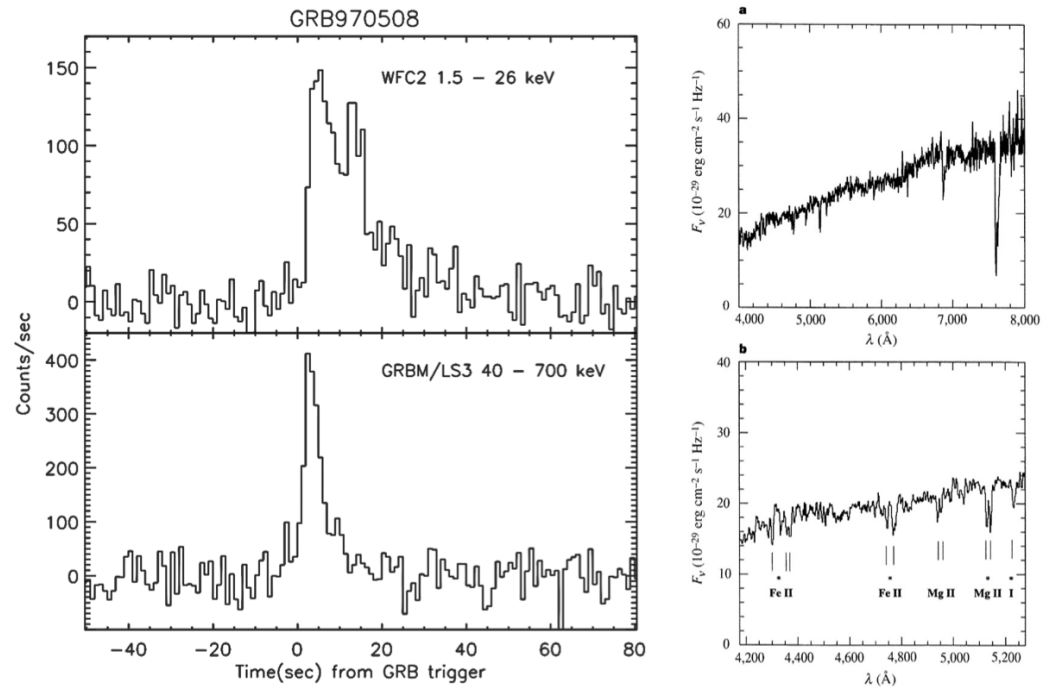
Figure 14. (Left top): Light curve detected by WFCs (1.5–26 keV). (Left bottom): Light curve detected by GRBM (40–700 keV). Reprinted from [44]. (Right): Spectrum of the optical counterpart of GRB 970508 taken with the Keck Low Resolution Imaging Spectrograph [46]. (a) Full spectrum; (b) expansion of a limited region of the spectrum, with strong absorption lines. Various absorption lines were discovered: those marked with an asterisk correspond to a system at redshift z = 0.835 , while the others at redshift of z = 0.767 . The largest z values were found, weeks later, in the emission lines from the host galaxy associated with the fading object.
