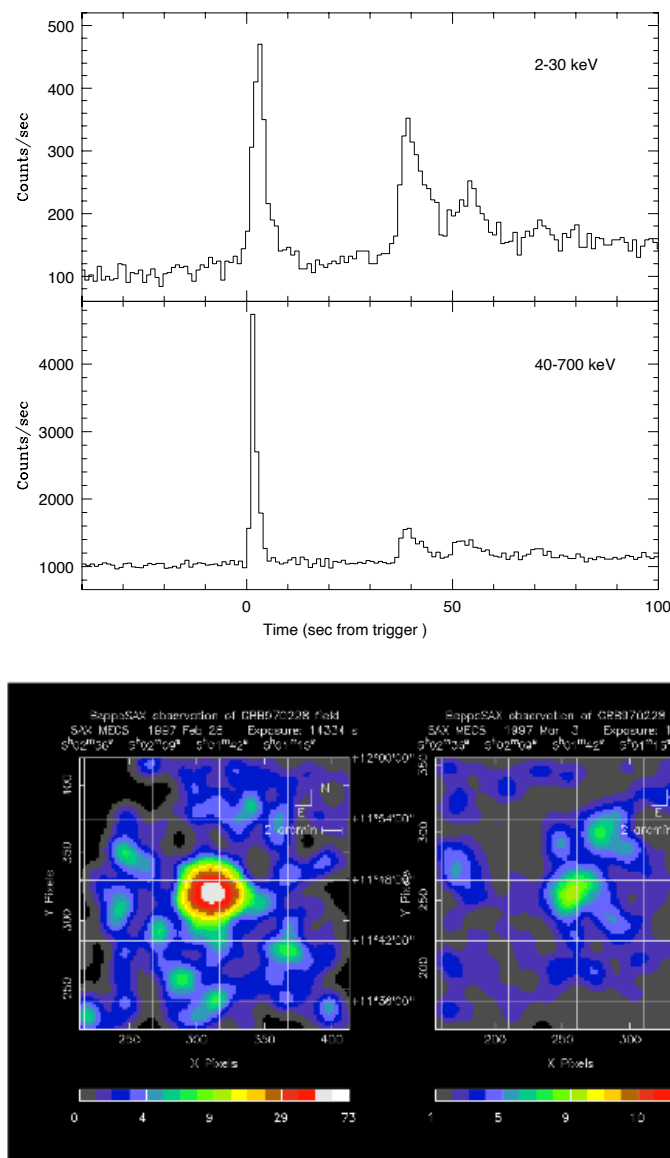
Figure 10. (Top panel): Light curve of GRB 970228 as detected with WFC and GRBM. (Bottom panel): X-ray images of GRB 970228 as detected with MECS telescopes at two different times. The image on the left is that obtained 8 to 16 h after the burst. The image on the right is that obtained in the observation 3.5 days after the burst. From the first to the second X-ray observation, the source had faded by a factor 20. Reprinted from [34].
