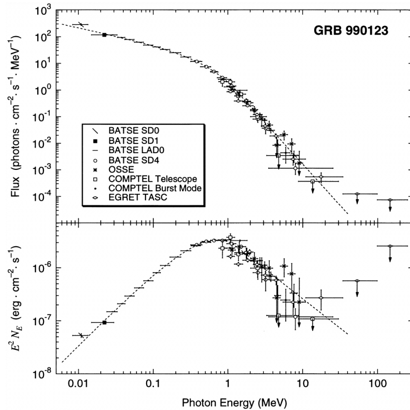
Figure 5. An example of GRB photon spectrum and the corresponding E^2 N(E) function. It shows the BATSE spectrum of the GRB occurred on 1999 January 23 (GRB 990123), that was also detected and promptly accurately localized with BeppoSAX . Reprinted from [13] © AAS. Reproduced with permission.
