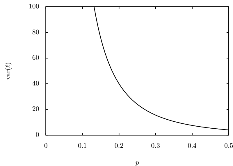
Figure 2. The variance (69) in the number of steps \ell as a function of p .
