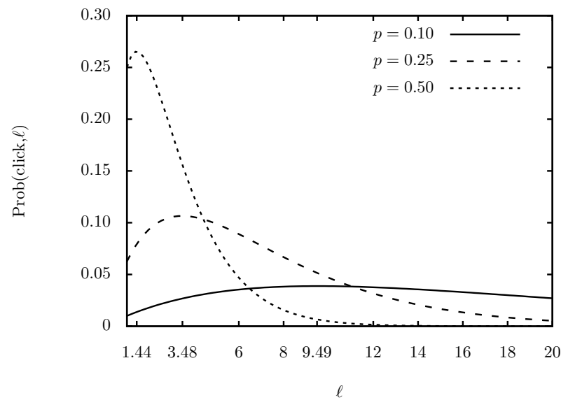
Figure 1. The probability (66) of a single click during \ell steps of the clock's evolution. The values of p are 0.1, 0.25, and 0.5.
