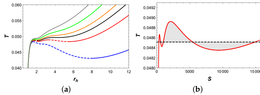
Figure 2. (a) T vs. r_h . The blue, red, black, orange, green and gray curves correspond to P = 0.0024 , 0.00337487 , 0.00374402 , 0.004 , 0.0044492 and 0.005 , respectively. Solid curves indicate stable branches, while dashed curves represent unstable branches. (b) T-S diagram of two pairs of equal area regions at pressure P = P_t = 0.00337487 . The horizontal line has a temperature T = T_t = 0.0485154 .
