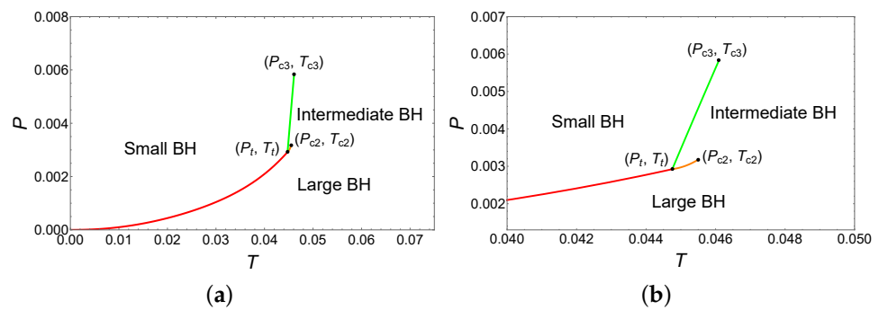
Figure 10. Phase diagram for the six-dimensional dyonic AdS BHs with H = 0.01 , \alpha_2 = 6 , and \eta = 0.01 . (a) Entire phase diagram. (b) An enlarged view near the triple point (P_t, T_t) .
