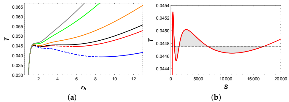
Figure 8. (a) T vs. r_h . The blue, red, black, orange, green, and gray curves correspond to P = 0.002 , 0.00292831 , 0.00317372 , 0.004 , 0.00583728 , and 0.007 , respectively. The solid and dashed curves represent stable and unstable branches, respectively. (b) T - S diagram of two pairs of equal area regions at a pressure of P = P_t = 0.00292831 . The horizontal line has a temperature of T = T_t = 0.0447573 .
