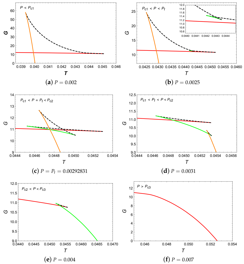
Figure 9. G vs. T . The red, green and orange curves represent the small, intermediate and large BHs, while the dashed curves indicate unstable BHs.
