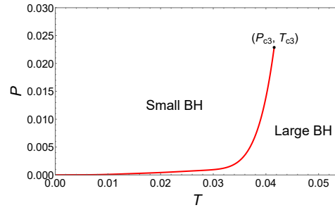
Figure 7. Phase diagram for the six-dimensional dyonic BHs with H = 0.01 , \eta = 0.01 and \alpha_2 = 10 .
