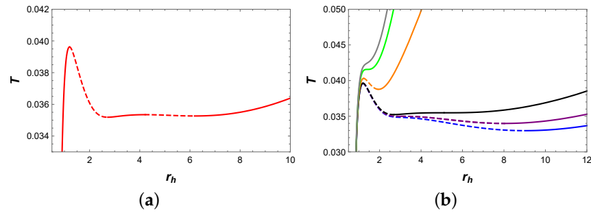
Figure 5. (a) T vs. r_h for P = 0.0019 . (b) T vs. r_h , where the blue, purple, black, orange, green and gray curves represent P = 0.0015, 0.0016521, 0.0019592, 0.01, 0.0228754 and 0.03 , respectively. Solid curves indicate stable branches, while dashed curves represent unstable branches.
