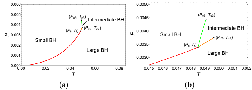
Figure 4. Phase diagram for the six-dimensional dyonic BHs with H = 0.01 , \eta = 0.01 and \alpha_2 = 5 . (a) Entire phase diagram. (b) An enlarged view near the triple point (P_t, T_t) .
