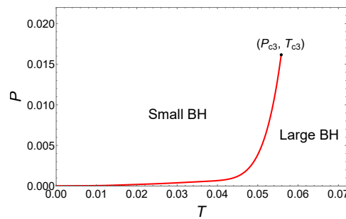
Figure 22. Phase diagram for the six-dimensional dyonic AdS BHs with \alpha_2 = 5 , \eta = 0.01 , and H = 1 .
