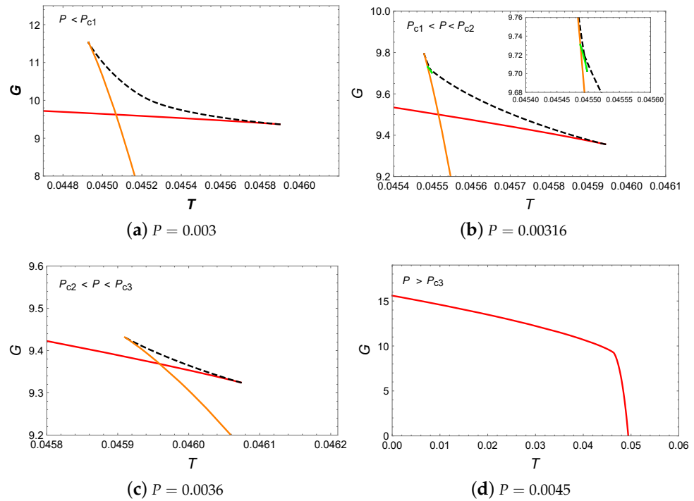
Figure 12. G vs. T . The red, green, and orange curves represent the small, intermediate, and large BHs, while the dashed curves indicate unstable BHs.
