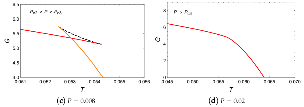
Figure 21. G vs. T . The red, green and orange curves represent the small, intermediate and large BHs, while the dashed curves indicate unstable BHs.
