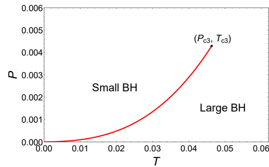
Figure 13. Phase diagram for the six-dimensional dyonic BHs with H = 0.01 , \alpha_2 = 6 , and \eta = 0.1 .
