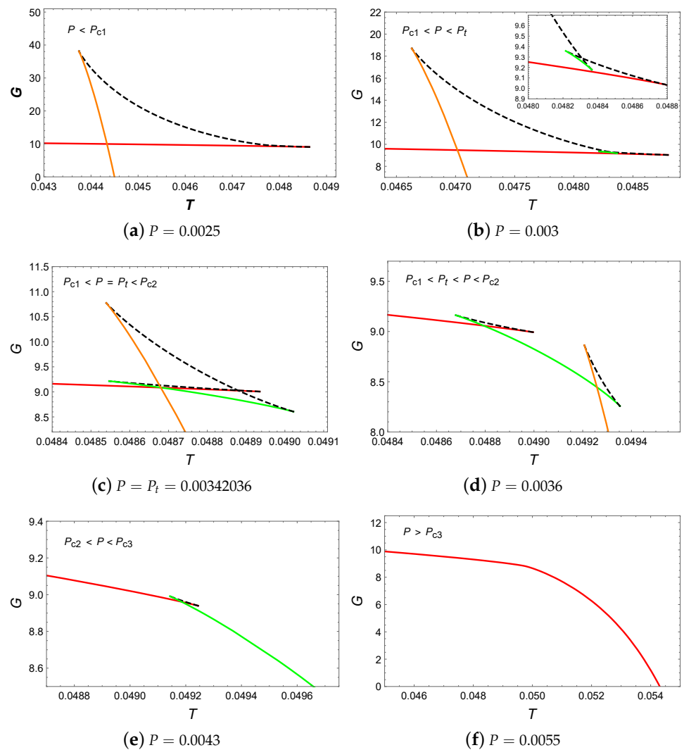
Figure 18. G vs. T . The red, green, and orange curves represent the small, intermediate, and large BHs, while the dashed curves indicate unstable BHs.
