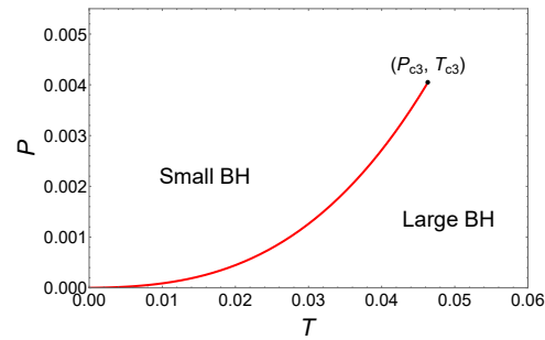
Figure 16. Phase diagram for the six-dimensional dyonic AdS BHs with H = 0.01 , \alpha_2 = 6 and \eta = 5 .
