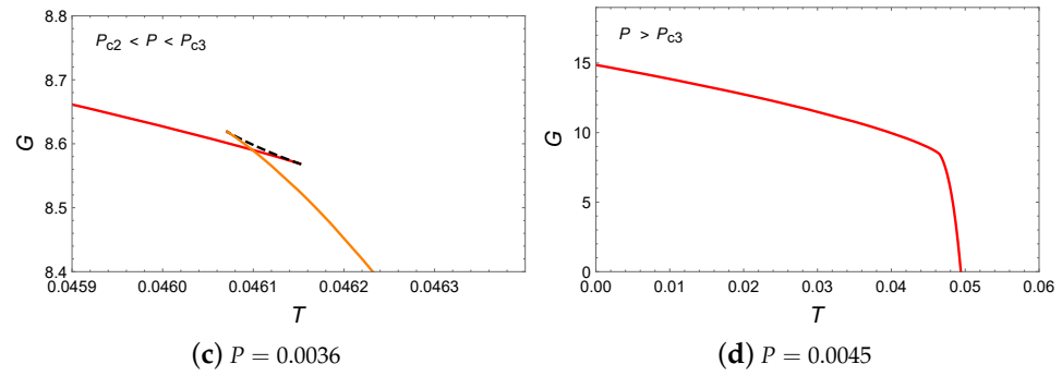
Figure 15. G vs. T . The red, green and orange curves represent the small, intermediate and large BHs, while the dashed curves indicate unstable BHs.
