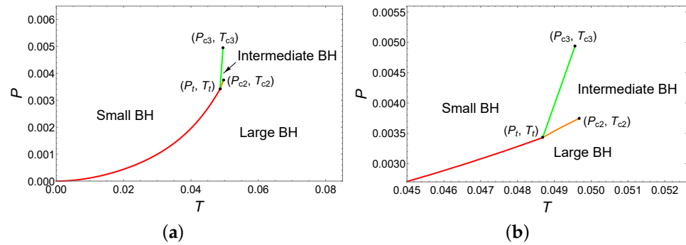
Figure 19. Phase diagram for the six-dimensional dyonic AdS BHs with \alpha_2 = 5 , \eta = 0.01 , and H = 0.1 . (a) Entire phase diagram. (b) An enlarged view near the triple point (P_t, T_t) .
