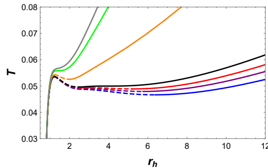
Figure 20. T vs. r_h , where the blue, purple, red, black, orange, green, and gray curves represent P = 0.003, 0.00326926, 0.0035, 0.00383222, 0.008, 0.0161884 , and 0.02 , respectively. The solid and dashed curves represent stable and unstable branches, respectively.
