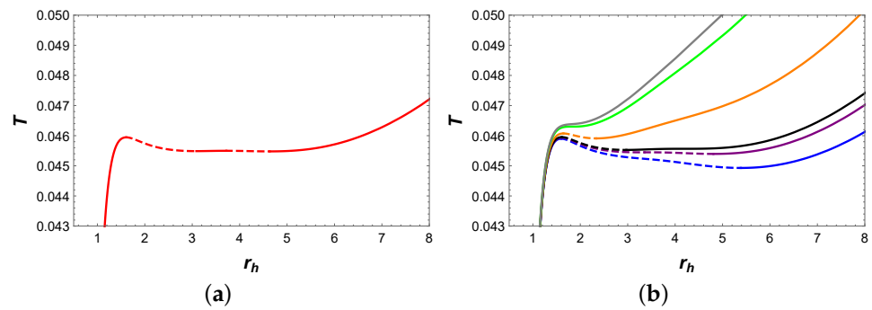
Figure 11. (a) T vs. r_h for P = 0.00316 . (b) T vs. r_h , where the blue, purple, black, orange, green, and gray curves represent P = 0.003, 0.00313279, 0.00319072, 0.0036, 0.00429228 , and 0.0045 , respectively. The solid and dashed curves represent stable and unstable branches, respectively.
