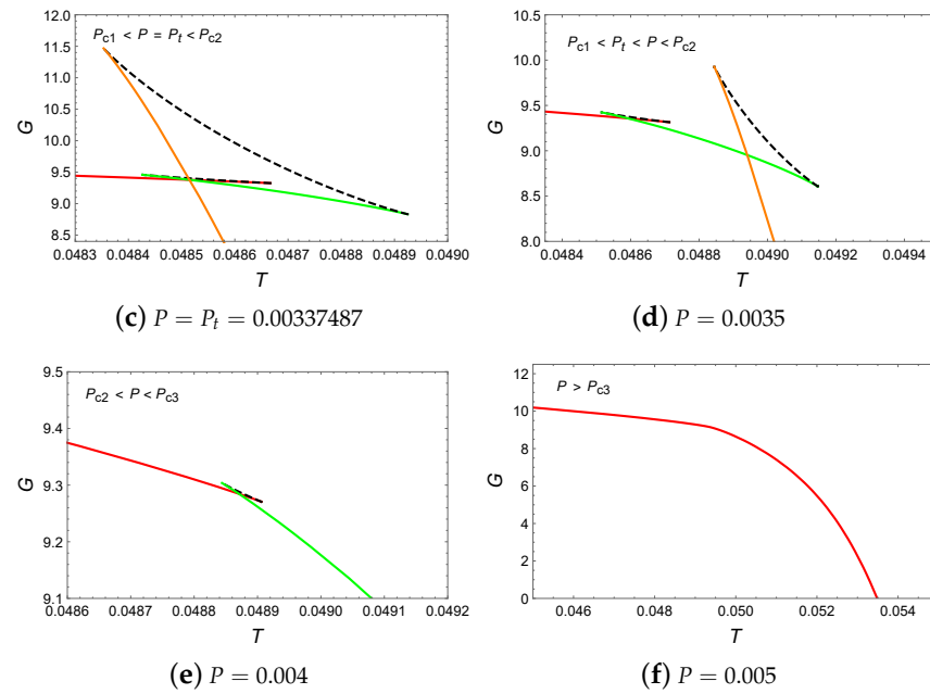
Figure 3. G vs. T . The red, green and orange curves represent the small, intermediate and large BHs, while the dashed curves indicate unstable BHs.
