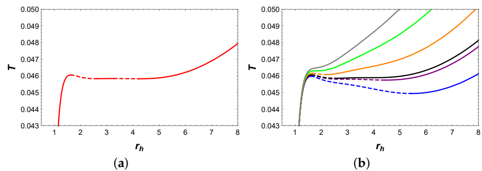
Figure 14. (a) T vs. r_h for P = 0.00327 . (b) T vs. r_h , where the blue, purple, black, orange, green, and gray curves represent P = 0.003, 0.00324087, 0.00329751, 0.0036, 0.00404979 , and 0.0045 , respectively. The solid and dashed curves represent stable and unstable branches, respectively.
