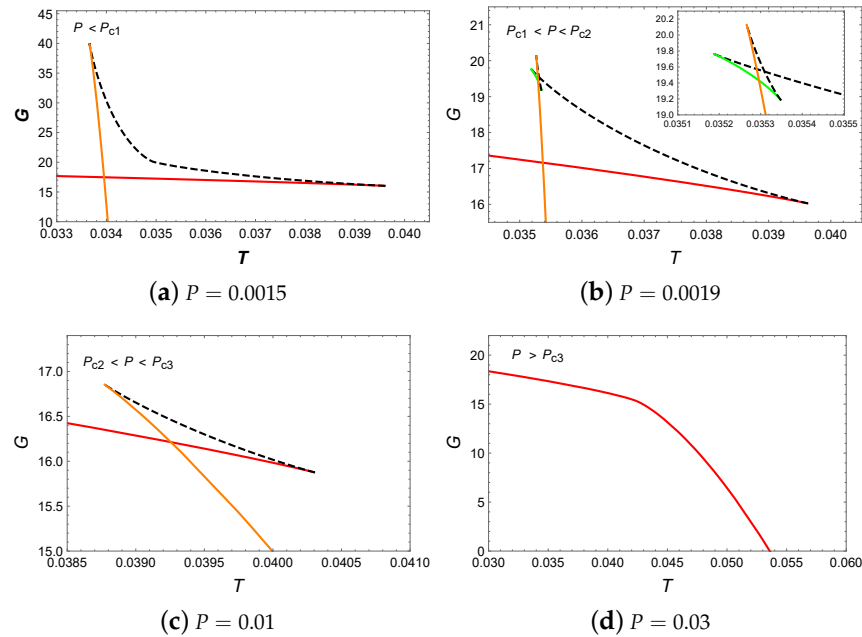
Figure 6. G vs. T . The red, green and orange curves represent the small, intermediate and large BHs, while the dashed curves indicate unstable BHs.
