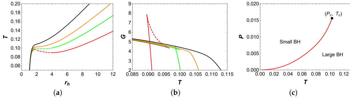
Figure 1. (a) Temperature T vs. horizon radius r_h . (b) Gibbs free energy G vs. temperature T . The red, green, orange, and black isobaric curves in (a,b) correspond to P = 0.01, 0.013, 0.0156174 , and 0.02 , respectively. Solid curves indicate stable branches, while dashed curves represent unstable branches. (c) P - T phase diagram for the six-dimensional dyonic BHs when H = 0.01 , \eta = 0.01 and \alpha_2 = 1 .
