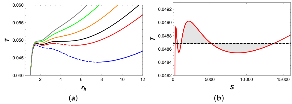
Figure 17. (a) T vs. r_h . The blue, red, black, orange, green, and gray curves corresponds to P = 0.0025 , 0.00342036, 0.00375132, 0.0043, 0.00494838, and 0.0055, respectively. The solid and dashed curves represent stable and unstable branches, respectively. (b) T - S diagram of two pairs of equal area regions at pressure P = P_t = 0.00342036 . The horizontal line has a temperature T = T_t = 0.0486811 .
