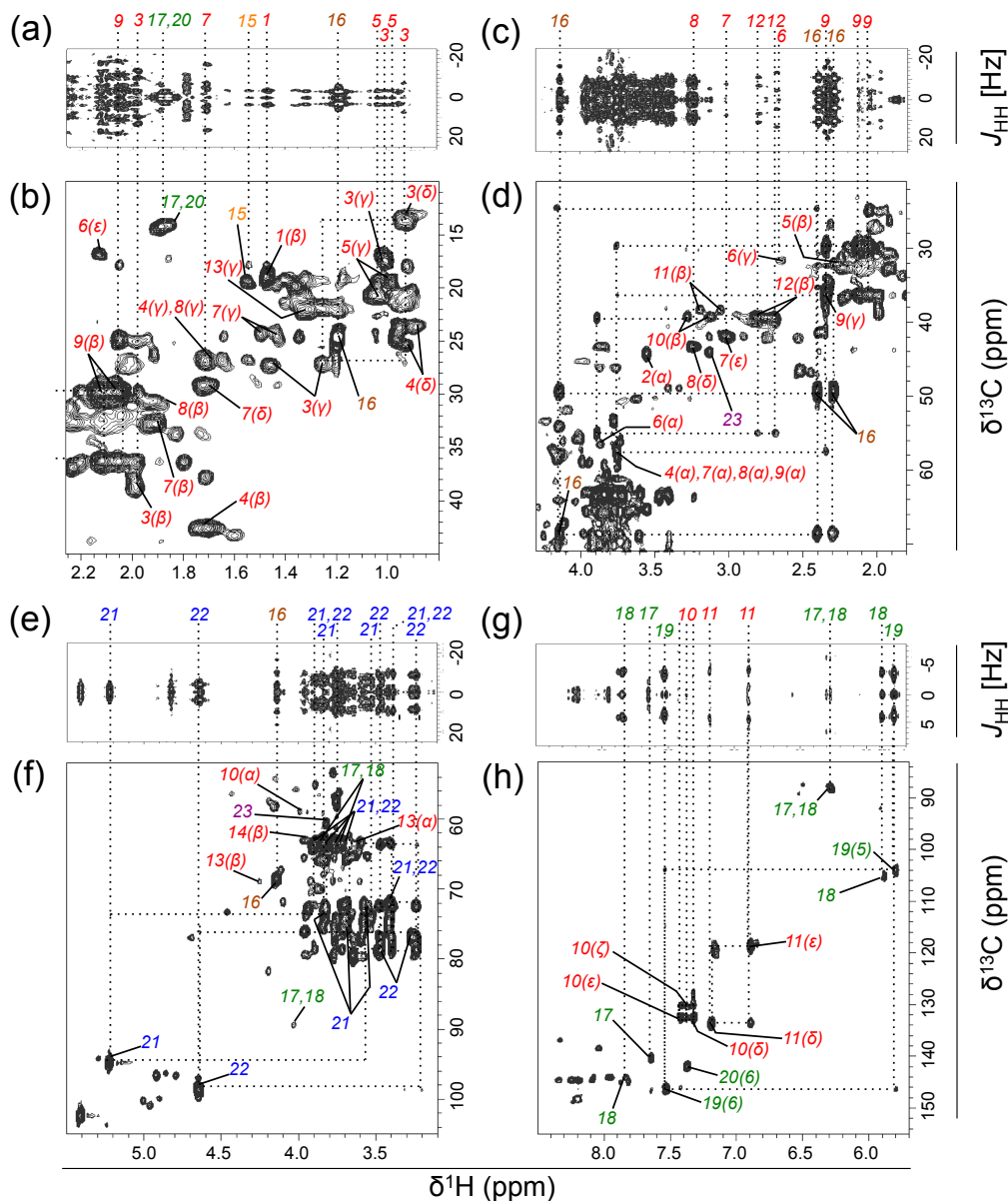
Figure 1. ^{13}\text{C} -decoupled two-dimensional ^1\text{H} - ^1\text{H} J -resolved spectroscopy (2D- J -res-dc) (a,c,e,g) and ^1\text{H} - ^{13}\text{C} heteronuclear single quantum coherence-total correlation spectroscopy (HSQC-TOCSY) (b,d,f,h) spectra for metabolites transformed from ^{13}\text{C}_6 -glucose by a natural aquatic bacterial community (final concentration added, 500\ \mu\text{M} C) (Experiment 1). Signals were obtained after a 2-day incubation of a seawater sample collected from a coastal location. Spectra for the \delta^1\text{H} ( \delta^{13}\text{C} ) ranged from 0.8 to 2.26 (10–45) (a,b); 1.8–4.3 (21–71) (c,d); 3.1–5.5 (52–105) (e,f); and 5.7–8.5 (83–155) ppm (g,h) are shown. Numbers indicate the corresponding metabolites listed in Table 1 (amino acids: red; dipeptides: orange; carboxylic acids: brown; nucleosides and nucleobases: green; carbohydrates: blue; amino alcohols: purple). Greek letters or numbers in parentheses for amino acids and nucleobases, respectively, denote the atom designation. In (a), an increased ( \times 6 ) contour intensity magnitude was used for the \delta^1\text{H} range 1.6–2.26 ppm relative to the rest of the field (0.8–1.6 ppm). For the detailed analytical settings, see Table S1.
