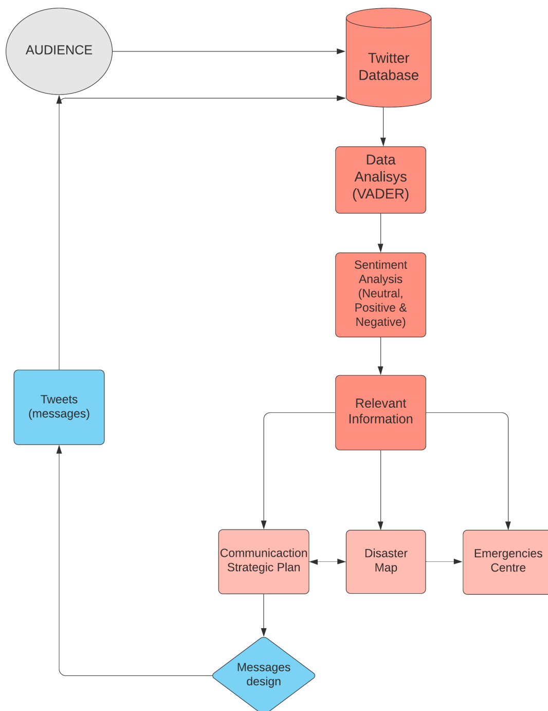
Figure 4. Flowchart. Source: own elaboration.
