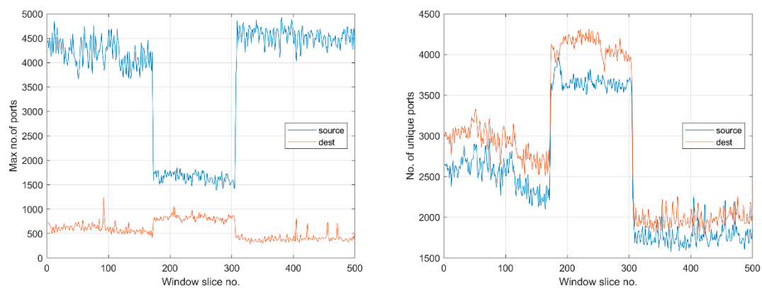
Figure 6. Maximum number of ports and the number of unique ports in NetFlow window slices.
