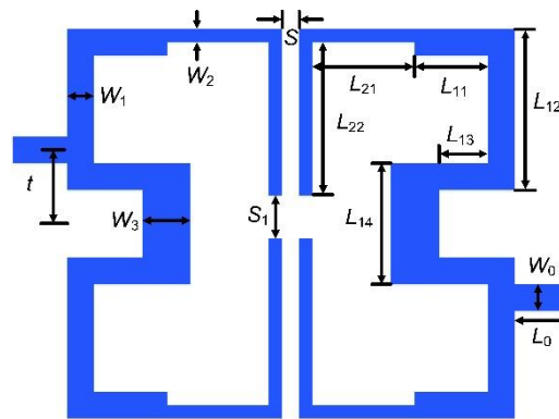
Figure 3. Schematic diagram of dual-wideband bandpass filters (BPF).
