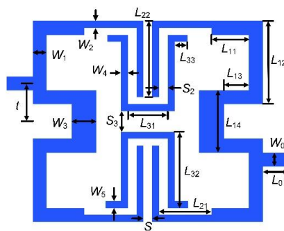
Figure 5. Schematic diagram of tri-wideband BPF.
