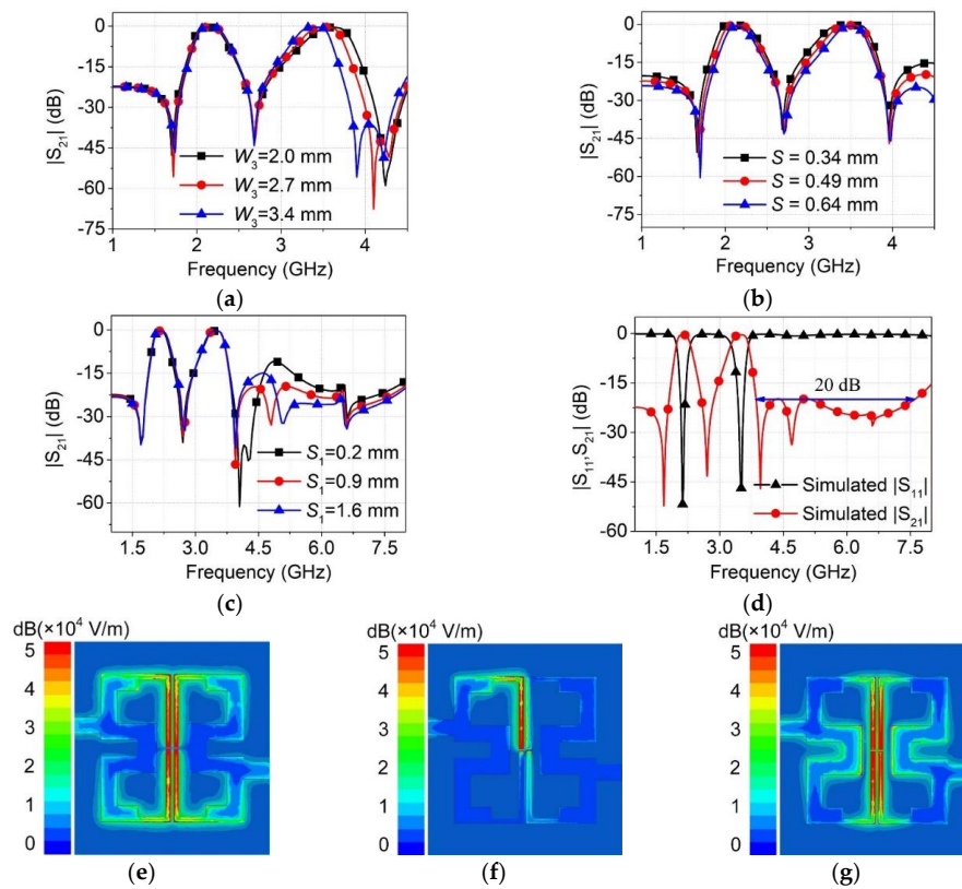
Figure 4. Simulation of dual-wideband bandpass filters (BPF). (a) The simulated |S_{21}| response of the filter for various widths of W_3 ; (b) The simulated |S_{21}| response of the filter for various widths of S ; (c) The simulated |S_{21}| response of the filter for various widths of S_1 ; (d) Simulated |S_{21}| , |S_{11}| response of the dual-wideband BPF; (e) The simulated electric fields distributions of the dual-wideband BPF at 2.14 GHz; (f) The simulated electric fields distributions of the dual-wideband BPF at 2.68 GHz; (g) The simulated electric fields distributions of the dual-wideband BPF at 3.5 GHz.
