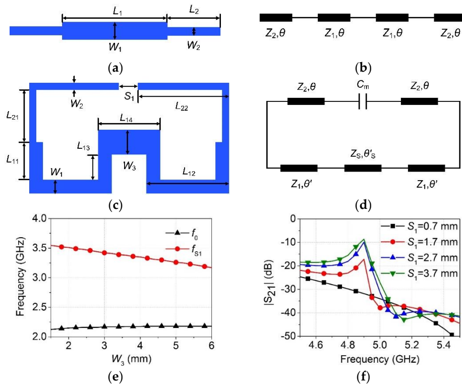
Figure 1. Design of folded open-loop stepped-impedance resonators (FOLSIR). (a) Schematic diagram of stepped-impedance resonators (SIR); (b) The equivalent circuit diagram of the SIR; (c) Schematic diagram of FOLSIR; (d) The equivalent circuit diagram of the FOLSIR; (e) The simulated resonant frequency f_0 and f_{S1} of the FOLSIR for various values of W_3 ; (f) The simulated |S_{21}| response of the resonator for various values of S_1 .
