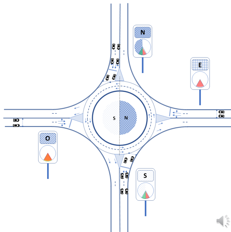
Figure 1. An example of a synchronous revolving roundabout with rotating priorities and staggered platoons.
