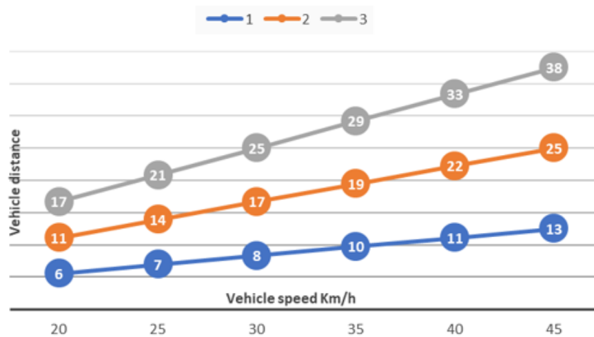
Figure 11. Inter-vehicle distance vs. gap in seconds and speed.
