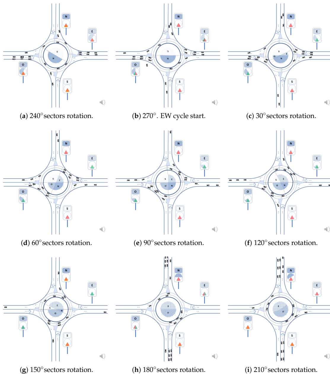
Figure 9. East-West (EW) access sequence. (a,b) show the completion of NS cycle. (b) shows the upcoming priority period for the east and west accesses. From (b) to (h), platoons at EW entries have priority. In (i) all entries are closed, and the roundabout empties.
