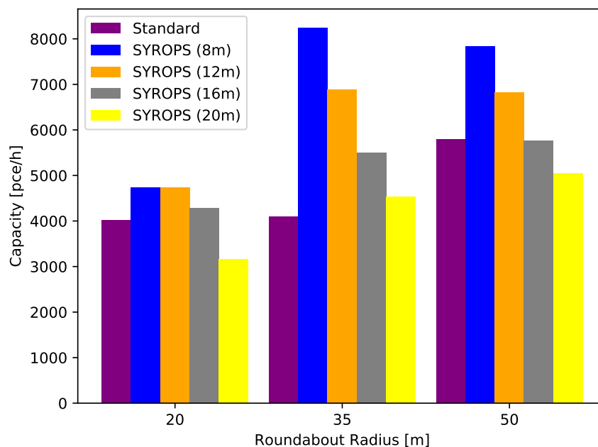
Figure 15. Roundabout capacity comparison versus size of the roundabout for standard roundabouts and SYROPS with and without platooning.
