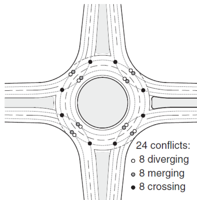
Figure 2. Conflict points in a standard roundabout [5].
