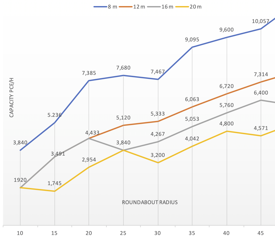
Figure 13. Maximum roundabout capacities vs. vehicle distances and roundabout radius.
