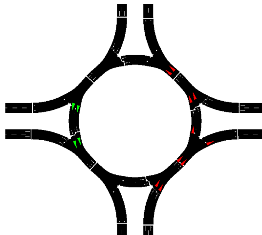
Figure 18. Snapshot of the SUMO simulation. Unbalanced traffic north–south. More vehicles from the south (red) and less vehicles from the north (green) enter the roundabout to compensate the traffic unbalance.
