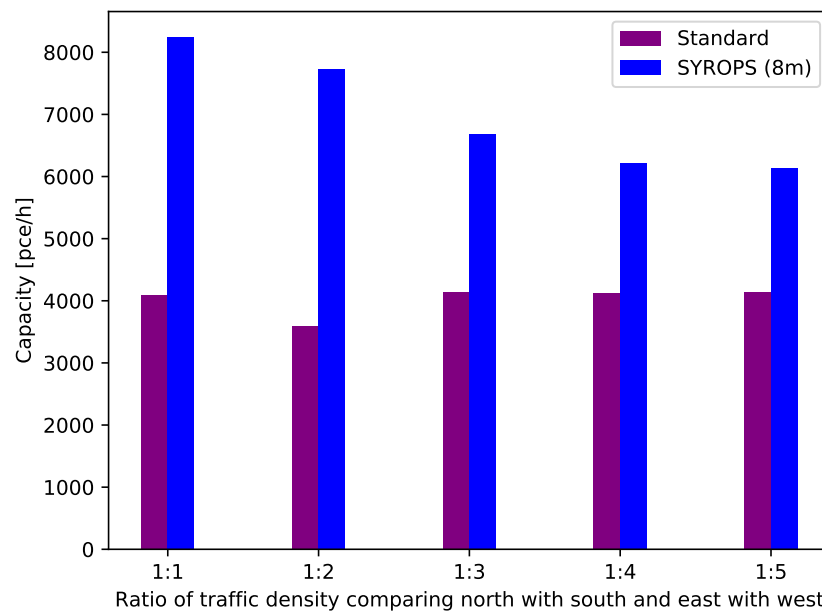
Figure 17. Roundabout capacity in vehicles per hour as a function of traffic unbalance ratio from opposing directions (N vs. S, E vs. W).
