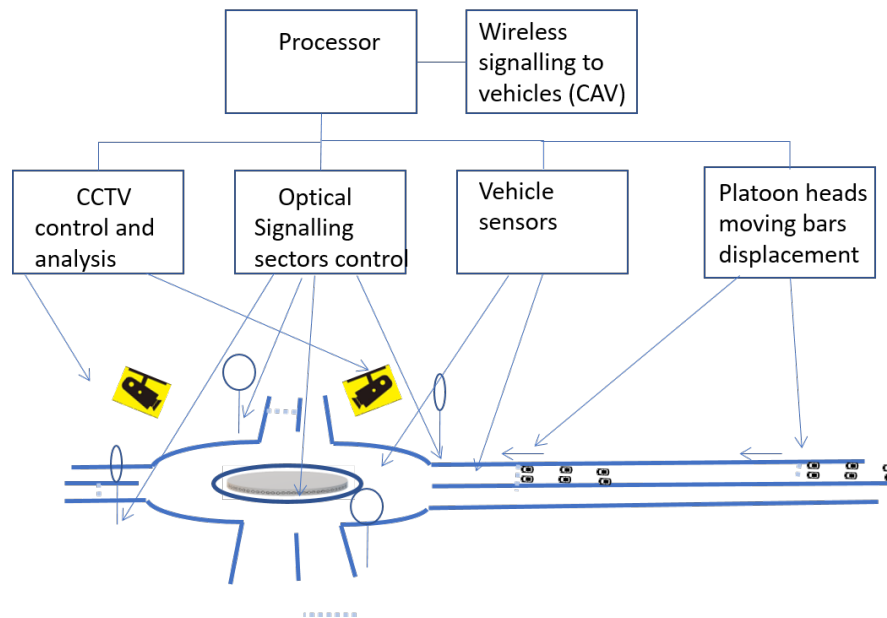
Figure 4. Block diagram of roundabout control.
