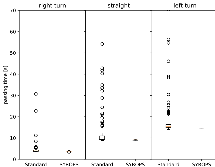
Figure 16. Roundabout delay per direction of travel for a roundabout radius of 35 m.
