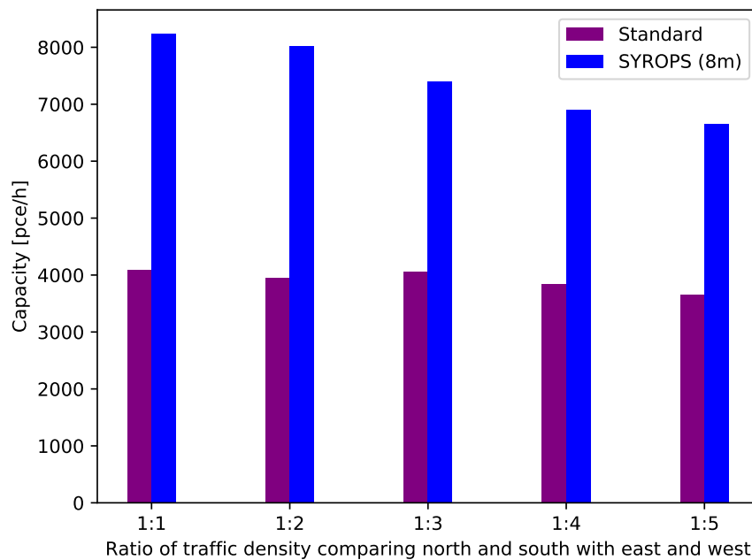
Figure 19. Roundabout capacity in vehicles per hour depending on the level of unbalance ratio between orthogonal directions (N–S vs. E–W).
