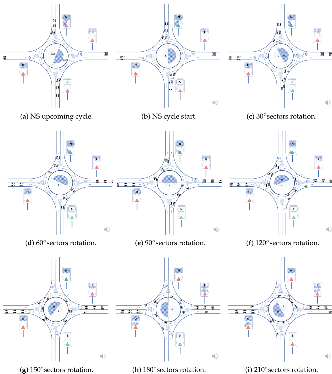
Figure 8. North-South (NS) access sequence. (a) shows the upcoming priority period for the north and south accesses. From (b) to (h), platoons at NS entries have priority. In (i) all entries are closed, and the roundabout empties.
