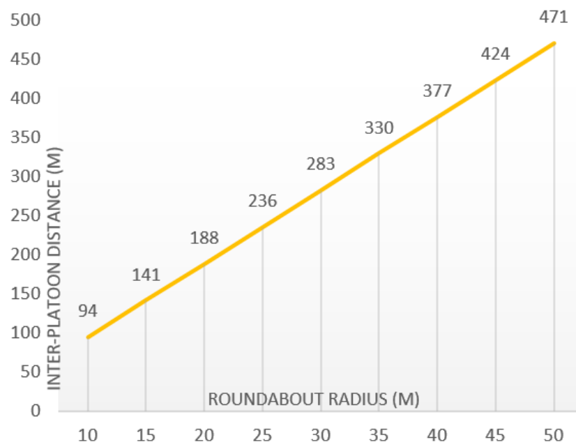
Figure 21. Inter-platoon distances versus roundabout radius.
