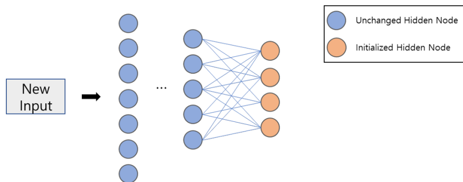
Figure 3. Transfer learning concept used in the proposed scheme.
