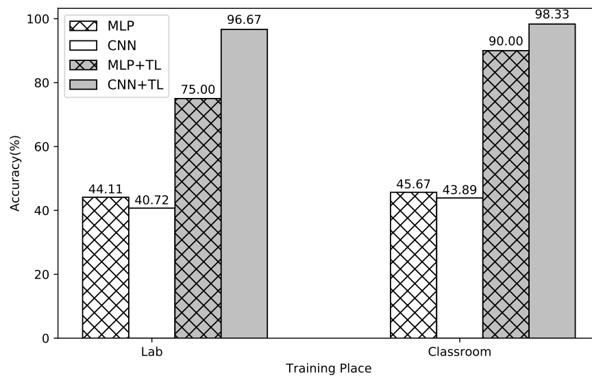
Figure 6. UWB channel classification accuracy of different training places and models.
