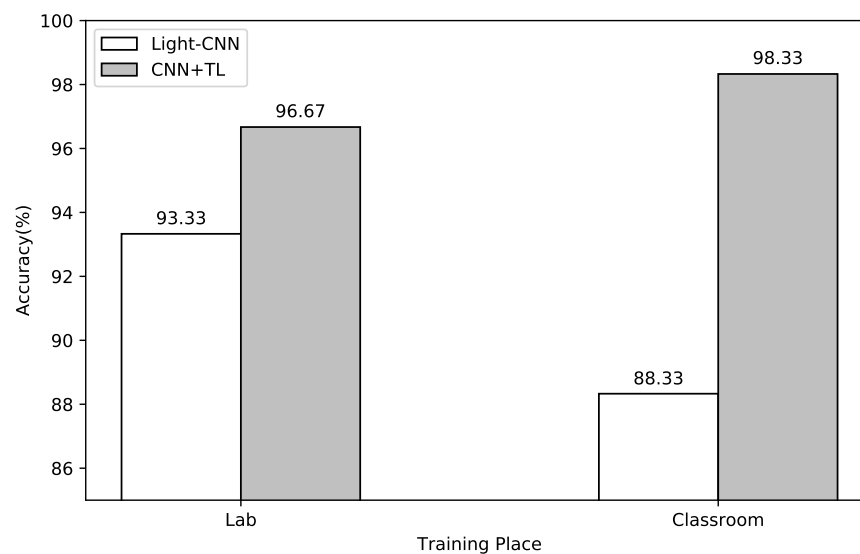
Figure 7. UWB channel classification accuracy of the light CNN and CNN with TL in different places.
