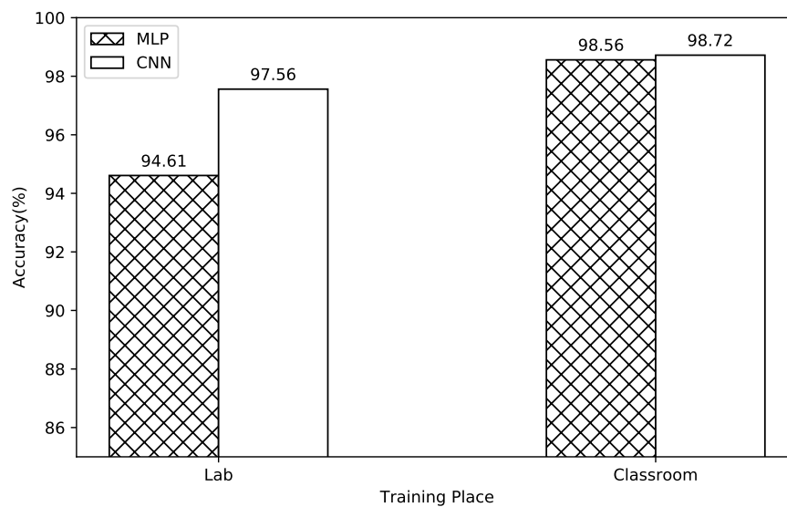
Figure 5. UWB channel classification accuracy of the MLP and CNN in the measured environment.
