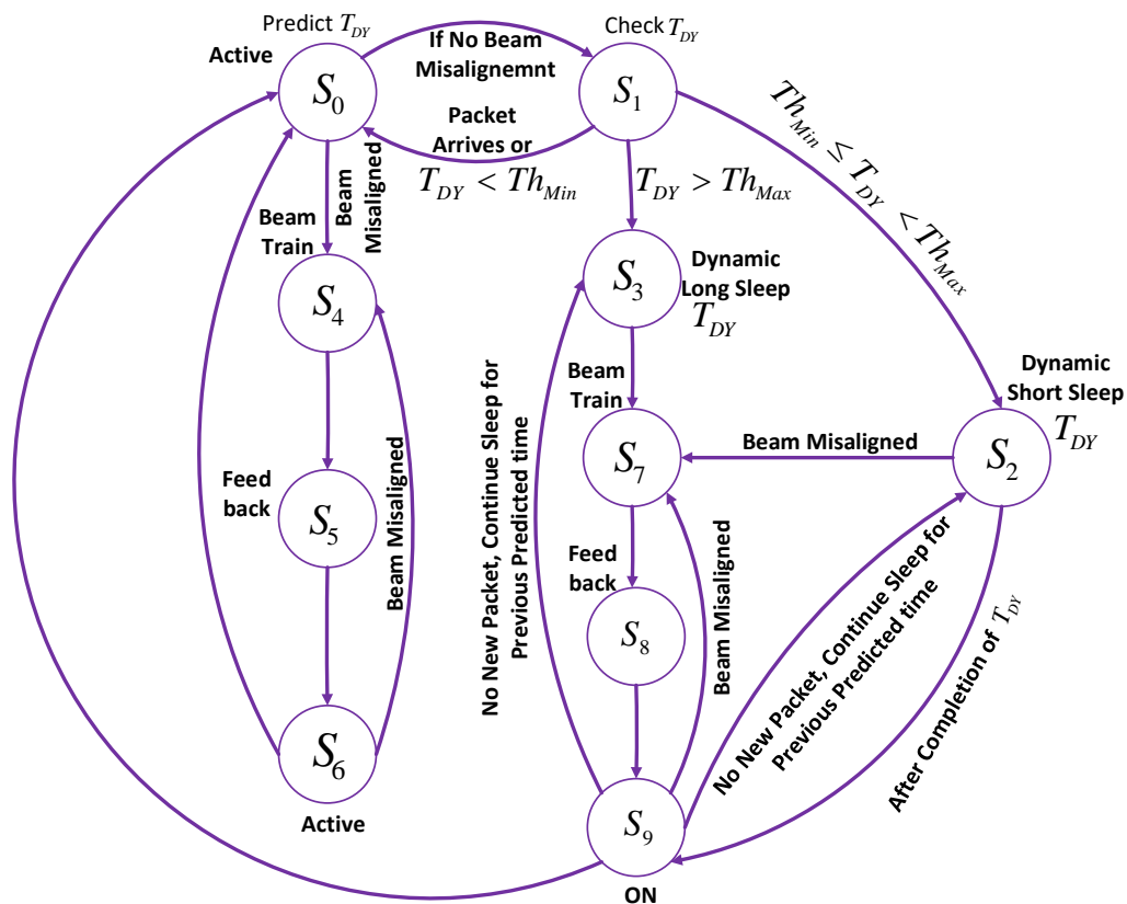
Figure 5. State diagram for AI-DRX.
