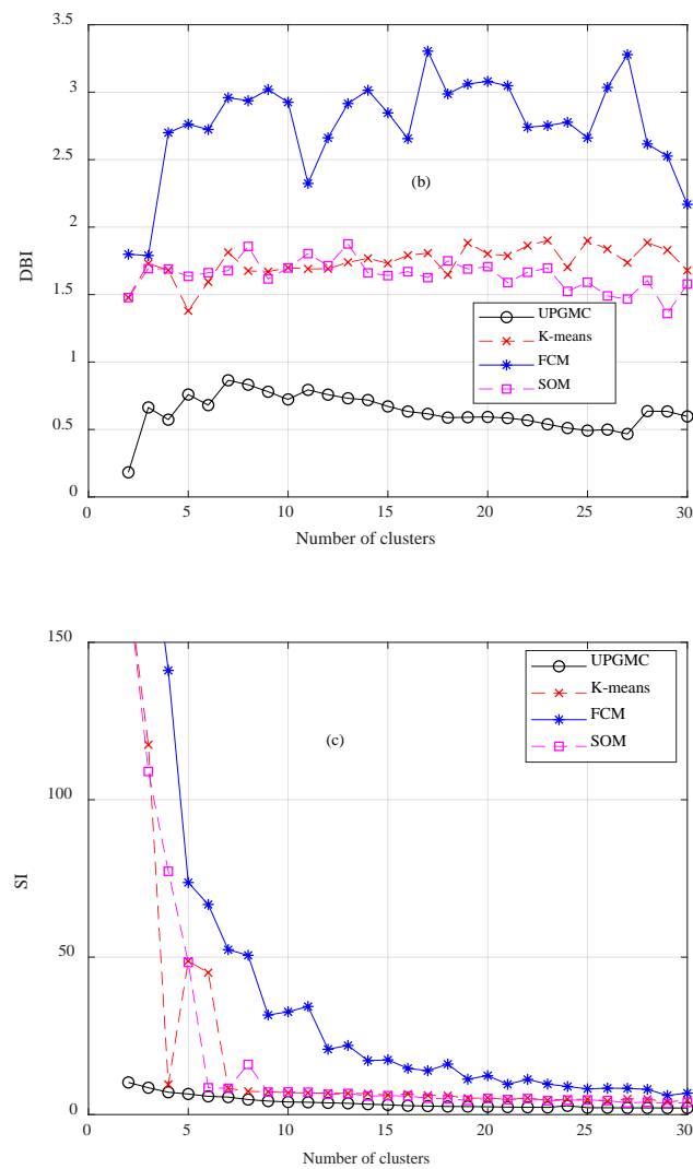
Figure 7. Algorithms comparison using: (a) J; (b) DBI; (c) SI indicators. The patterns dimension is D = 1440 .
