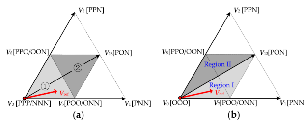
Figure 5. The division of small regions in Sector Z_1 . (a) Conventional strategy; (b) improved strategy.
