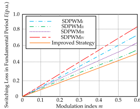
Figure 7. Switching loss figure at \varphi = \pi/4 .
