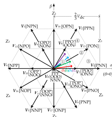
Figure 2. Space vector diagram of the three-level inverter.
