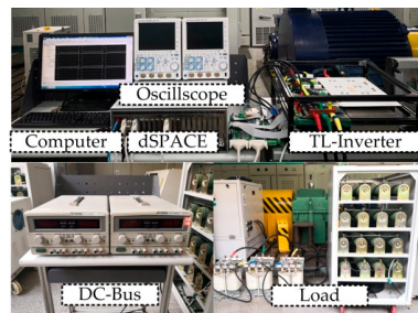
Figure 8. Physical figure of experimental system.
