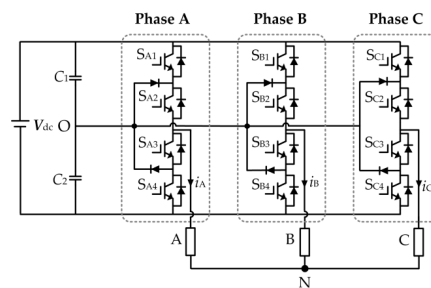
Figure 1. Topology of NPC three-level inverter.
