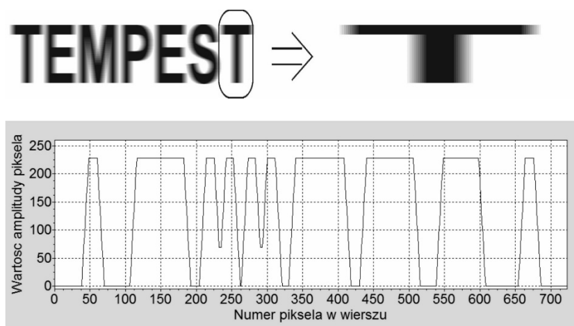
Figure 3. Application effect of a low-pass filter on the output of the VGA video standard.
