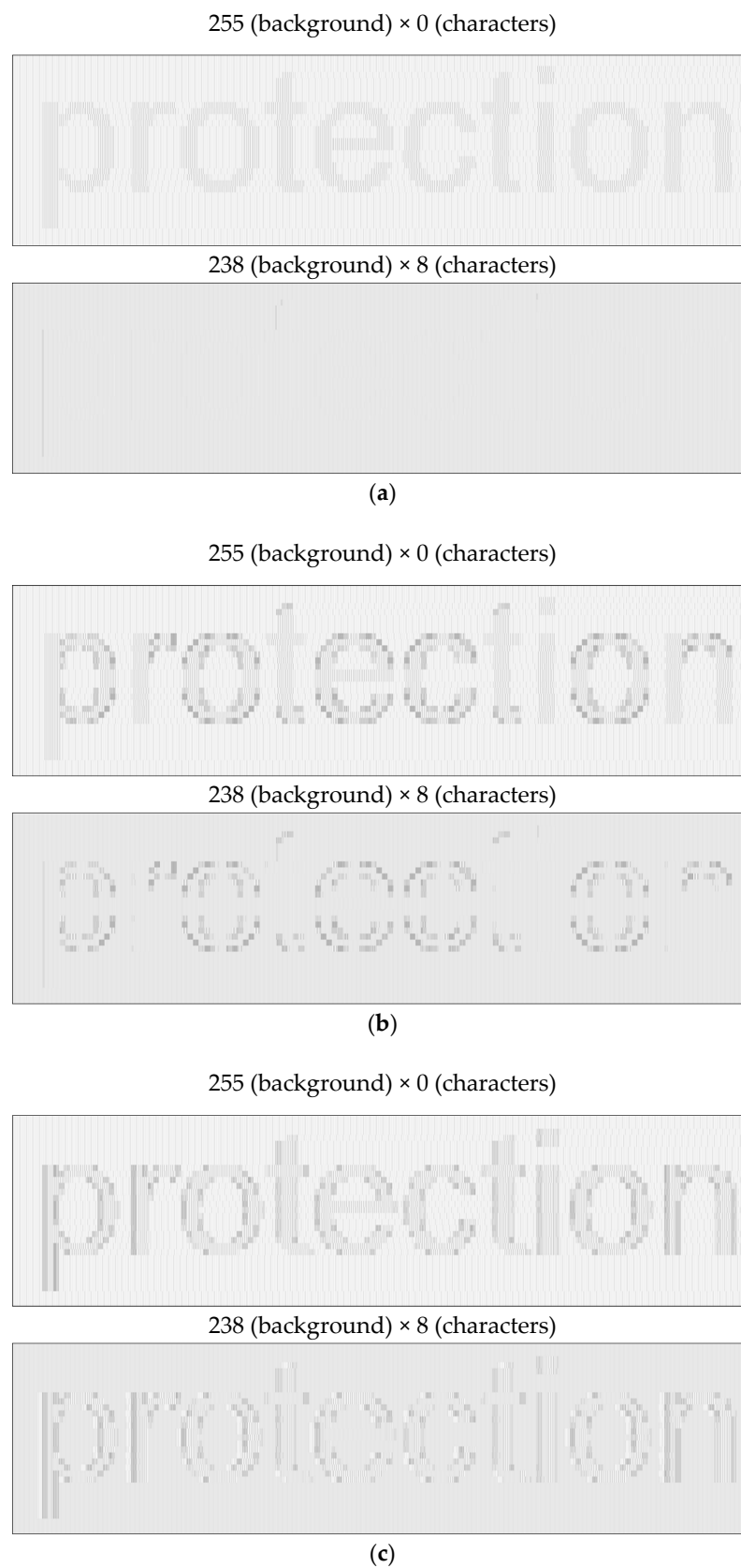
Figure 12. Examples of images obtained based on compromising emanations for different color pairs (background and characters) and for three edge smoothing modes (using Windows XP OS) for theoretical analysis: (a) without an edge smoothing mode, (b) Standard edge smoothing mode, and (c) ClearType edge smoothing mode.
