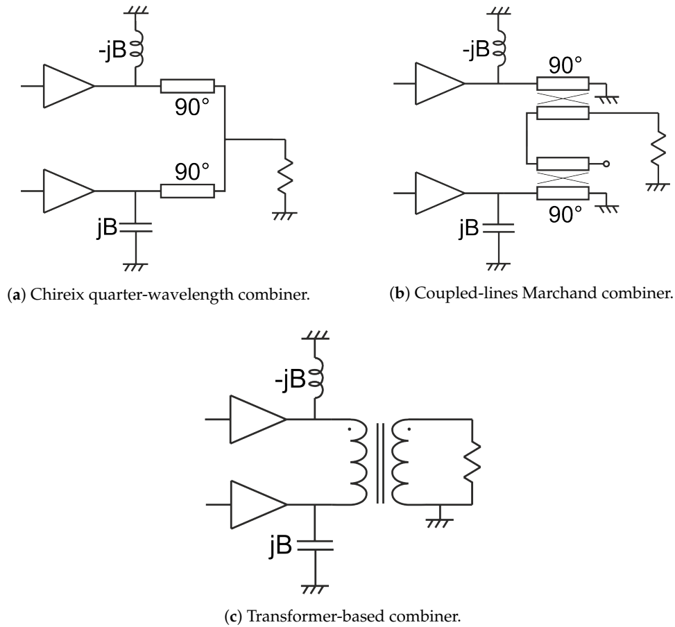
Figure 14. Typical balun topologies adopted for the Chireix PA output combiner.
