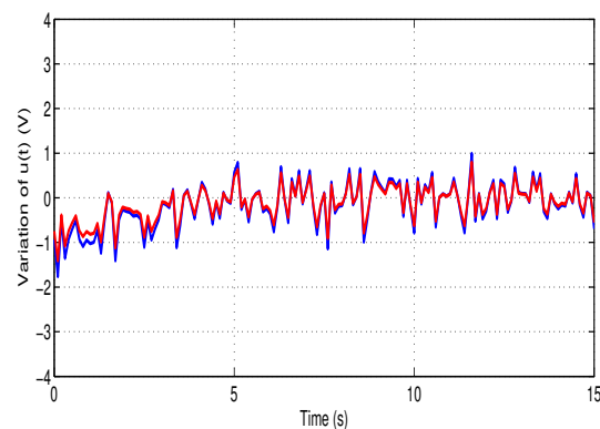
Figure 4. Control \bar{u}(t) variation for NEMF ( \bar{u}_1(t) )-blue and \bar{u}_2(t) -red.
