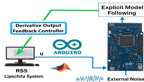
Figure 1. RTI diagram.
