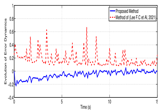
Figure 5. Evolution of error dynamics under proposed EMF controller and [16].
