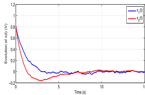
Figure 2. The evolution of states \bar{x}(t) under the proposed EMF controller.
