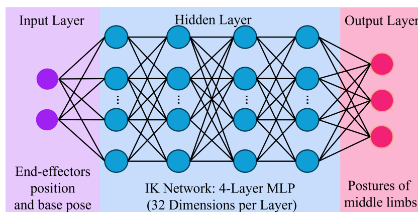
Figure 3. Overview of the Inverse Kinematics Network (IK-N) based on MLP. The MLP takes torso posture and limb-end positions as input and outputs estimated joint angles for full-body posture estimation.
