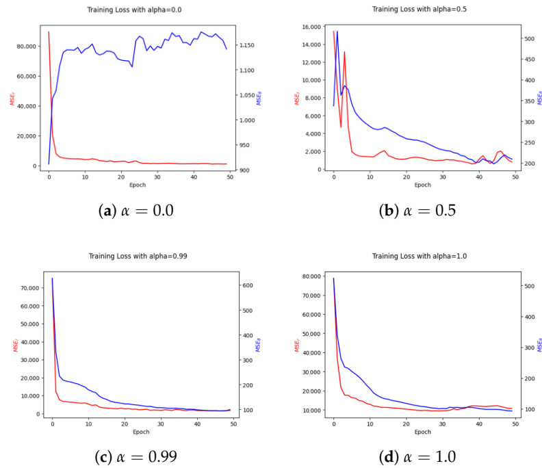
Figure 7. Trends of loss reduction during training. The red line represents the IK-N loss function L_{\theta} , and the blue line represents the PINN loss function L_K . The effect of PINN varies according to the value of \alpha . In (a), where kinematics is not considered, L_K does not decrease at all. In (b), with \alpha = 0.5 , the kinematic results are improved by PINN. In (c,d), with \alpha = 0.99 and \alpha = 1.0 , respectively, it is observed that convergence is faster with \alpha = 0.99 , which considers position errors, than with \alpha = 1.0 , which does not consider position errors at all.
