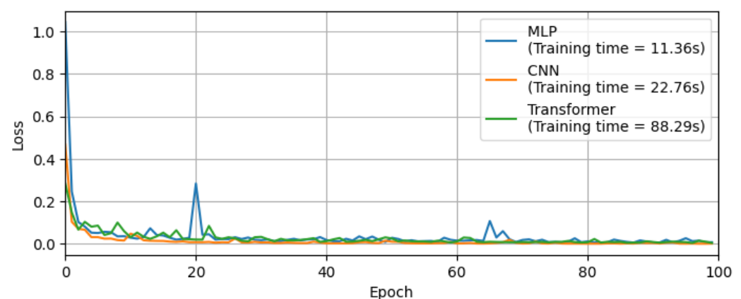
Figure 12. Learning curves and training time for simple angle estimation using MLP, CNN, and Transformer architectures. The MLP achieves training speeds approximately twice as fast as CNN and eight times faster than Transformer, while maintaining sufficient nonlinear expressive power for effective implementation within the PINN framework.
