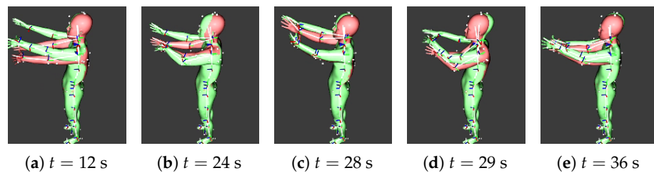
Figure 9. The experimental results of IK-N using PINN ( \alpha = 0.99 ). The green and red bodies represent the true and estimated poses, respectively. The parameter t corresponds to the same timing as in Figure 8. By utilizing PINN, the estimation accuracy of the elbow joint has improved, leading to a highly precise reconstruction of the hand position.
