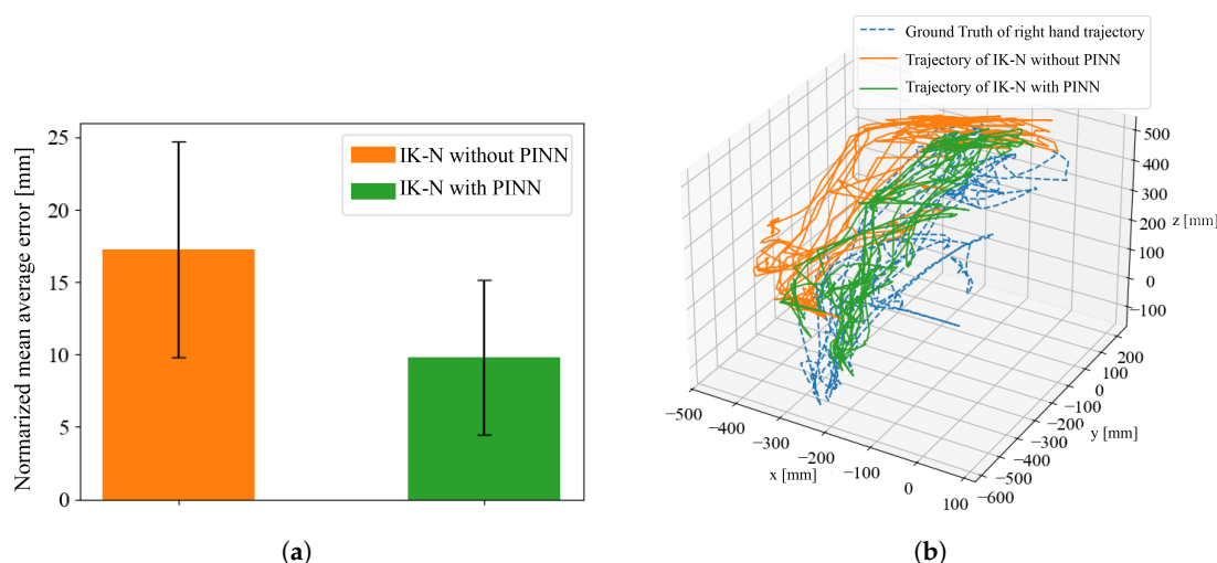
Figure 10. Comparison of mean average error between IK-N model with and without PINN. (a) The normalized mean errors and their corresponding standard deviations. (b) Each right-hand trajectory used in this analysis.
