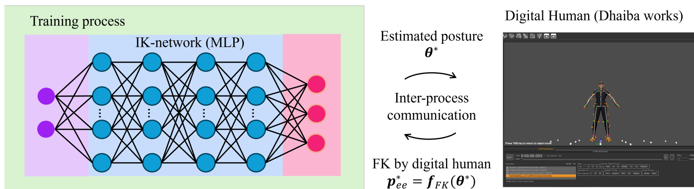
Figure 5. Digital Human Model (DhaibaWorks) for in-the-loop IK-N training. The digital human model can be integrated into the MLP training system as a set of physical laws representing human-like motion, enabling in-the-loop training. For more details on DhaibaWorks, please refer to [23].
