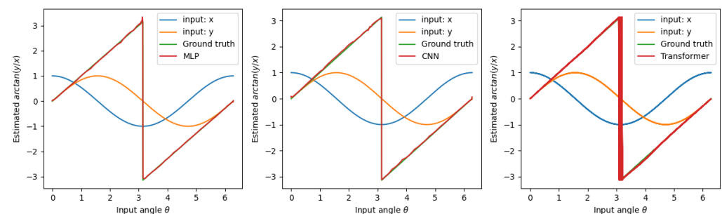
Figure 11. Comparison of simple angle estimation problem using MLP, CNN, and Transformer architectures. Despite its simplicity, MLP demonstrates comparable expressive power for nonlinear phenomena relative to more complex inference models. Due to its sequence-based learning mechanism, the Transformer requires approximately ten times more data to stably represent discontinuities.
