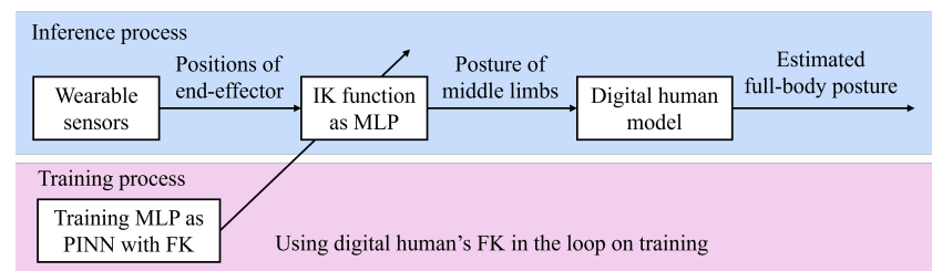
Figure 2. Overview of the proposed system for full-body posture estimation. The system integrates wearable sensors, a digital human model, and a PINN to achieve accurate posture estimation from torso and limb-end data.
