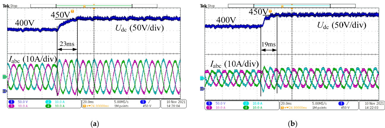
Figure 29. Single-loop state feedback control voltage step response when changing grid voltage: (a) Step response of voltage under single-loop state feedback control when reducing grid voltage; (b) step response of voltage under single-loop state feedback control when increasing grid voltage.
