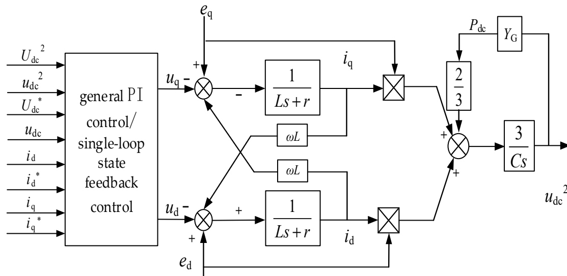
Figure 3. Grid-connected converter linear model structure.
