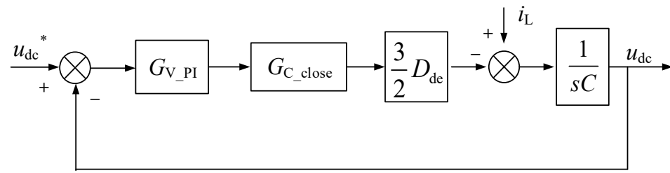
Figure 5. Block diagram of traditional PI control double-closed-loop.
