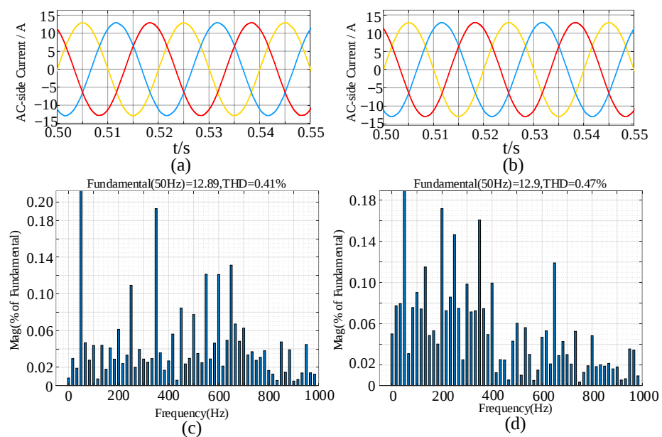
Figure 20. Harmonic analysis of the AC-side current under double-loop PI control and single-loop state feedback control: (a) Waveform of the AC-side current under traditional PI control; (b) waveform of the AC-side current under single-loop state feedback control; (c) FFT Analysis of the AC-side current under traditional PI control; (d) FFT analysis of the AC-side current under single-loop state feedback control.
