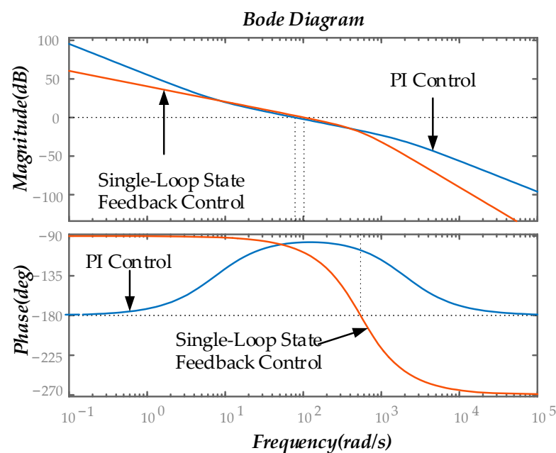
Figure 12. Bode diagram comparison.
