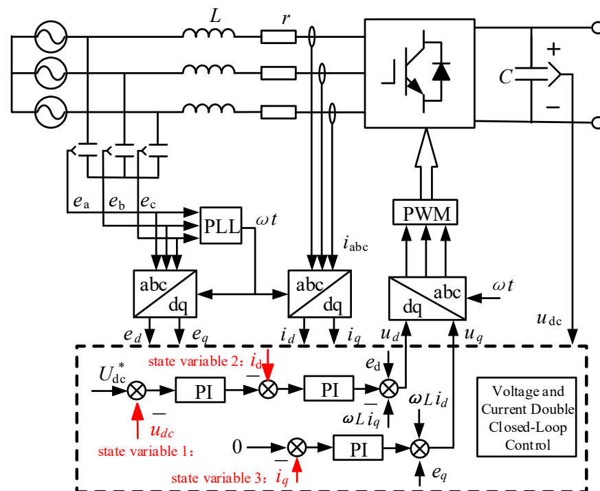
Figure 4. Grid-connected converter general control structure diagram.
