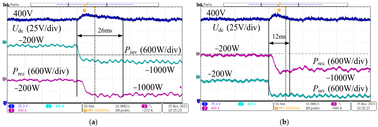
Figure 27. Comparison of bus voltage fluctuation between two control strategies when transmitting reverse power: (a) Bus voltage fluctuations under PI control; (b) bus voltage fluctuations under single-loop state feedback control.
