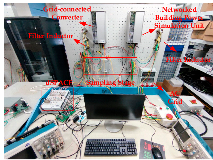
Figure 21. Experimental hardware configuration.
