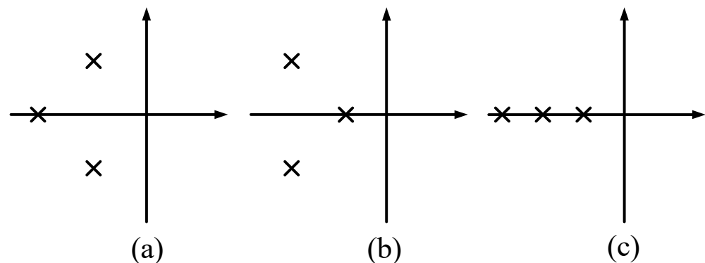
Figure 10. Pole configuration mode.
