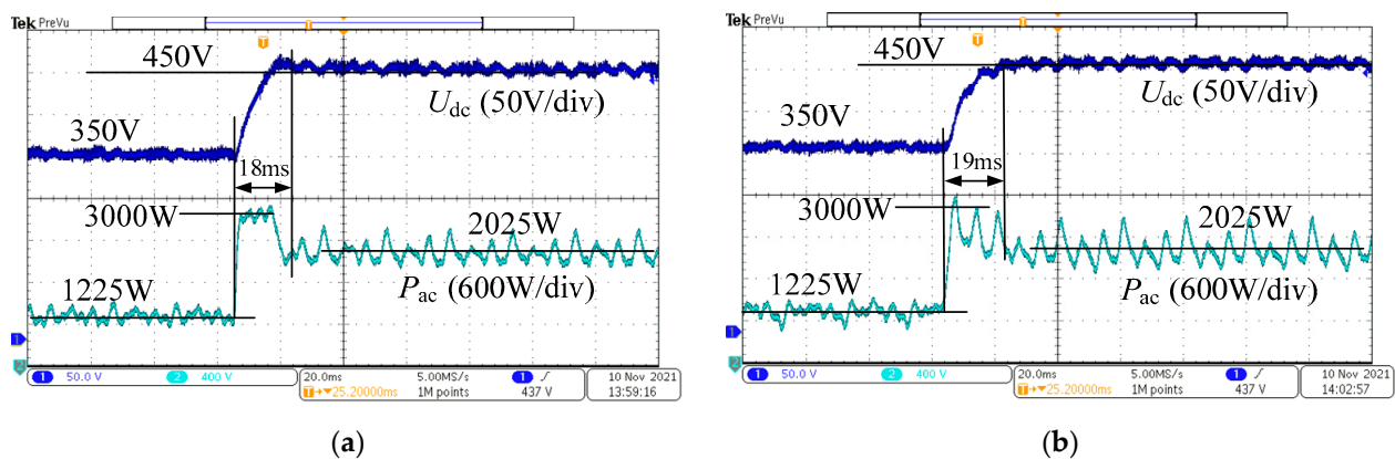
Figure 25. Comparison of dynamic characteristics between two control strategies after adjustment: (a) Step response of grid-tied converter under adjusted PI control; (b) step response of grid-tied converter under adjusted single-loop state feedback control.
