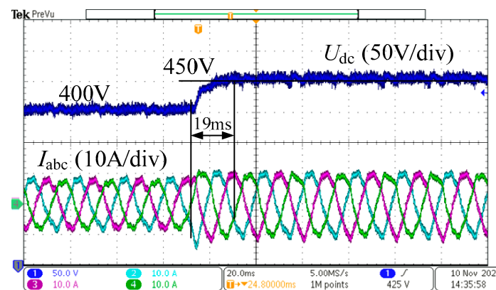
Figure 28. Single-loop state feedback control voltage step response when reducing inductance.
