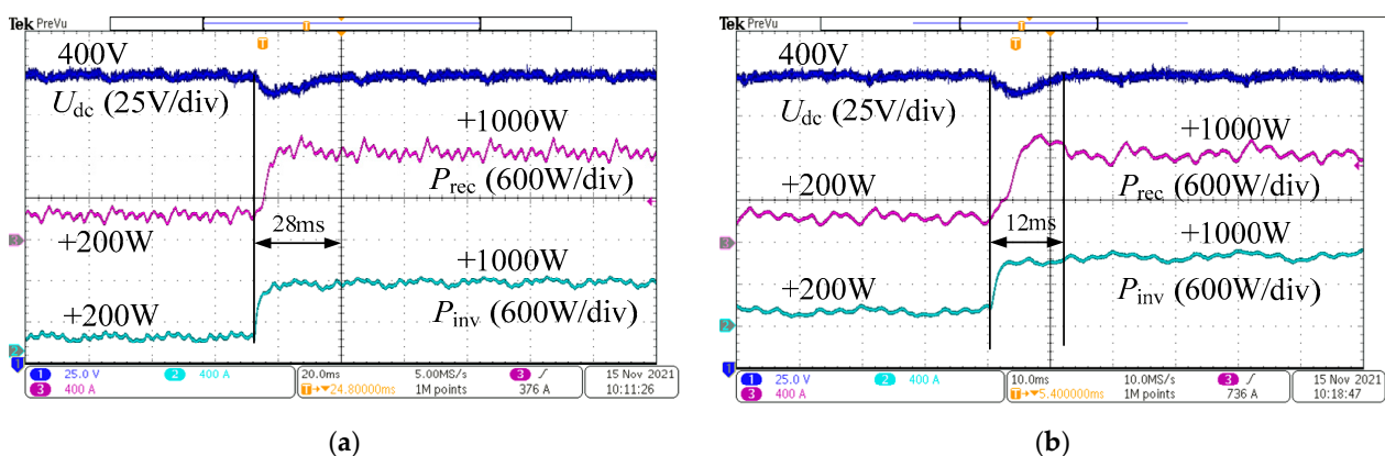
Figure 26. Comparison of bus voltage fluctuation between two control strategies when transmitting forward power: (a) Bus voltage fluctuations under PI control; (b) bus voltage fluctuations under single-loop state feedback control.
