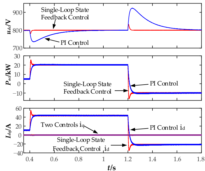
Figure 17. Bus voltage fluctuation under power disturbance.
