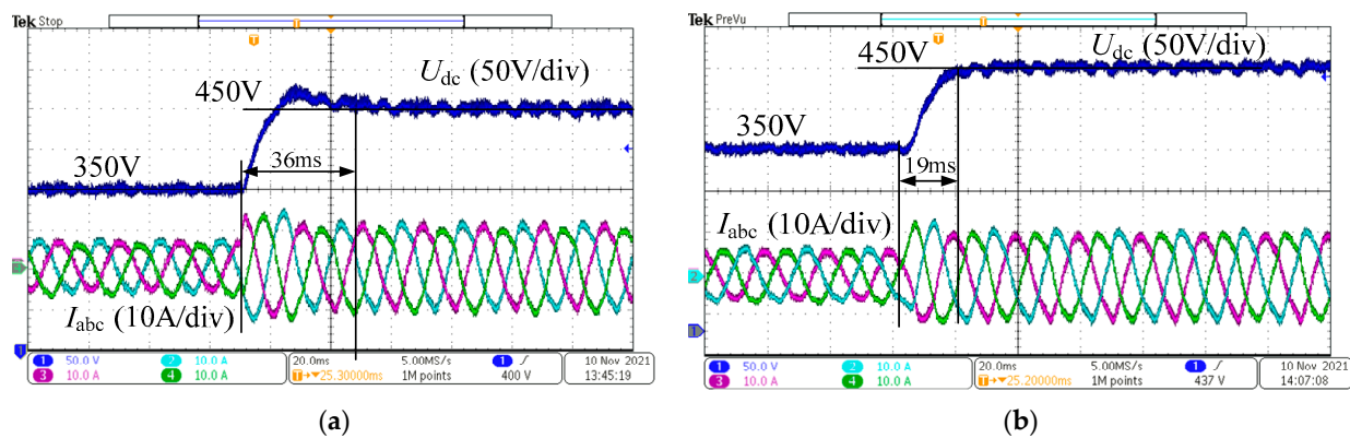
Figure 23. Comparison of experimental results of the dynamic characteristics of two control strategies: (a) Step response of grid-tied converter under PI control; (b) step response of AC/DC converter under single-loop state feedback control.
