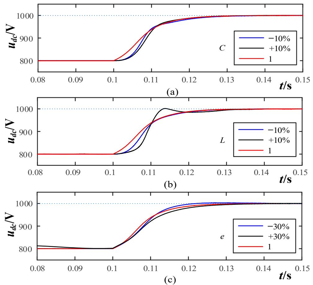
Figure 19. Comparison of voltage step response and disturbance characteristics with variable integral parameters: (a) DC-side capacitor variation response curve; (b) AC-side filtering inductor variation response curve; (c) grid voltage variation response curve.
