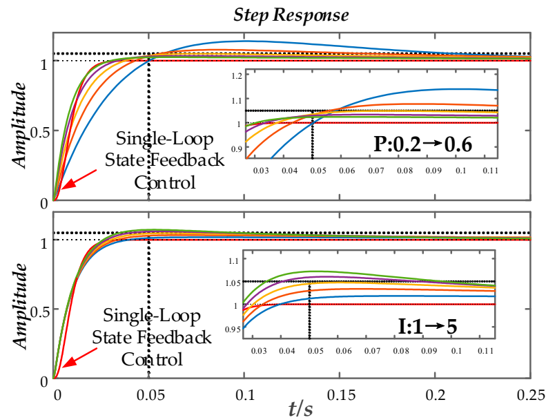
Figure 13. Change the PI parameter step response diagram.
