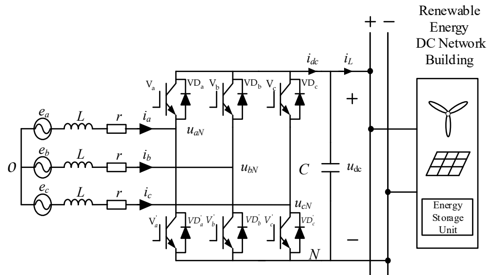
Figure 2. Grid-connected converter topology.
