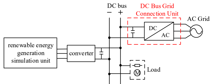
Figure 22. Diagram of the experimental system.
