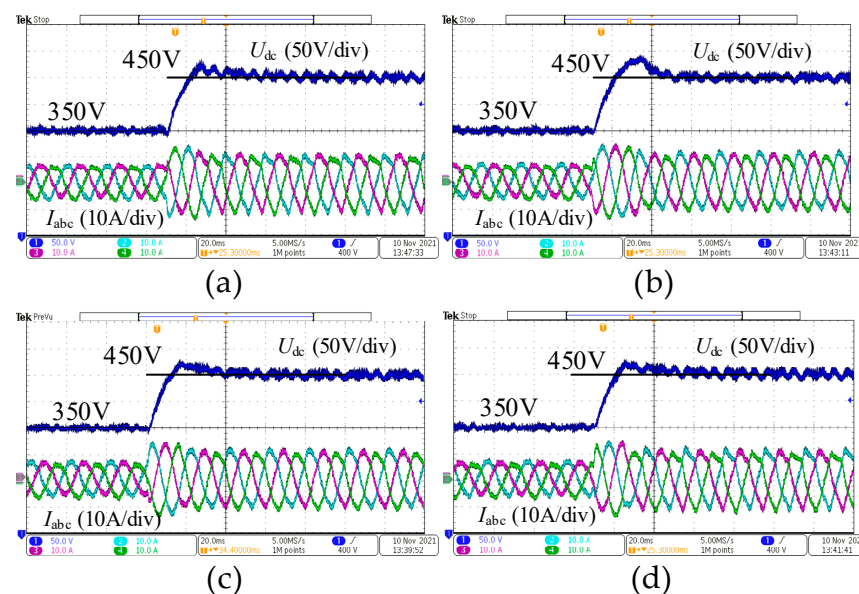
Figure 24. The voltage step response of changing PI parameters: (a) The voltage step response of increasing proportional coefficient; (b) the voltage step response of increasing integral coefficient; (c) the voltage step response of decreasing proportional coefficient; (d) the voltage step response of decreasing integral coefficient.
