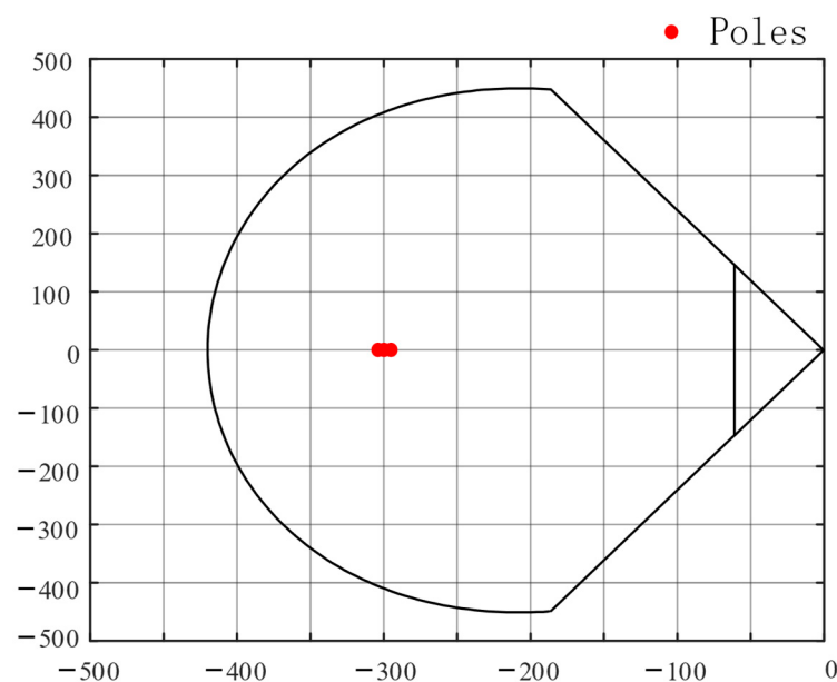
Figure 11. Pole placement area.
