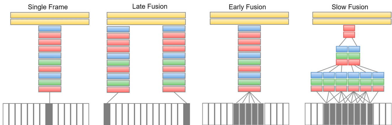
Figure 5. Different strategies for video classification tasks: single-frame, late-fusion, early-fusion, and slow-fusion neural networks.
