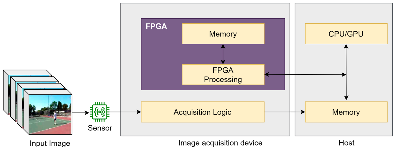
Figure 7. Image processing using FPGA.
