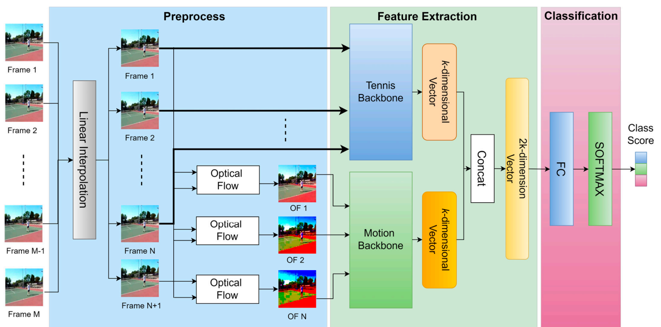
Figure 9. The architecture of the transformer model for extracting frames from a video.
