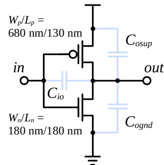
Figure 5. Architecture of each stage of the ring oscillator. The values of the equivalent capacitances are fitted separately for each supply voltage value.
