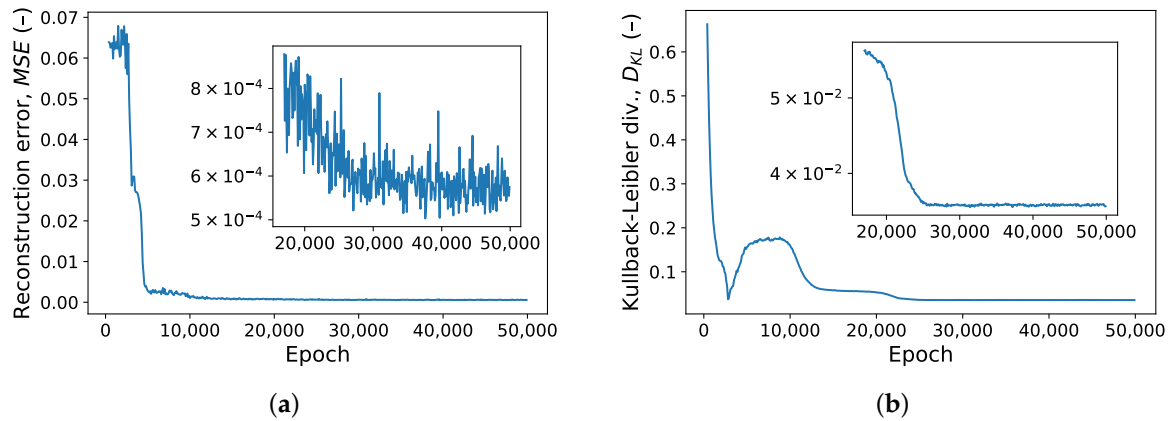
Figure 6. (a) VAE reconstruction error and (b) Kullback–Leibler divergence (KLD) on the validation dataset evaluated in the training phase every 100 epochs. The insets show that the KLD saturates after approximately 20,000 epochs, while the reconstruction error takes approximately twice as long to reach its minimum.
