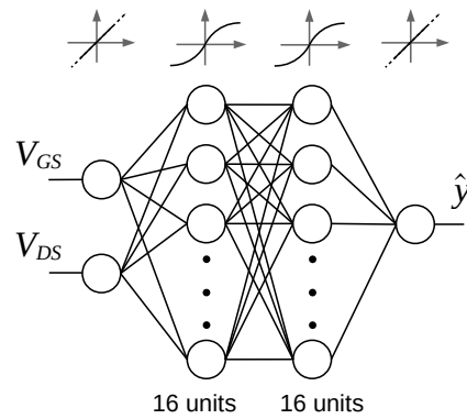
Figure 8. Architecture of the fully-connected ANN used to model individual devices. Also shown are the activation functions of all the layers and the sizes of hidden layers.
