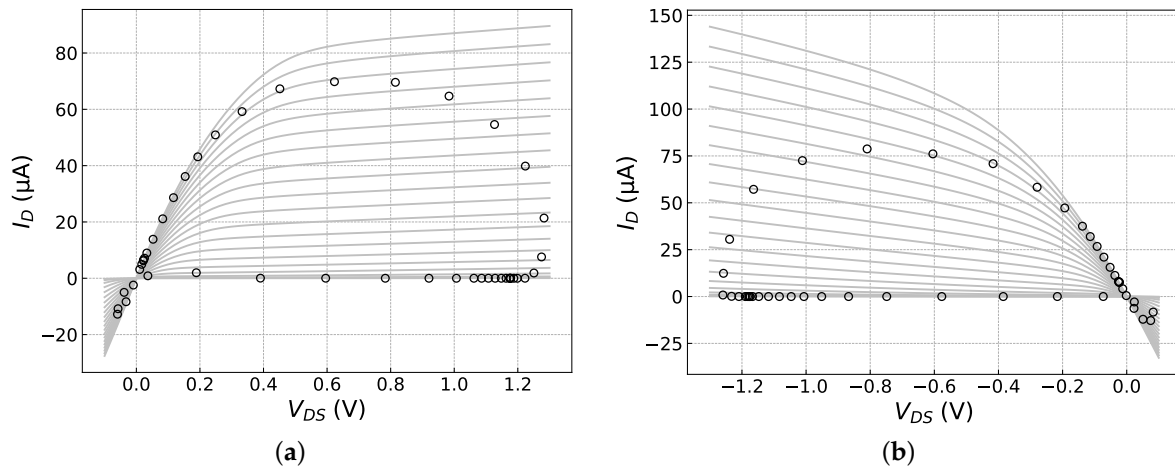
Figure 4. The circles represent (I_D, V_{DS}) samples collected at 5 ps intervals during a single oscillation period from one n-channel and one p-channel MOSFET (Figures (a) and (b), respectively), plotted against the respective device’s output curves. The top curve corresponds to |V_{GS}| = 1.2 V (oscillator supply voltage); the spacing between curves is \Delta V_{GS} = 50 mV.
