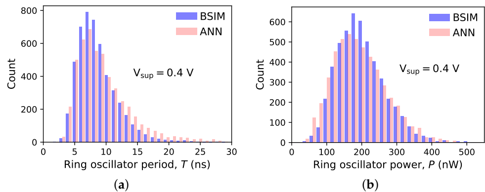
Figure 10. Histograms of the (a) period and (b) power consumption of 5000 ring oscillators with devices operating in moderate inversion ( V_{sup} = 0.4 V). The ANN-based device models were generated by VAEs trained using 50 instances per device type. BSIM results serve as a reference.
