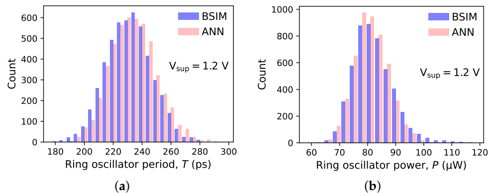
Figure 9. Histograms of (a) period and (b) power consumption of 5000 ring oscillators described in Section 3.1. The ANN-based device models were generated by VAEs trained using 50 instances per device type. BSIM results serve as a reference.
