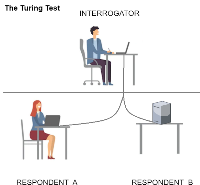
Figure 1. Turing test.
