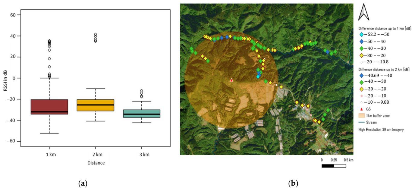
Figure 5. Comparison between measurement data and theoretical data: (a) difference between distance up to 1, 2, and 3 km; (b) Difference of received signal strength on the map.
