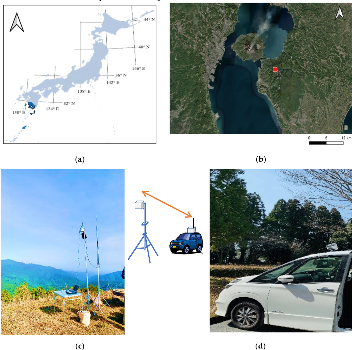
Figure 2. Experimental setup: (a) Map of Japan; (b) Experimental area; (c) Ground station located at Mt. Takatouge; (d) Transmitting station mounted on the roof of vehicle.
