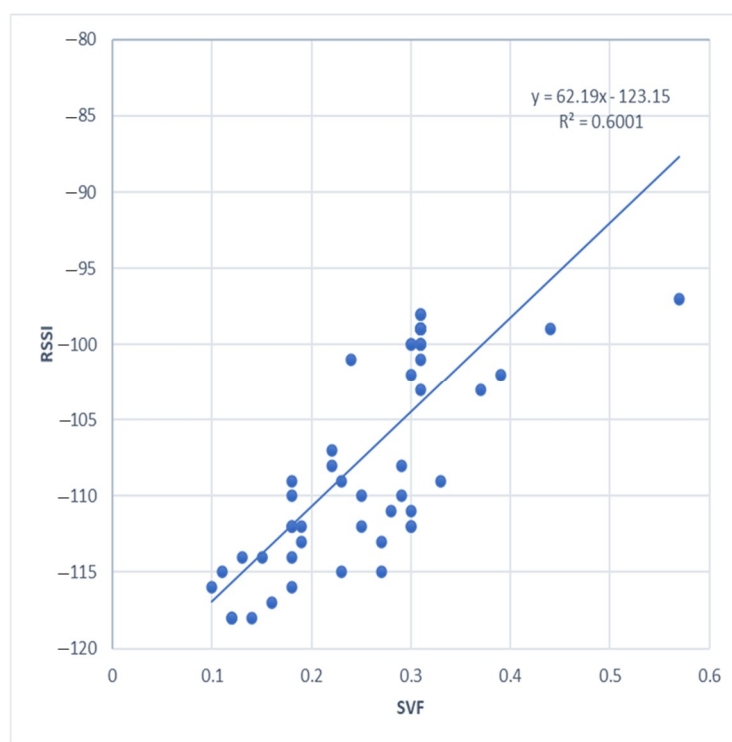
Figure 6. Correlation analysis between received signal strength indicator (RSSI) and Sky View Factor (SVF).
