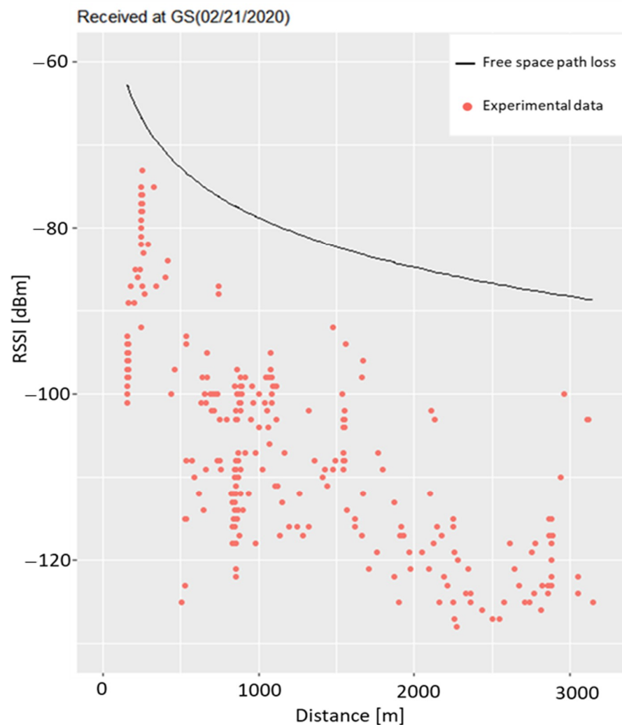
Figure 4. Propagation characteristics of 920 MHz band in distance: Experimental and theoretical data versus distance.
