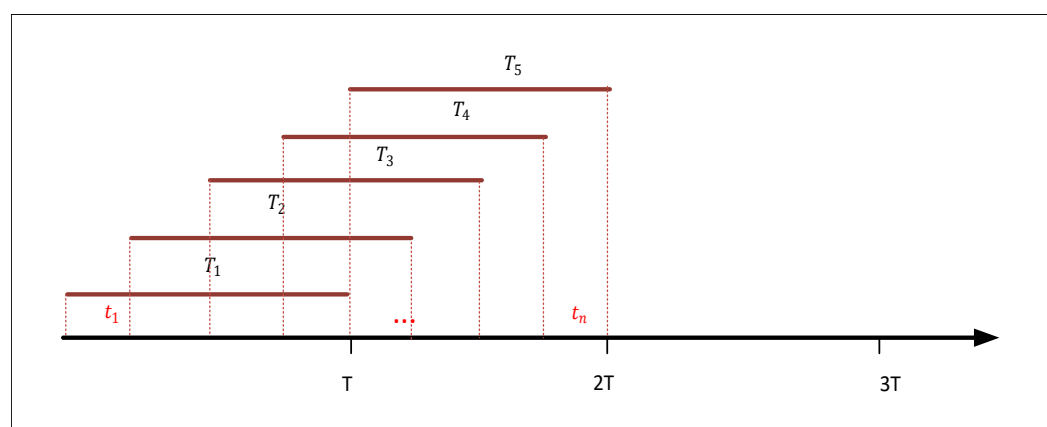
Figure 5. Sliding Time Window Principle.
