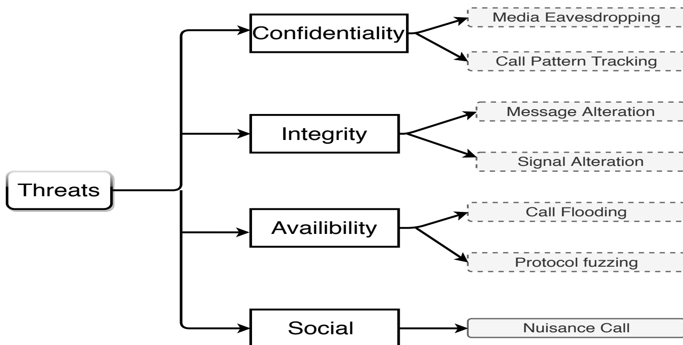
Figure 1. Taxonomy of Internet Telephony Threats.
