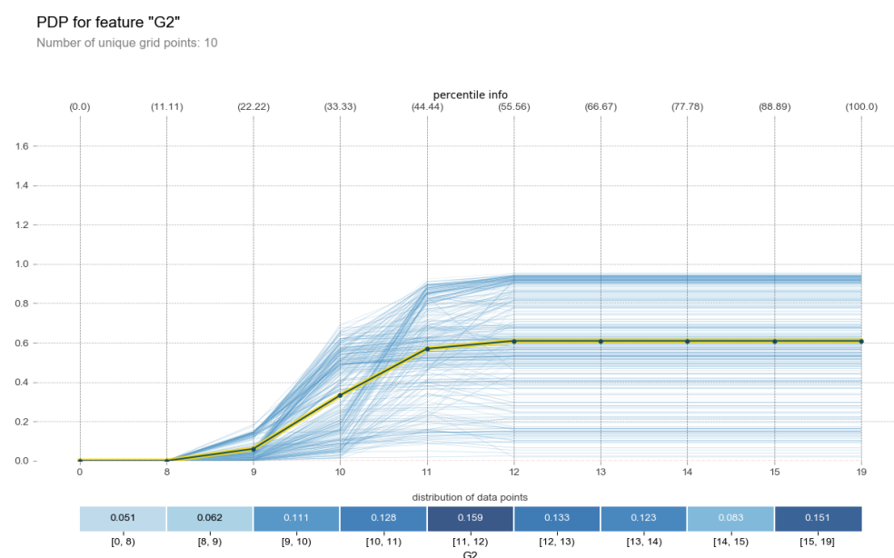
Figure 14. Explanation of the feature G2 for the gradient boosting classifier.
