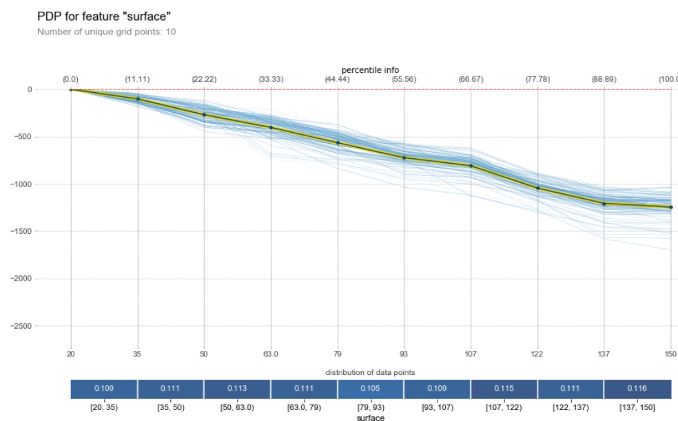
Figure 7. Global explanation of the feature surface for GBR .
