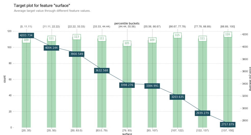
Figure 6. Target distribution for an independent numerical variable surface which shows the overall behavior of price for an average surface.
