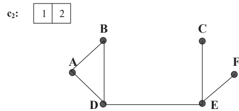
Figure 3. Channel Graph for c_2 .
