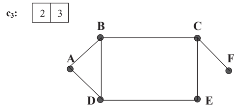
Figure 4. Channel Graph for c_3 .
