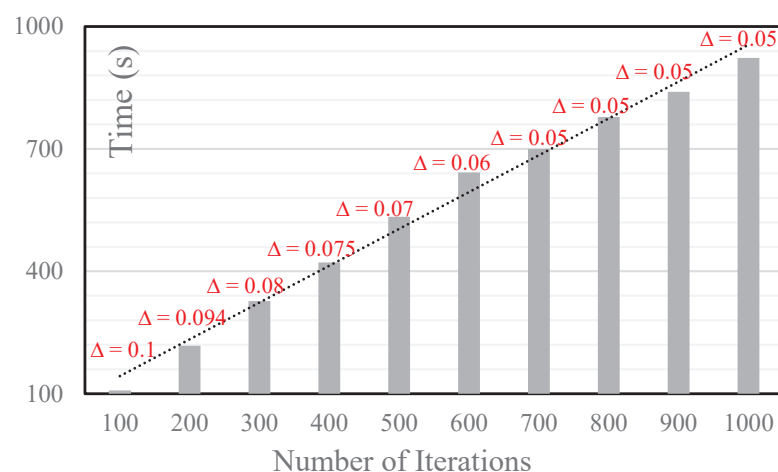
Figure 6. Iteration Number and Computational Time.
