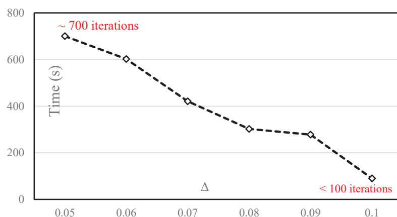
Figure 5. \Delta and Computational Time.
