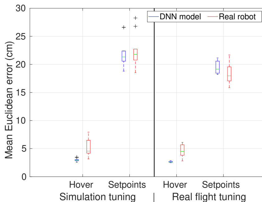
Figure 5. Boxplot of mean Euclidean error obtained by the weight sets having top ten grade values in the lookup tables from simulation (left) and real flight (right) tuning.
