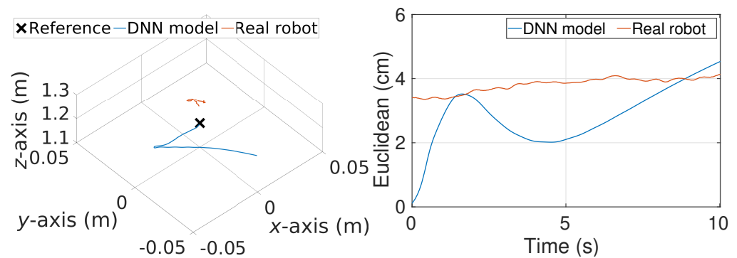
Figure 3. Hovering performance of the weight set obtained from simulation tuning. Left: 3D view of the stationary reference and tracked trajectories. Right: resulting Euclidean error over the DNN model and the real robot.
