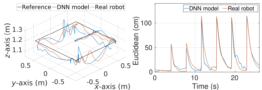
Figure 4. Sequential-setpoints tracking performance of the weight set obtained from simulation tuning. Left: 3D view of the sequential-setpoints and tracked trajectories. Right: resulting Euclidean error over the DNN model and the real robot.
