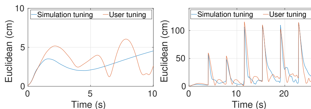
Figure 7. Euclidean errors for hover (left) and for sequential setpoints (right) by the best weight sets from simulation and user-based tuning.
