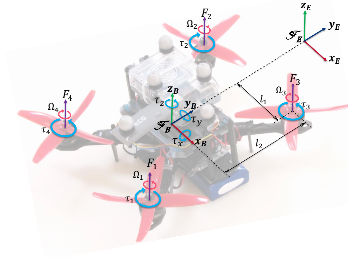
Figure 1. Custom-made quadrotor of interest. Notation: F_i and \tau_i are the force and torque generated by i^{\text{th}} rotor with \Omega_i angular velocity; \tau_x, \tau_y, \tau_z are the external moments about x -, y -, z -axes, respectively.
