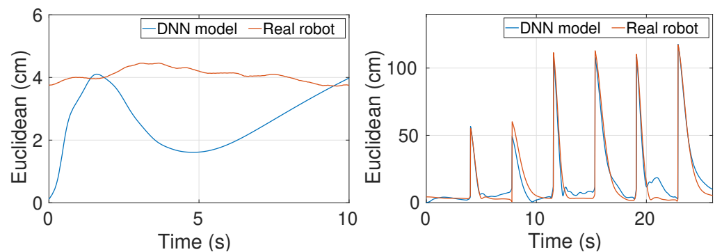
Figure 6. Euclidean errors for hover (left) and for sequential-setpoints (right) by the weight set from real flight tuning.
