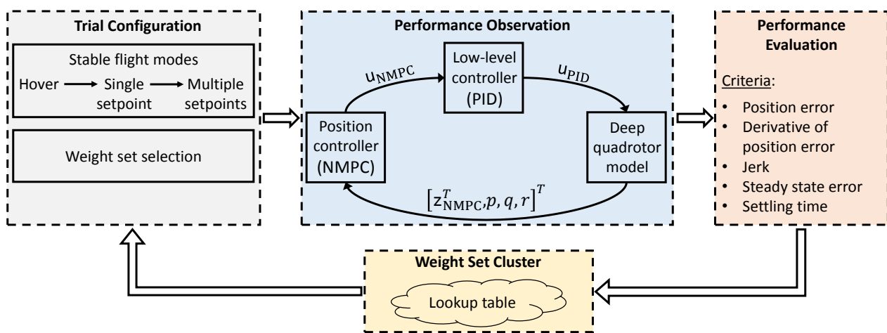
Figure 2. Proposed (N)MPC weight tuning framework. Throughout the tuning process, each trial starts with the Trial Configuration module. Weight set selection and Stable flight mode submodules give necessary instructions to (N)MPC. Taking these as inputs, (N)MPC controls the quadrotor model while its performance is being observed simultaneously. Once a flight is completed, the performance of the (N)MPC with the utilized weight set is graded based on the five criteria. Subsequently, the trial is finalized by updating the weight set cluster. Thereafter, a new trial begins with the selection of a new weight set within the Trial Configuration module, and thus closes the loop.
