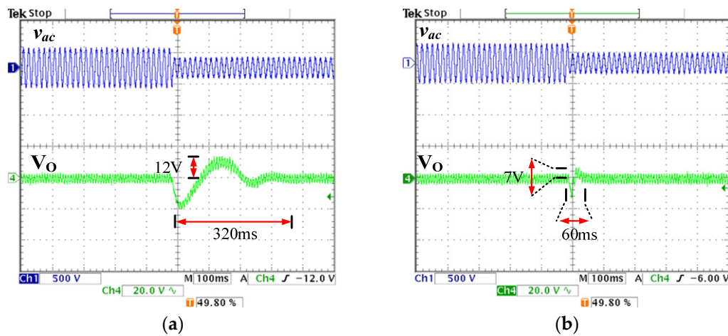
Figure 11. Transient response waveform of an input voltage change from 220 to 110 V_{rms} based on PFC with the use of (a) the conventional control strategy and (b) the new control strategy ( V_{ac} : 500 V/div., v_o : 20 V/div., time: 100 ms/div.).
