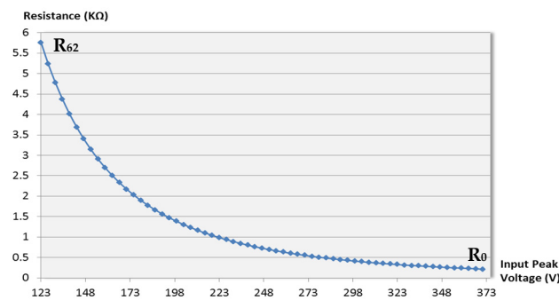
Figure 7. Resistance corresponding to various input voltage peaks.
