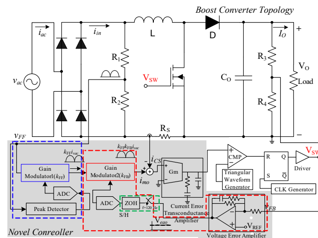
Figure 3. Proposed PFC control circuit block.
