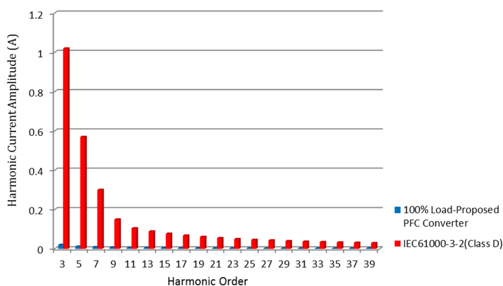
Figure 13. Comparison of current harmonic between the proposed structure and the standard of IEC61000-3-2 (Class-D) under the input voltage 110 V and output power 300 W.
