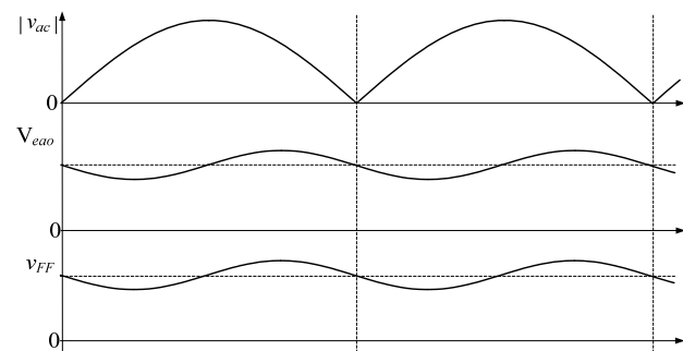
Figure 2. Crucial command waveform.
