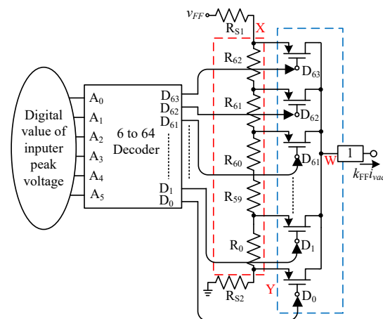
Figure 5. The proposed feedforward loop circuit scheme.
