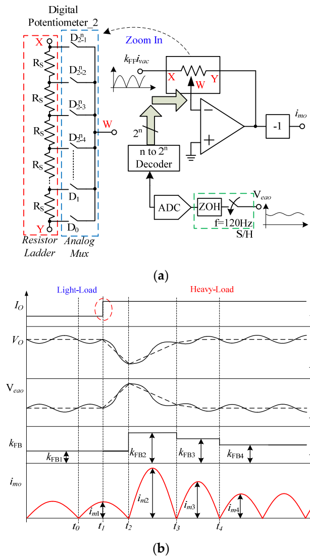
Figure 6. (a) The proposed new control strategy-based voltage feedback loop control circuit scheme; (b) relevant critical waveforms.
