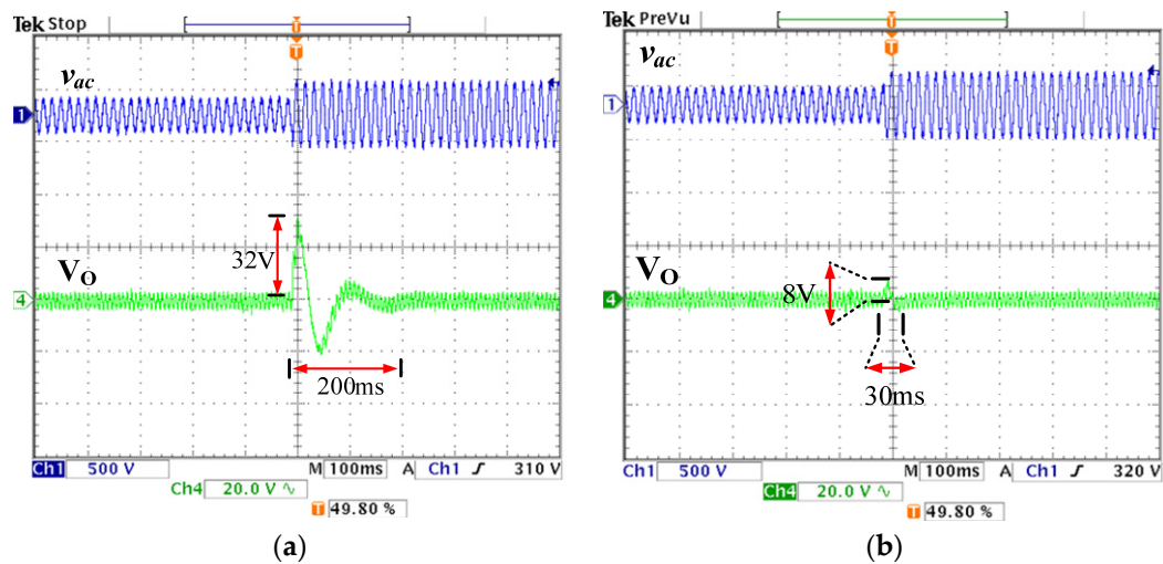
Figure 10. Transient response waveform of an input voltage change from 110 to 220 V_{rms} based on PFC with the use of (a) the conventional control strategy and (b) the new control strategy ( V_{ac} : 500 V/div., v_o : 20 V/div., time: 100 ms/div.).
