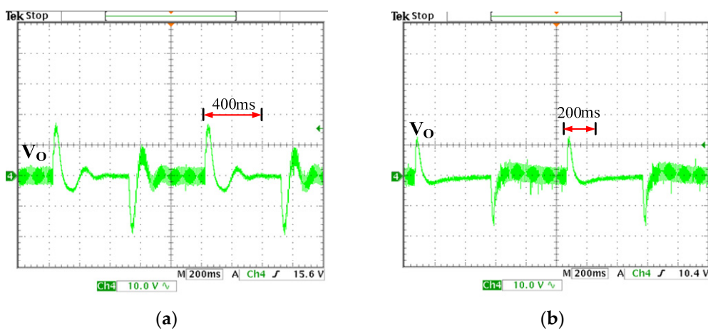
Figure 12. Output transient response waveform based on PFC with the use of (a) the conventional control strategy and (b) the new control strategy ( V_{ac} : 500 V/div., v_o : 10 V/div., time: 200 ms/div.).
