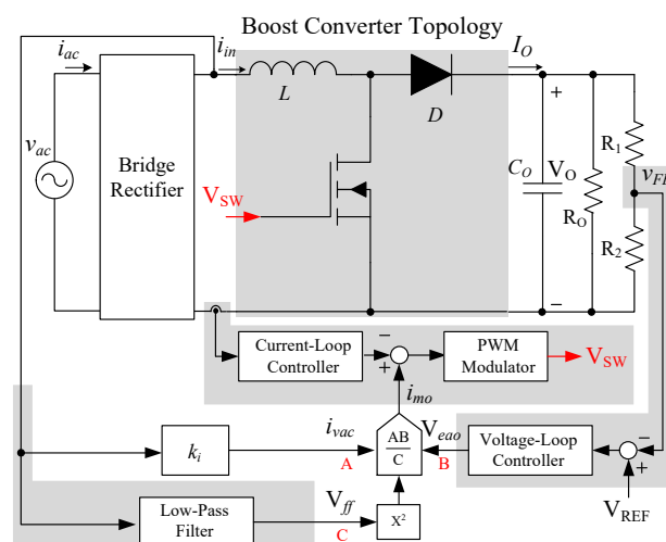
Figure 1. PFC regulators control scheme operating in the average current mode.
