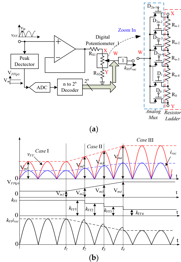
Figure 4. (a) The proposed novel feedforward loop control circuit scheme; (b) relevant key waveforms.
