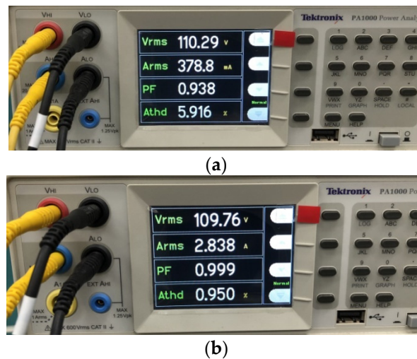
Figure 9. At an input voltage of 110 V rms , the boost PFC input line current THDi with (a) output power of 40 W and (b) output power of 300 W.
