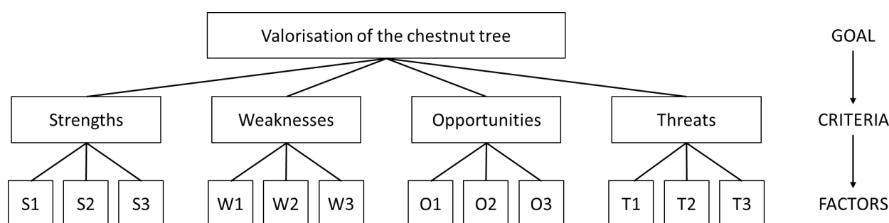
Figure 1. AHP structure.
