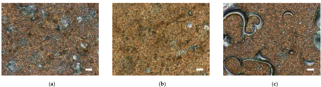
Figure 12. CLSM images of PAN:PEO samples after stabilization with a PAN:PEO ratio of 9:1 and PEO molecular weights of (a) 40 kDa; (b) 600 kDa; (c) 1000 kDa. Scale bars correspond to 1 \mu m.
