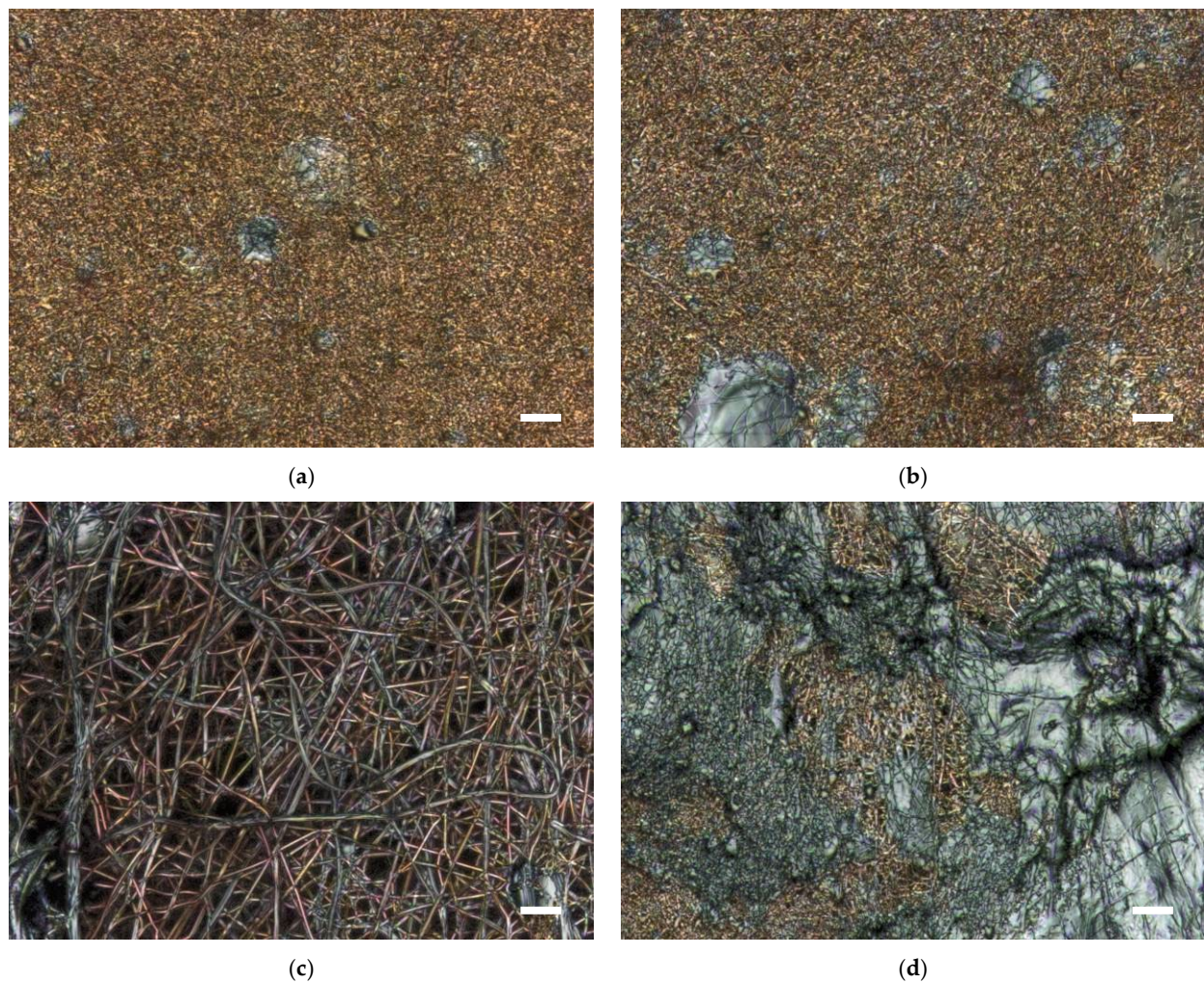
Figure 11. CLSM images of PAN:PEO samples after stabilization with a PAN:PEO ratio of (a) 9:1; (b) 8:2; (c) 7:3; (d) 6:4 and PEO 300 kDa. Scale bars correspond to 1 \mu m.
