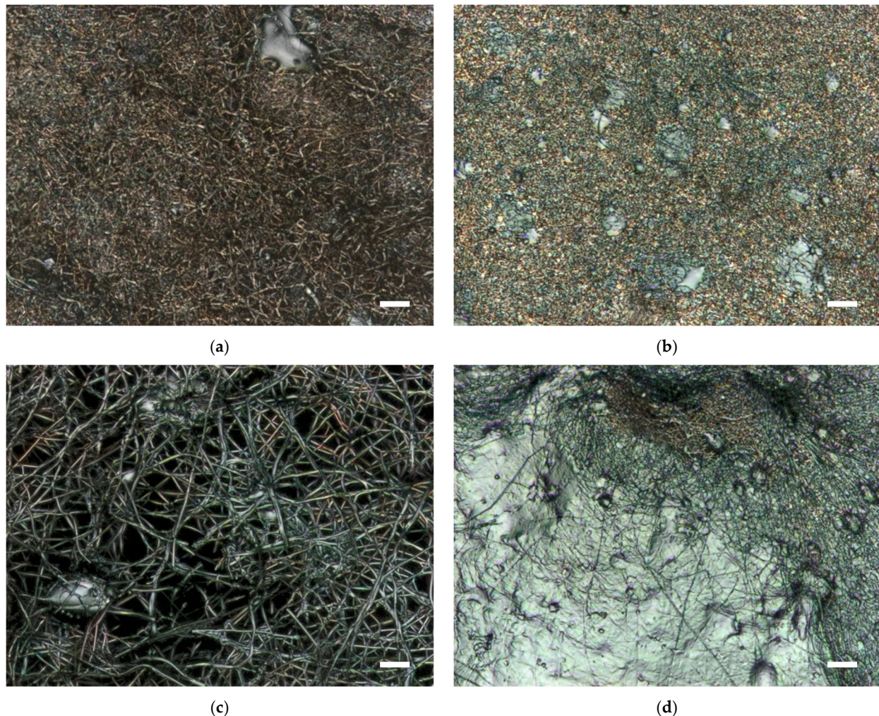
Figure 13. CLSM images of PAN:PEO samples after carbonization with a PAN:PEO ratio of (a) 9:1; (b) 8:2; (c) 7:3; (d) 6:4 and PEO 300 kDa. Scale bars correspond to 1 \mu m .
