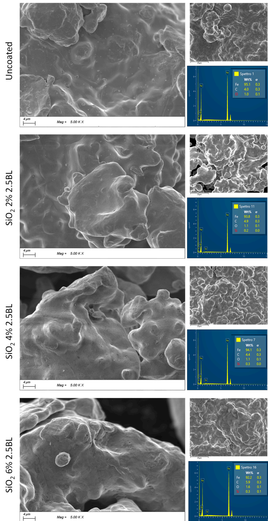
Figure 7. Microstructure analysis at 5000× and EDS measurements of uncoated and 2.5 BL (SiO 2 2%, 4% and 6%) coated iron powder.
