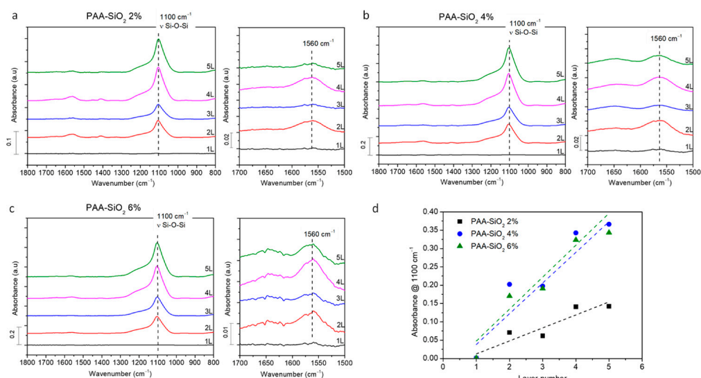
Figure 6. Coating growth on model silicon substrate: IR spectra at different deposited layers (plus additional magnified range graph) for PAA-SiO 2 2% (a), PAA-SiO 2 4% (b), PAA-SiO 2 6% (c) and absorbance of the signal at 1100 cm −1 vs. number of deposited layers (d).
