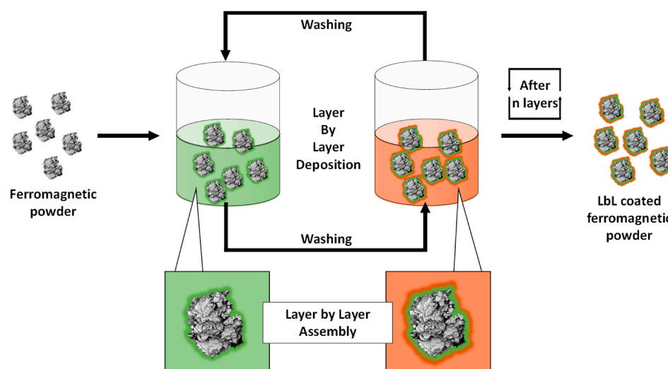
Figure 1. Layer-by-layer deposition process on iron powders.
