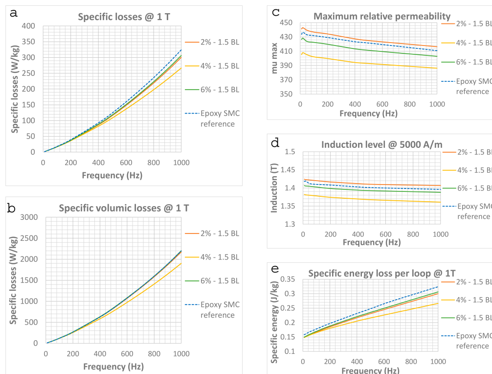
Figure 8. Magnetic and energetic comparison as a function of the variation in the SiO 2 with coating obtained with 1.5 BL (3 layers): Specific iron loss @ 1 T as a function of frequency related to weight (a) and volume (b); maximum relative magnetic permeability as a function of frequency (c); magnetic induction @ 5000 A/m as a function of frequency (d) and specific energy @ 1 T as a function of frequency (e).
