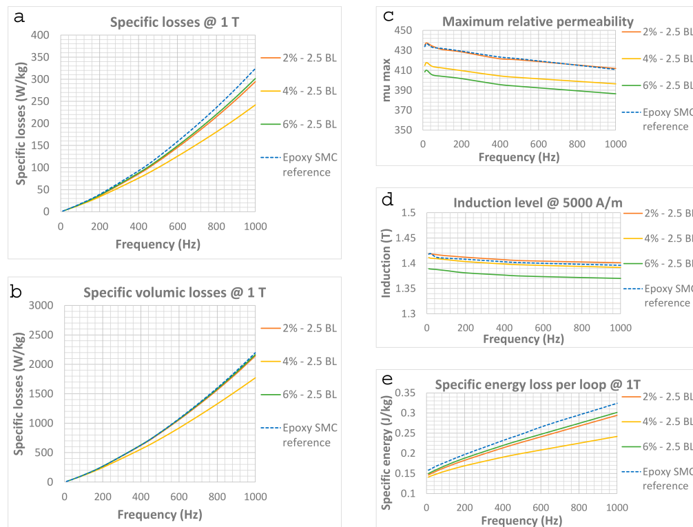
Figure 9. Magnetic and energetic comparison as a function of the variation in the SiO 2 with coating obtained with 2.5 BL (5 layers): Specific iron loss @ 1 T as a function of frequency related to weight (a) and volume (b); maximum relative magnetic permeability as a function of frequency (c); magnetic induction @ 5000 A/m as a function of frequency (d) and specific energy @ 1 T as a function of frequency (e).
