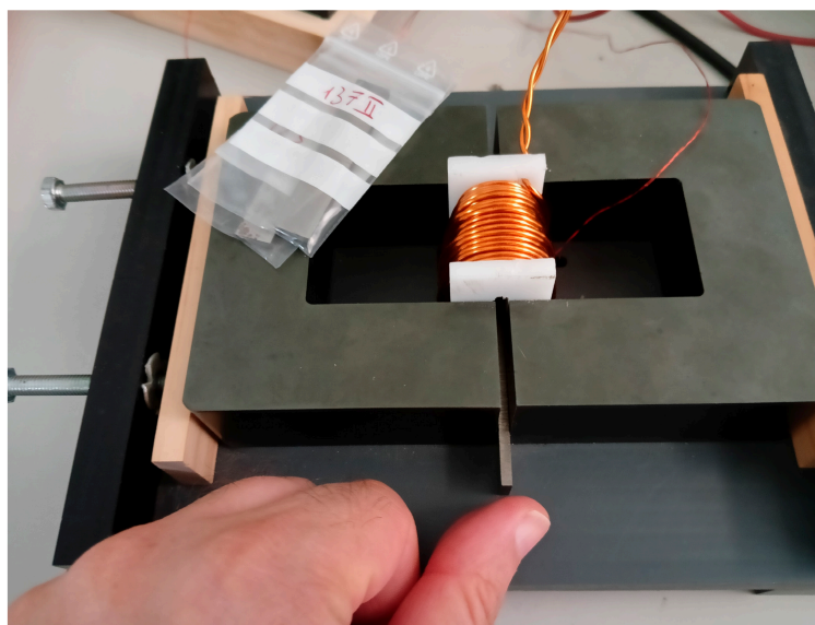
Figure 4. Single-sheet tester with the BPEI/SiO 2 SMC samples under examination.
