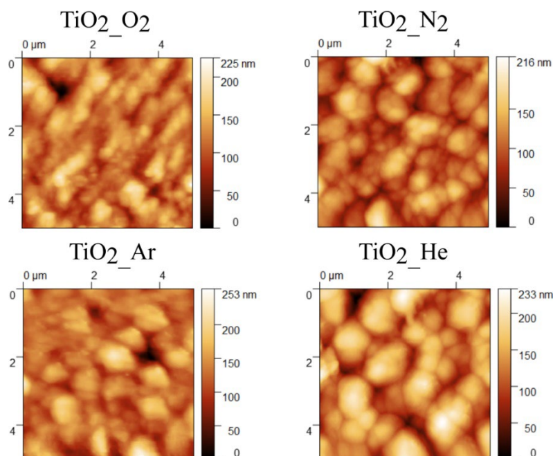
Figure 3. Typical AFM micrographs ( 5 \times 5 \mu\text{m}^2 investigation area) of the coatings deposited by PLD under different gas environments ( \text{O}_2 , \text{N}_2 , Ar, and He).
