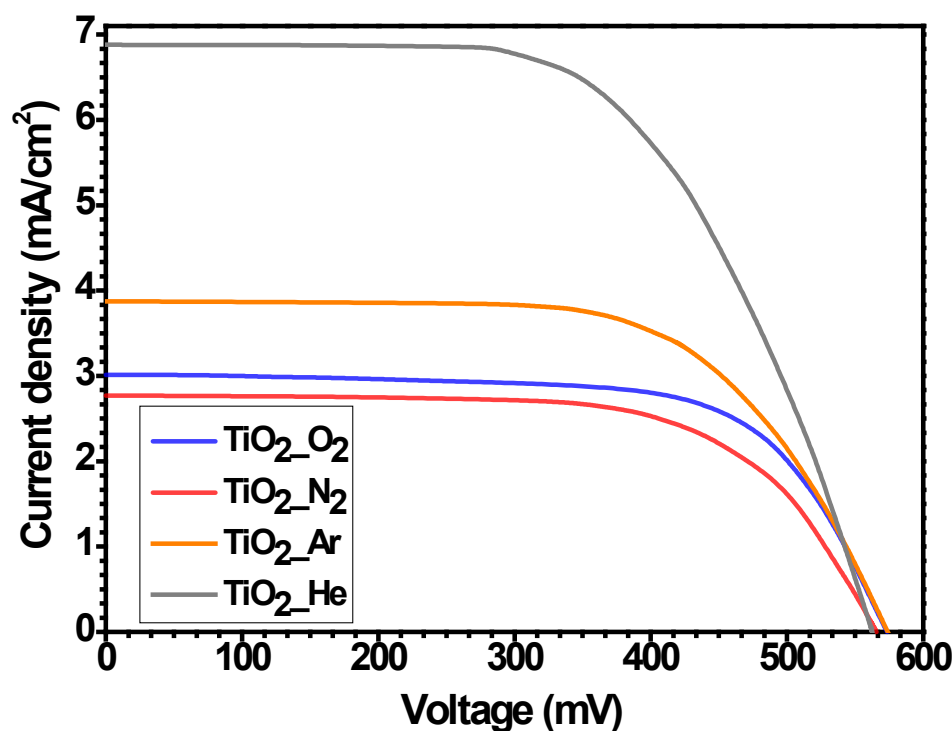
Figure 5. Current–voltage curves for typical dye-sensitized solar cells fabricated using photoelectrodes with various coatings: TiO 2 -O 2 (blue line); TiO 2 -N 2 (red line); TiO 2 -Ar (orange line); and TiO 2 -He (grey line). The measurements were carried out under standard AM 1.5G illumination conditions.
