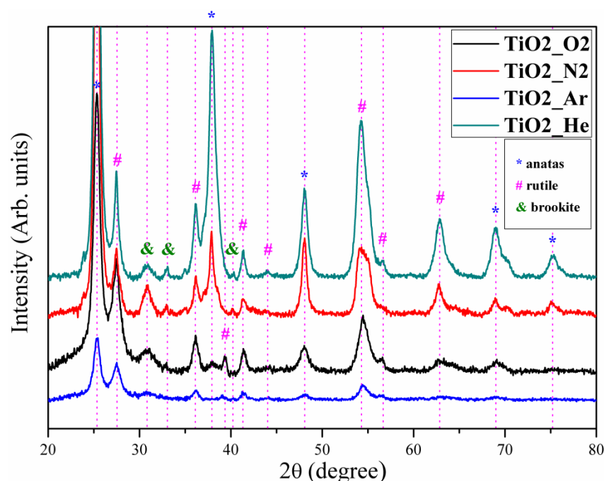
Figure 4. XRD patterns of TiO 2 coatings deposited by PLD in different ambient gases (O 2 , N 2 , Ar, or He).
