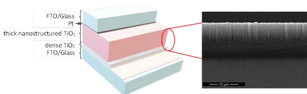
Figure 1. Schematic design of the solar cell (left); and cross-section SEM image of the \text{TiO}_2 coating (right).
