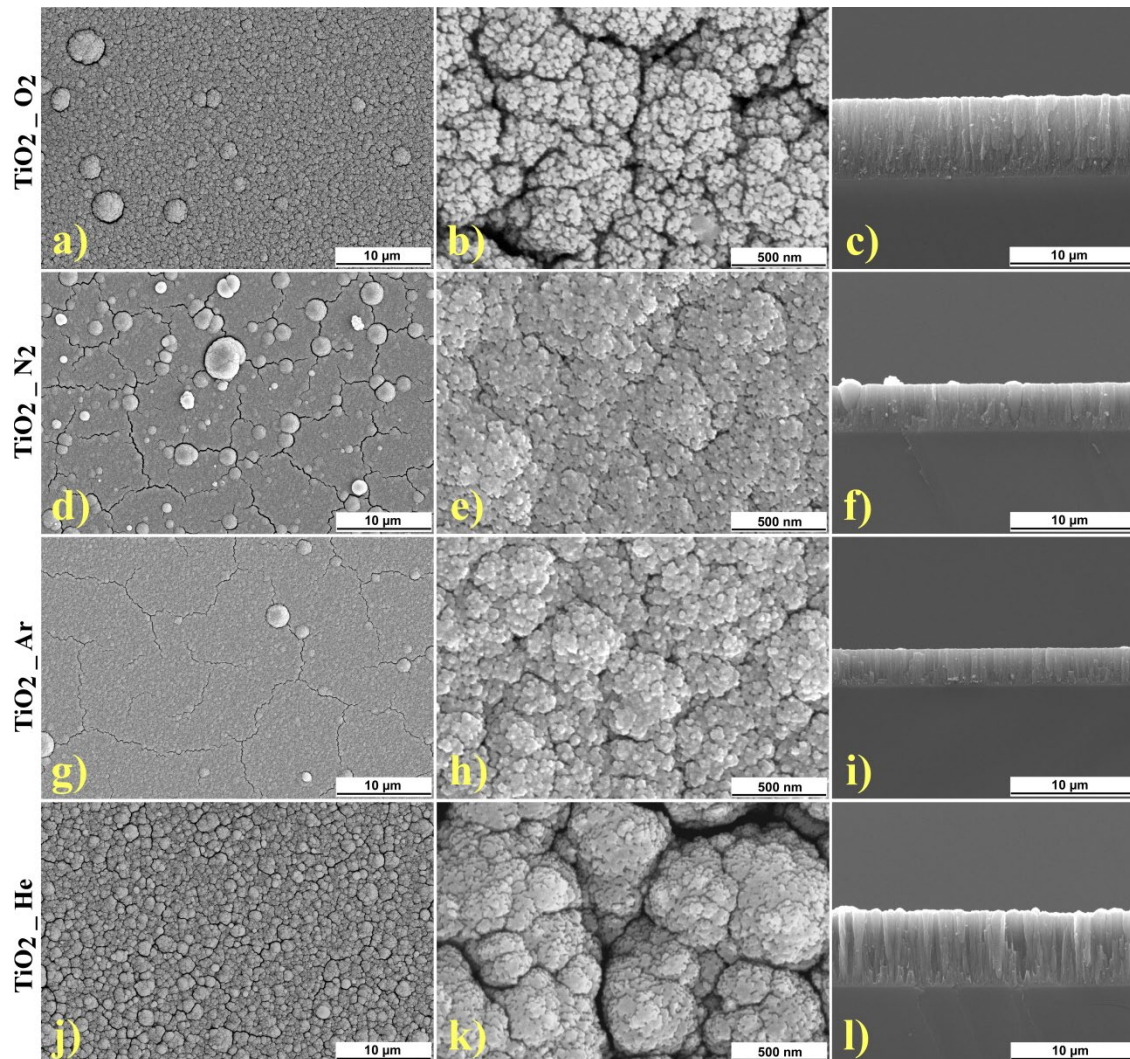
Figure 2. Typical top-view images of (a,d,g,j) low magnification, and (b,e,h,k) high-magnification, and (c,f,i,l) cross-section SEM micrographs of the thick nanostructured films deposited under various atmospheres (O 2 , N 2 , Ar, or He).
