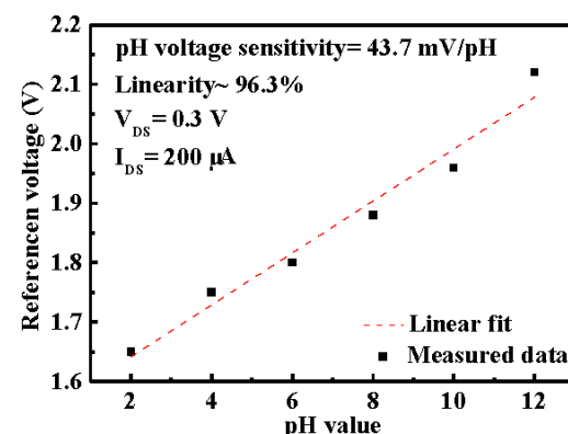
Figure 8. Reference voltage ( V_{\text{REF}} ) as a function of pH value.
