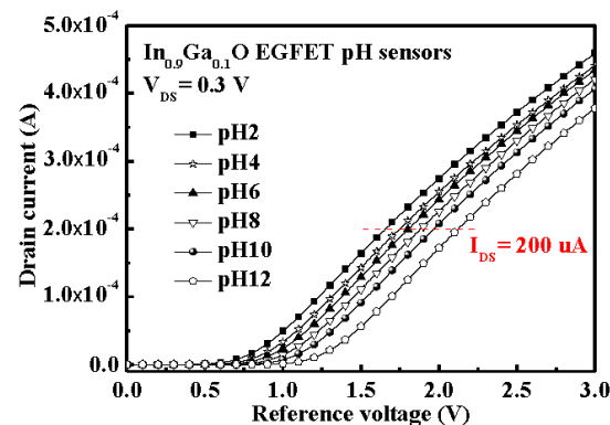
Figure 7. The transfer characteristic curves ( I_{\text{DS}}-V_{\text{REF}} ) characteristics of the \text{In}_{0.9}\text{Ga}_{0.1}\text{O} EGFET pH sensors.
