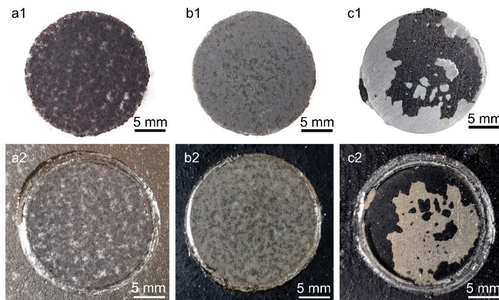
Figure 6. Fracture surface morphologies of (a) RS, (b) RS coated with RCC, (c) BS coated with RCC: (1) spindle, (2) substrate (RS: rusted steel, BS: bare steel, RCC: rust conversion coating).
