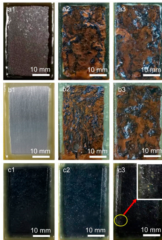
Figure 5. The surface state of the steel plates before and after rust conversion treatment under salt spray test on 1d (a1,b1,c1)—7d (a2,b2,c2)—20d (a3,b3,c3): (a1–a3) Rusty steel with AR, (b1–b3) Bare steel, (c1–c3) RCC.
