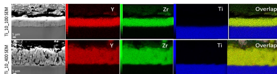
Figure 6. Distributions of map elements for deposited coatings. Scale bar = 1 µm.
