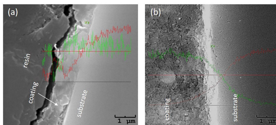
Figure 7. Linear analysis of the distribution of elements for obtained coatings. Scale bar = 1 µm; (a) Ti_10_100; (b) Ti_10_400.
