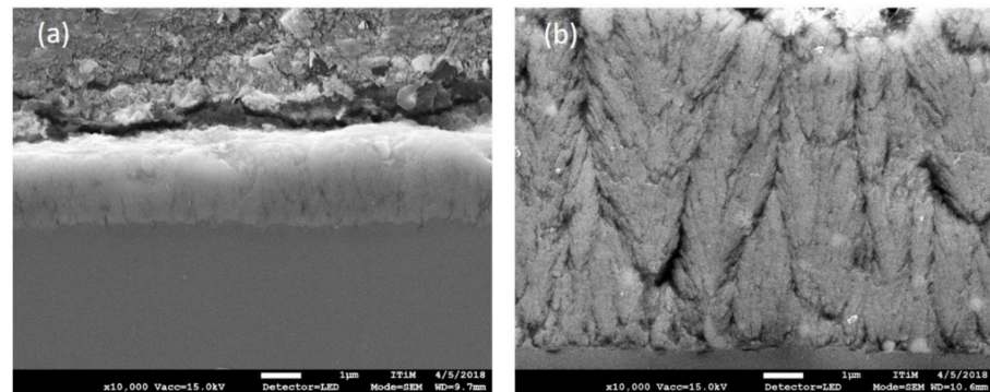
Figure 1. Characteristic columnar structure observed by high-resolution SEM. Scale bar = 1 µm; (a) Ti_10_100; (b) Ti_10_400.
