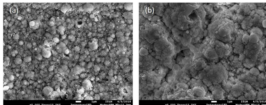
Figure 2. Top-view HR-SEM images for obtained coatings. Scale bar = 1 µm; (a) Ti_10_100; (b) Ti_10_400.
