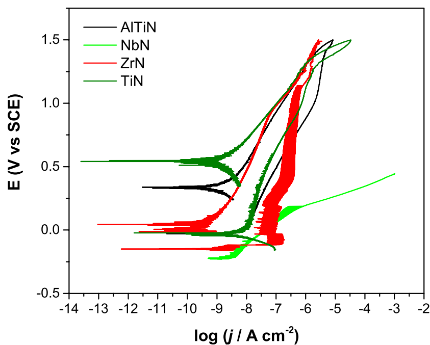
Figure 2. Anodic polarization curves relative to all the investigated coatings performed in 0.1 M \text{Na}_2\text{SO}_4 (pH 5.5). Scan rate of 0.17 \text{ mV s}^{-1} , equilibration time of 5 min and reverse current of 2 \text{ mA/cm}^2 .
