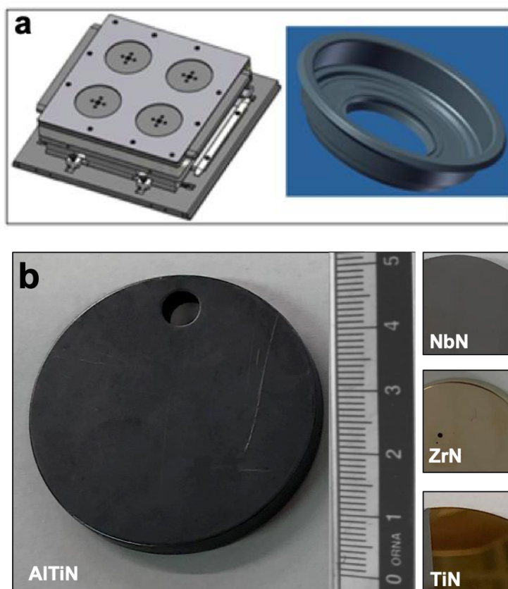
Figure 1. (a) Mould apparatus and moulded seal; (b) PVD coated-substrates samples.
