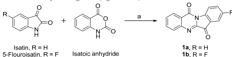
Scheme 1. Synthetic route for the preparation of tryptanthrins. Reagents and conditions: (a) triethylamine, toluene, 110 °C, 4 h, 90%.
