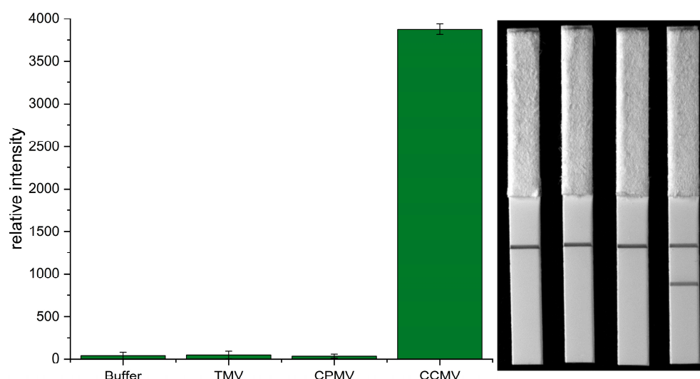
Figure 5. Determination of assay selectivity. Running buffer was spiked with 2000 µg/L of TMV, CPMV, and CCMV, respectively. (Left): Quantitative evaluation of relative line intensities. Error bars were calculated as the relative standard deviation of duplicate measurements. (Right): representative test strips corresponding to the tested samples.
