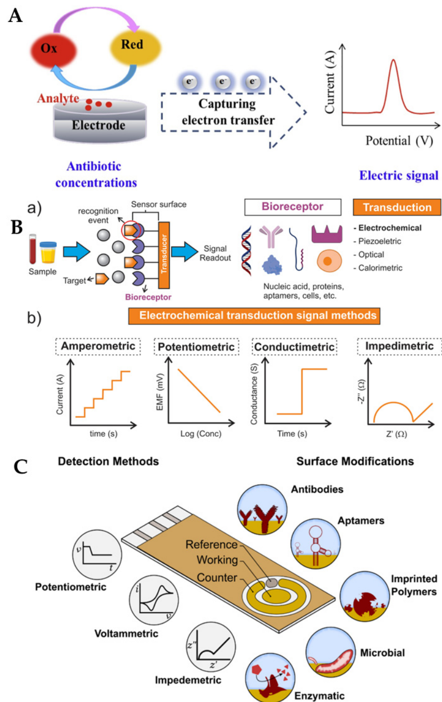
Figure 3. (A) Principle of electrochemical sensors (electrode) for the detection of antibiotics [68]. Reprinted from Ref. [68], Copyright (2021), with permission from Elsevier. (B(a)) Schematic of a generic biosensor device. A sample containing the target (analyte) is placed in close contact with the surface of the sensor. The bioreceptor (antibody, lectin, enzyme, aptamer, DNA, or cells), which is immobilised above the transducer (electrochemical, piezoelectric, optical, calorimetric modes, etc.), binds with the target from the sample (recognition event), after which the transducer converts the binding event into a measurable signal that is proportional to the concentration of the target (signal readout). (b) Examples of electrochemical transduction signals encompass amperometric, potentiometric, conductimetric, and impedimetric signals [69]. Reprinted from Ref. [69], Copyright (2022), with permission from Elsevier. (C) Electrochemical detection, in which the working, reference and counter electrodes are arranged in a manner allowing the sample to be in contact with all three at the same time. The range of possible surface modifications on the working electrode are shown [70]. Reproduced under the terms of the CC-BY licence from Ref. [70], Copyright 2021, The Authors, published by MDPI.
