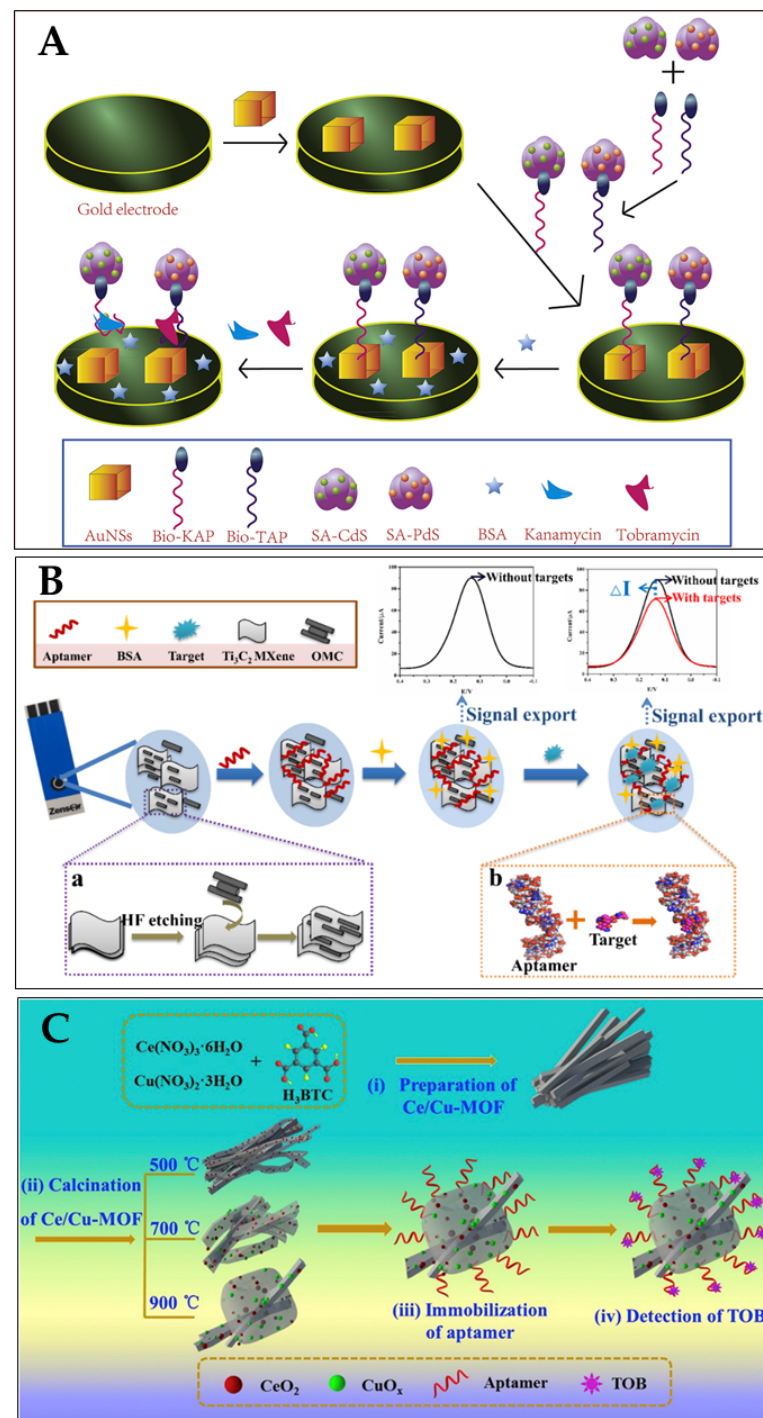
Figure 13. (A) Schematic illustration of aptasensor based on the utilisation of QDs, AuNSs, RNA-based aptamer strands, and high-affinity pairing between Bio and SA for the simultaneous detection of multiple antibiotics [119]. Reprinted from Ref. [119], Copyright (2021), with permission from Elsevier. (B) Schematic aptasensor fabrication process: (a) formation process of OMC@ \text{Ti}_3\text{C}_2 MXene; (b) binding mode of aptamer with target [120]. Reproduced under the terms of the CC-BY licence from Ref. [120], Copyright 2022, The Authors, published by MDPI. (C) Schematic diagram of the fabrication procedure of the \text{CeO}_2/\text{CuO}_x/\text{mC} -based aptasensor for detecting TOB, including (i,ii) the preparation of the series of \text{CeO}_2/\text{CuO}_x/\text{mC} nanocomposites, (iii) the immobilisation of the aptamer strands over the \text{CeO}_2/\text{CuO}_x/\text{mC} composite, and (iv) TOB detection using the proposed \text{CeO}_2/\text{CuO}_x/\text{mC} -based aptasensor [121]. Reprinted from Ref. [121], Copyright (2019), with permission from Elsevier.
