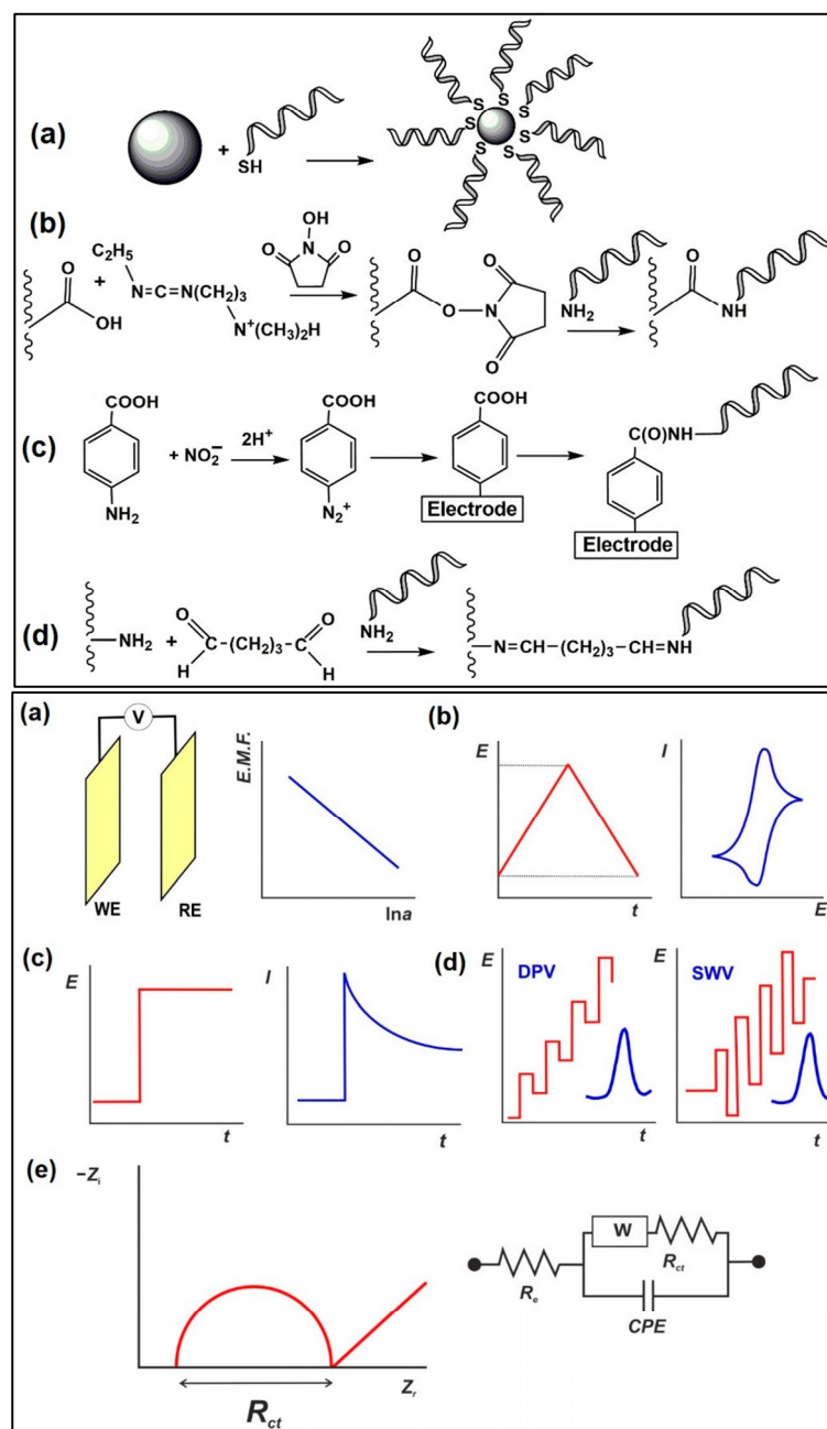
Figure 11. (Top) Immobilisation protocols applied in electrochemical aptasensors: (a) interaction of thiolated aptamer with AuNPs/bare Au electrode; (b) carbodiimide binding to carboxylated support; (c) electrografting with diazonium salt generated from aromatic amino group; (d) glutaraldehyde cross-binding of aminated aptamer and carrier. (Bottom) Electrochemical sensors used as transducers of aptasensors: (a) potentiometric cell: WE—working electrode, RE—reference electrode, V—voltmeter; (b) cyclic voltammetry; (c) amperometry; (d) differential pulse voltammetry (DPV) and square wave voltammetry (SWV). The red line illustrates the shape of the current peak obtained; (e) electrochemical impedance spectroscopy; the Nyquist diagram and equivalent circuit correspond to the double-electric layer. R_e is electrolyte resistance, R_{ct} is charge transfer resistance, W is Warburg impedance, and CPE is the constant phase element [111]. Reproduced under the terms of the CC-BY licence from Ref. [111] [Sensors], Copyright 2022, The Authors, published by MDPI.
