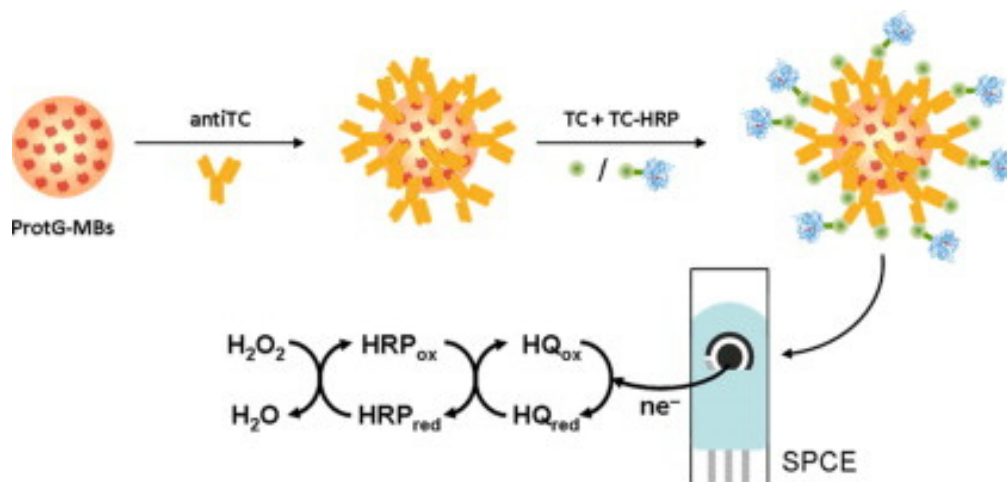
Figure 6. Graphical representation/abstract of the disposable amperometric magneto-immunosensor for the direct detection of tetracycline antibiotic residues in milk [95]. Reprinted from Ref. [95], Copyright (2012), with permission from Elsevier.
