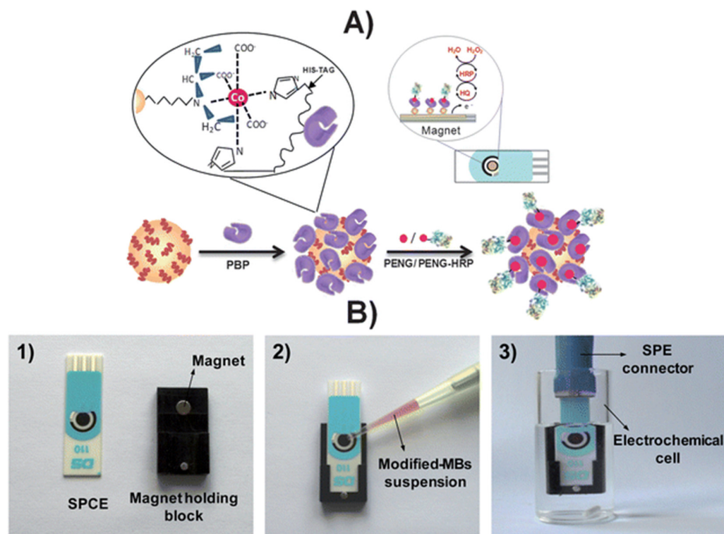
Figure 10. (A) Schematic display of the steps involved in the affinity magnetosensor developed for \beta -lactam antibiotics. (B) Picture showing the SPCE and the home-made magnet holding block (1), the deposition of the modified MBs on the SPCE assembled on the magnet holding block (2) and the assembled SPCE-magnet holding block immersed in the electrochemical cell used for the amperometric measurements (3) [100]. Reproduced from Ref. [100], Copyright (2013), with permission from the Royal Society of Chemistry.
