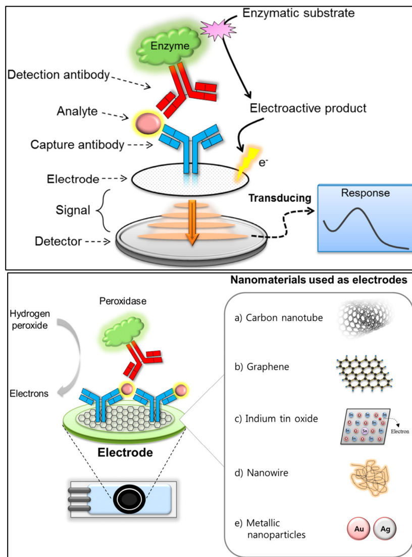
Figure 5. (Top) Basic analytical principle of electrochemical immunosensors. (Bottom) Nanomaterials used as electrodes or supporting solid matrices to enhance the analytical performance of electrochemical immunosensing [84]. Reproduced under the terms of the CC-BY licence from Ref. [84], Copyright 2018, The Authors, published by MDPI.
