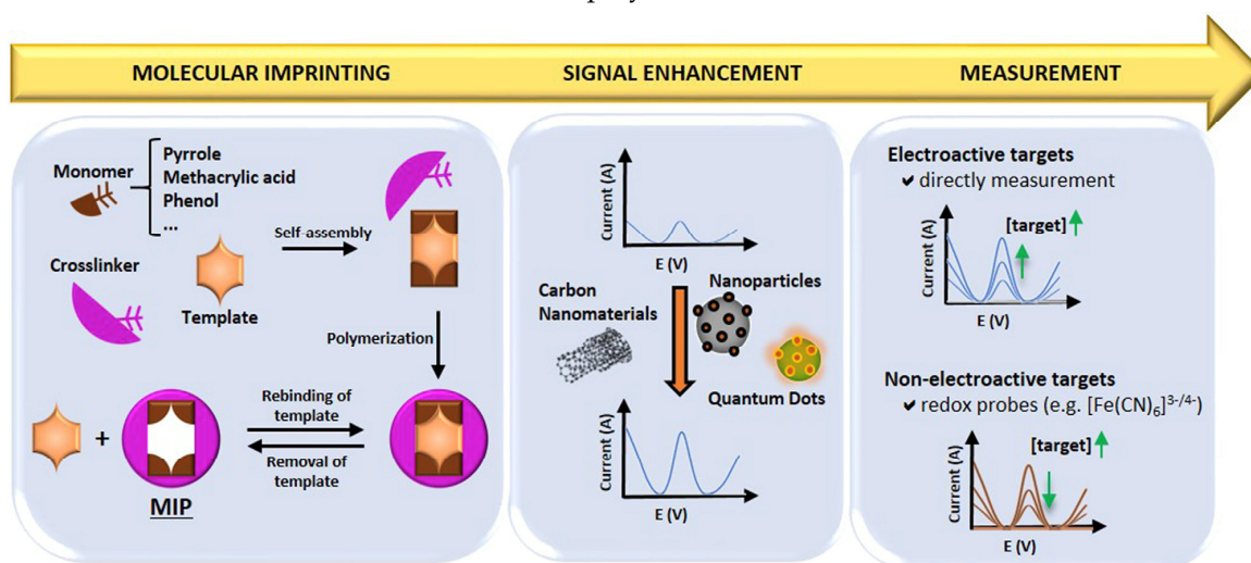
Figure 14. Summary of the preparation procedure, signal enhancement and sensing mechanism for MIPs in MIP-based electrochemical sensors [133]. Reprinted from Ref. [133], Copyright (2021), with permission from Elsevier.
