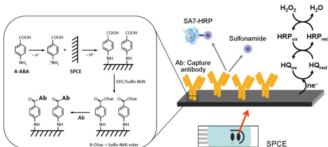
Figure 7. Schematic display of the immunosensor developed for the detection of sulfonamide antibiotics (inset: details of the surface chemistry involved in the covalent immobilisation of the capture antibody by using EDC and Sulfo-NHS 4-ABA film formed on an SPCE) [97]. Reprinted from Ref. [97], Copyright (2012), with permission from Elsevier.
