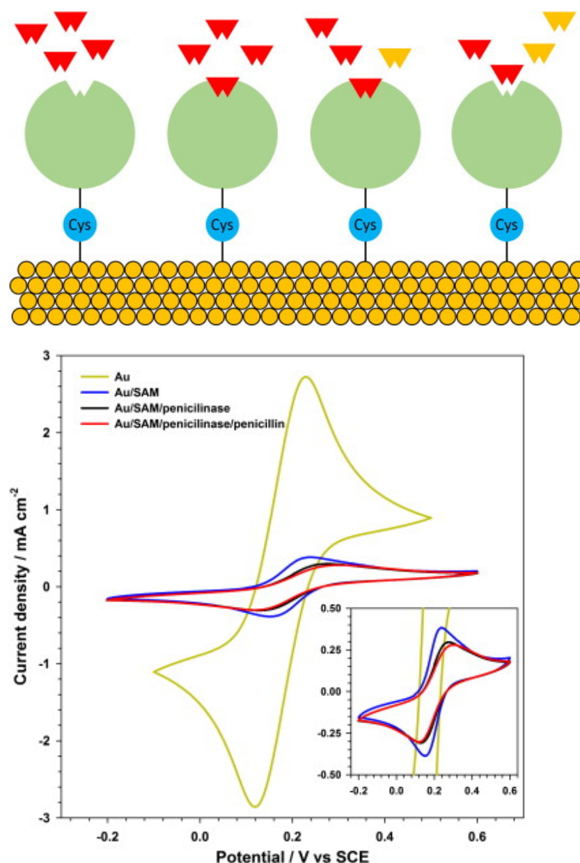
Figure 18. (Top) Schematic diagram of the experimental configuration: \beta -lactamases are connected to the gold electrode surface by cysteine molecules. Penicillin G molecules in solution react with the \beta -lactamases. (Bottom) Cyclic voltammetry of a ferrocene solution, 2 \text{ mmol L}^{-1} , in \text{KNO}_3 , 1 \text{ mol L}^{-1} , with different electrode surfaces: bare gold; gold and cysteine SAM; gold, cysteine SAM with penicillinase; and gold, cysteine SAM with penicillinase and the analyte penicillin (inset: detail of lower currents) [155]. Reprinted from Ref. [155], Copyright (2014), with permission from Elsevier.
