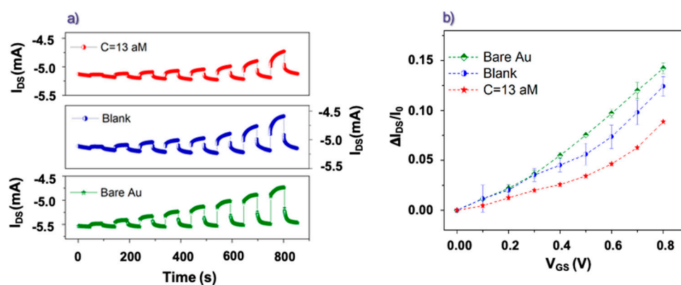
Figure 2. (a) I_{DS} vs. time (pulse) curves recorded in PBS using a pristine gate electrode (Bare Au), a gate electrode functionalized with anti-TG2 antibodies before any incubation step (Blank) and after the incubation in solution with attomolar concentration of rhTG2 protein ( C = 13 aM) (b) Corresponding average values of the I_{DS} modulation extracted as a function of V_{GS} . Error bars represent the standard deviations.
