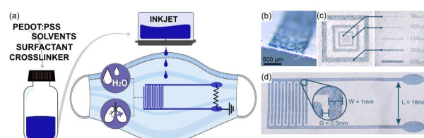
Figure 1. E-mask fabrication process. (a) Schematics of the e-mask fabrication route composed of the printable PEDOT:PSS ink formulation (on the left), the sensor direct printing onto the medical facemask (on the right), and the possibility of dual monitoring with IDEs. (b) Picture of a printed IDEs finger, a cross-section view. (c) Optical images of the square resolution pattern printed on the facemask filter fabric with a zoomed view of the printed lines with different width. (d) Picture of the printed IDEs sensor with the specific dimensions: the length between the electrodes (L), the width of the electrodes' fingers (W), and the gap between fingers (G).
