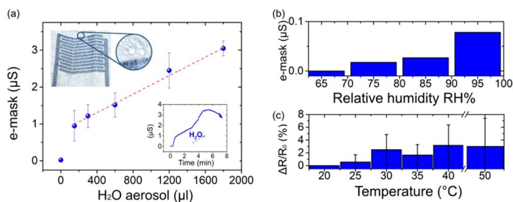
Figure 2. E-mask characterization. (a) E-mask calibration curve with respect to \text{H}_2\text{O} aerosol flow. Error bars represent the standard error over three measurements; the dotted red line is the linear fit. Top-left inset shows the damp sensor with the zoom on the condensed water droplets formation. Bottom-right inset shows the e-mask time response to aerosol flow (rate of 300 \mu\text{L}/\text{min} ). (b) E-mask signal output ( \mu\text{S} ) variation with respect to the relative humidity (RH varies from 65% to 95%). (c) Electrical resistance variation (%) of printed PEDOT:PSS lines with respect to the temperature increase (from 20^\circ\text{C} to 50^\circ\text{C} ).
