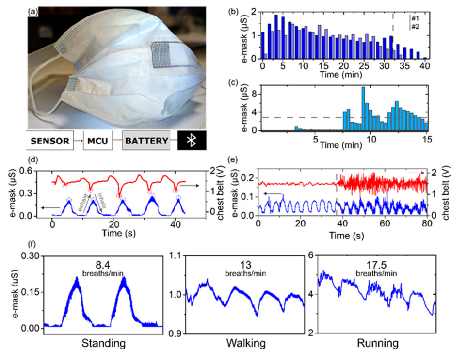
Figure 3. E-mask system response: (a) Picture of the final e-mask with printed IDEs (dark lines). On the bottom, a schematic presentation of the portable acquisition system for the data collection, the digitalization, and the wireless signal transfer. (b) E-mask time response of the wetting process monitoring during a walking activity (data from 2 different masks). The dashed line indicates when the e-mask is removed and left to dry at ambient conditions. (c) E-mask time response of the wetting process monitoring during running activity. The dashed line reports the 3 \mu\text{S} threshold associated with the facemask damp condition. (d) Time window of the respiration rate monitoring: the e-mask (blue) and chest belt (red). Small circles indicate respiration cycles. (e) Raw signals of the e-mask (blue) and chest belt (red). The vertical dashed line indicates the passage from resting to running. (f) Estimation of the respiration rate from the e-mask raw signal at standing, walking, and running activities. RR estimation is given over a time window of 20 s and sensor's response below and over the dampness threshold, demonstrating a possibility for multimodal detection in running conditions.
