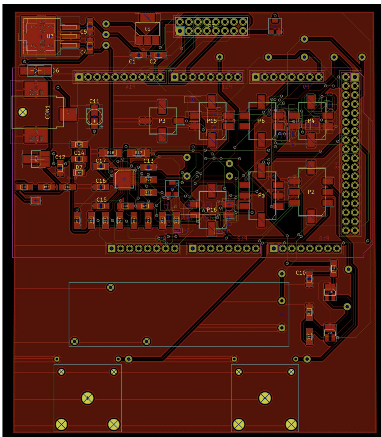
Figure S2. Main PCB layout.
