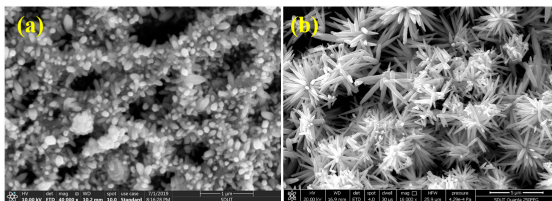
Figure S2. SEM images of as-prepared (a) ZnO HS1 sample and (b) ZnO HS2 sample after application in the gas sensing.
