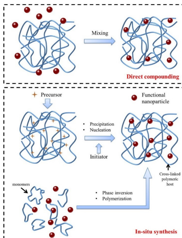
Scheme 4. Illustration of synthesis methods for polymeric nano-composites. Reproduced with permission from [109]. Copyright Elsevier, 2016.
