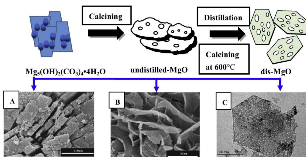
Scheme 3. Schematic illustration for the formation of mesoporous MgO nanosheets. Reproduced with permission from [205]. Copyright Elsevier, 2015.
